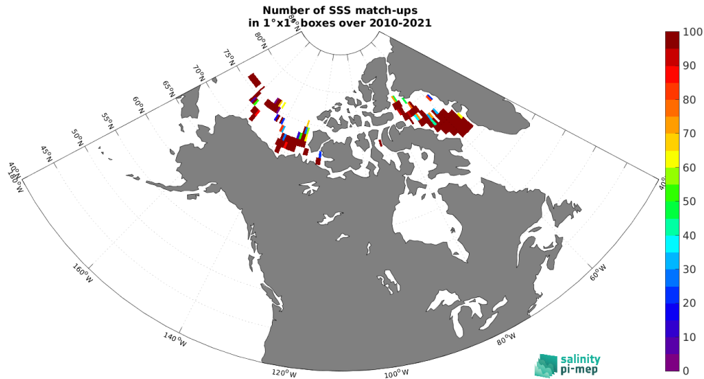
Figure 4: Number of SSS match-ups between TSG (Amundsen) SSS and the SMOS SSS L2Q v331 - With FLAG (CMEMS-CATDS-CPDC) SSS product for the Arctic Ocean Pi-MEP region over 1^\circ \times 1^\circ boxes and for the full satellite product period.
