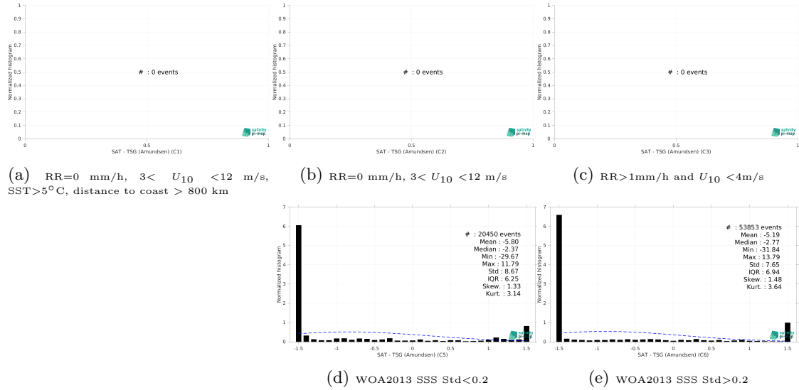
Figure 13: Normalized histogram of \Delta SSS (SMOS SSS L2Q v331 - With FLAG (CMEMS-CATDS-CPDC) - TSG (Amundsen)) for 5 different subdatasets corresponding to: RR=0 mm/h, 3 < U_{10} < 12 m/s, SST > 5°C, distance to coast > 800 km (a), RR=0 mm/h, 3 < U_{10} < 12 m/s (b), RR > 1mm/h and U_{10} < 4 m/s (c), WOA2013 SSS Std < 0.2 (d), WOA2013 SSS Std > 0.2 (e).
