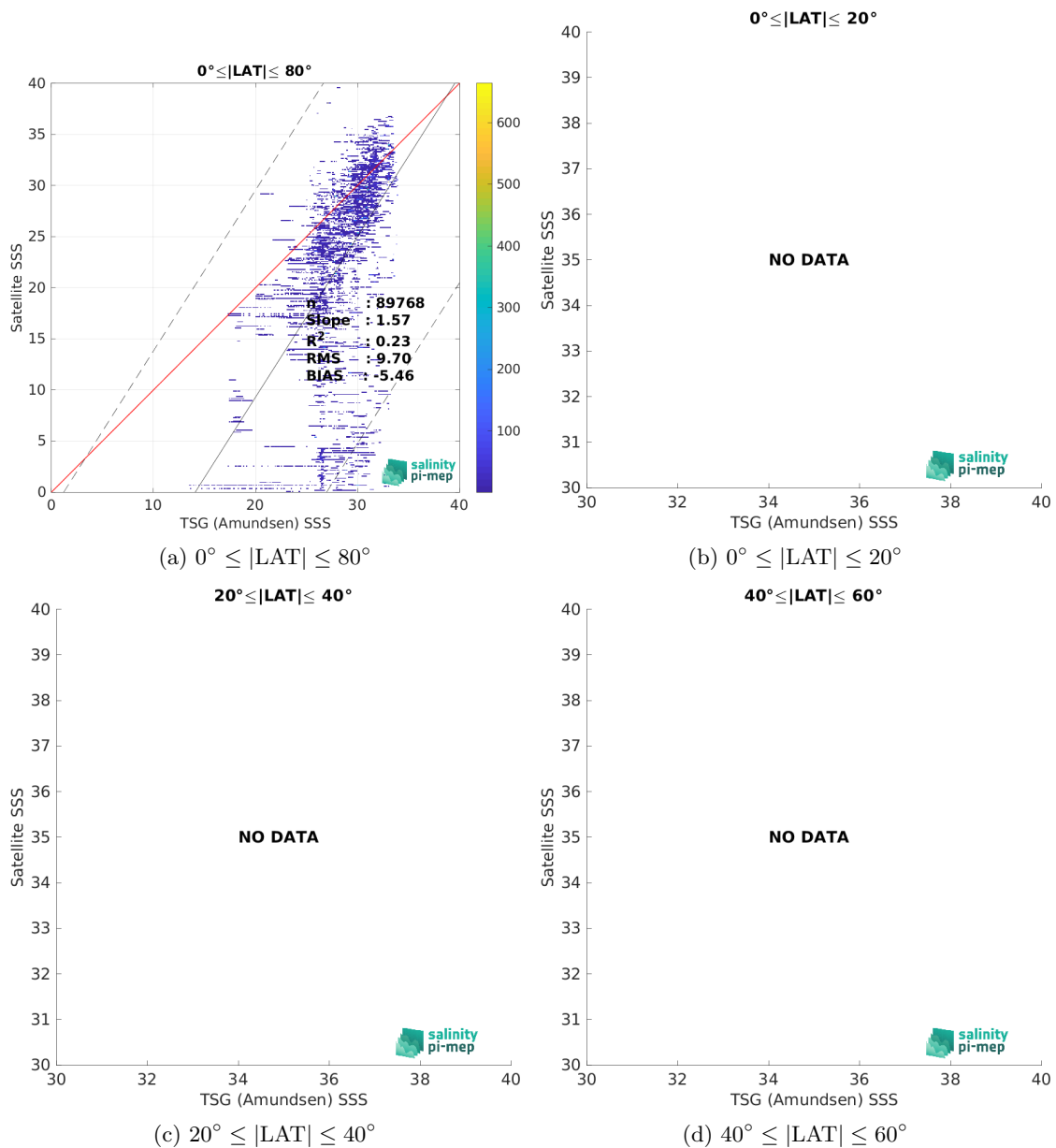
Figure 9: Contour maps of the concentration of SMOS SSS L2Q v331 - With FLAG (CMEMS-CATDS-CPDC) SSS (y-axis) versus TSG (Amundsen) SSS (x-axis) at match-up pairs for different latitude bands. For each plot, the red line shows x=y . The black thin and dashed lines indicate a linear fit through the data cloud and the \pm 95\% confidence levels, respectively. The number match-up pairs n , the slope and R^2 coefficient of the linear fit, the root mean square (RMS) and the mean bias between satellite and in situ data are indicated for each latitude band in each plots.
