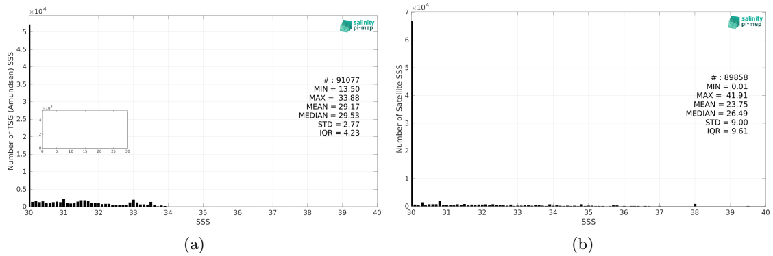
Figure 2: Histograms of SSS from TSG (Amundsen) (a) and SMOS SSS L2Q v331 - With FLAG (CMEMS-CATDS-CPDC) (b) considering all match-up pairs per bins of 0.1 over the Arctic Ocean Pi-MEP region and for the full satellite product period.
