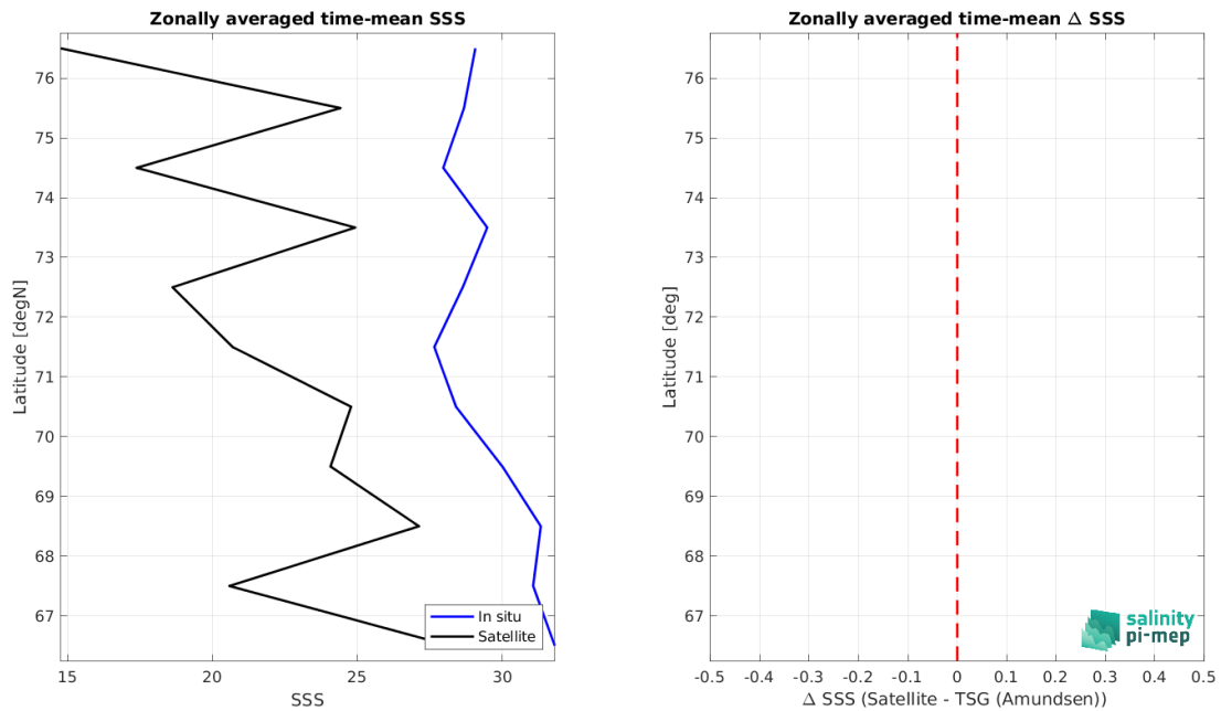
Figure 8: Left panel: Zonal mean SSS from SMOS SSS L2Q v331 - With FLAG (CMEMS-CATDS-CPDC) satellite product (black) and from TSG (Amundsen) (blue). Right panel: Zonal mean of \Delta SSS (Satellite - TSG (Amundsen)) for all the collected Pi-MEP match-up pairs estimated over the full satellite product period.
