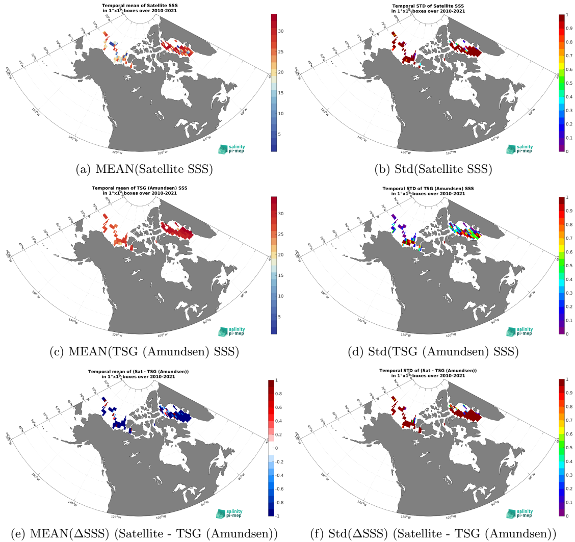
Figure 6: Temporal mean (left) and Std (right) of SSS from SMOS SSS L2Q v331 - With FLAG (CMEMS-CATDS-CPDC) (top), TSG (Amundsen) (middle), and of \Delta SSS (Satellite - TSG (Amundsen)). Only match-up pairs are used to generate these maps.
