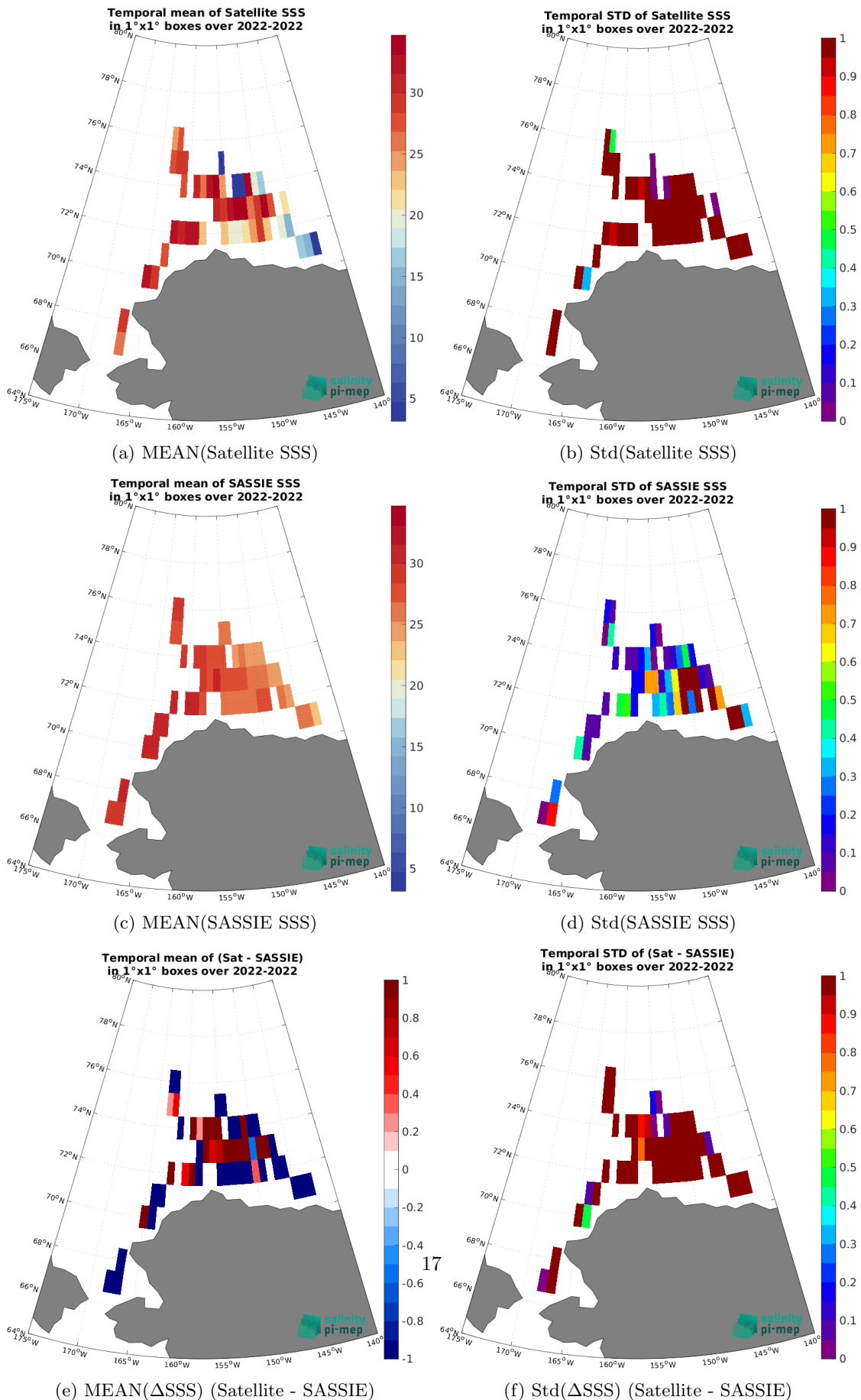
Figure 7: Temporal mean (left) and Std (right) of SSS from SMOS SSS L2Q v331 - With FLAG (CMEMS-CATDS-CPDC) (top), SASSIE (middle), and of \Delta SSS (Satellite - SASSIE). Only match-up pairs are used to generate these maps.
