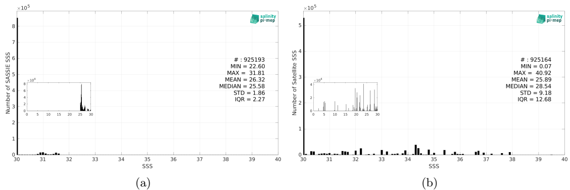
Figure 3: Histograms of SSS from SASSIE (a) and SMOS SSS L2Q v331 - With FLAG (CMEMS-CATDS-CPDC) (b) considering all match-up pairs per bins of 0.1 over the Arctic Ocean Pi-MEP region and for the full satellite product period.
