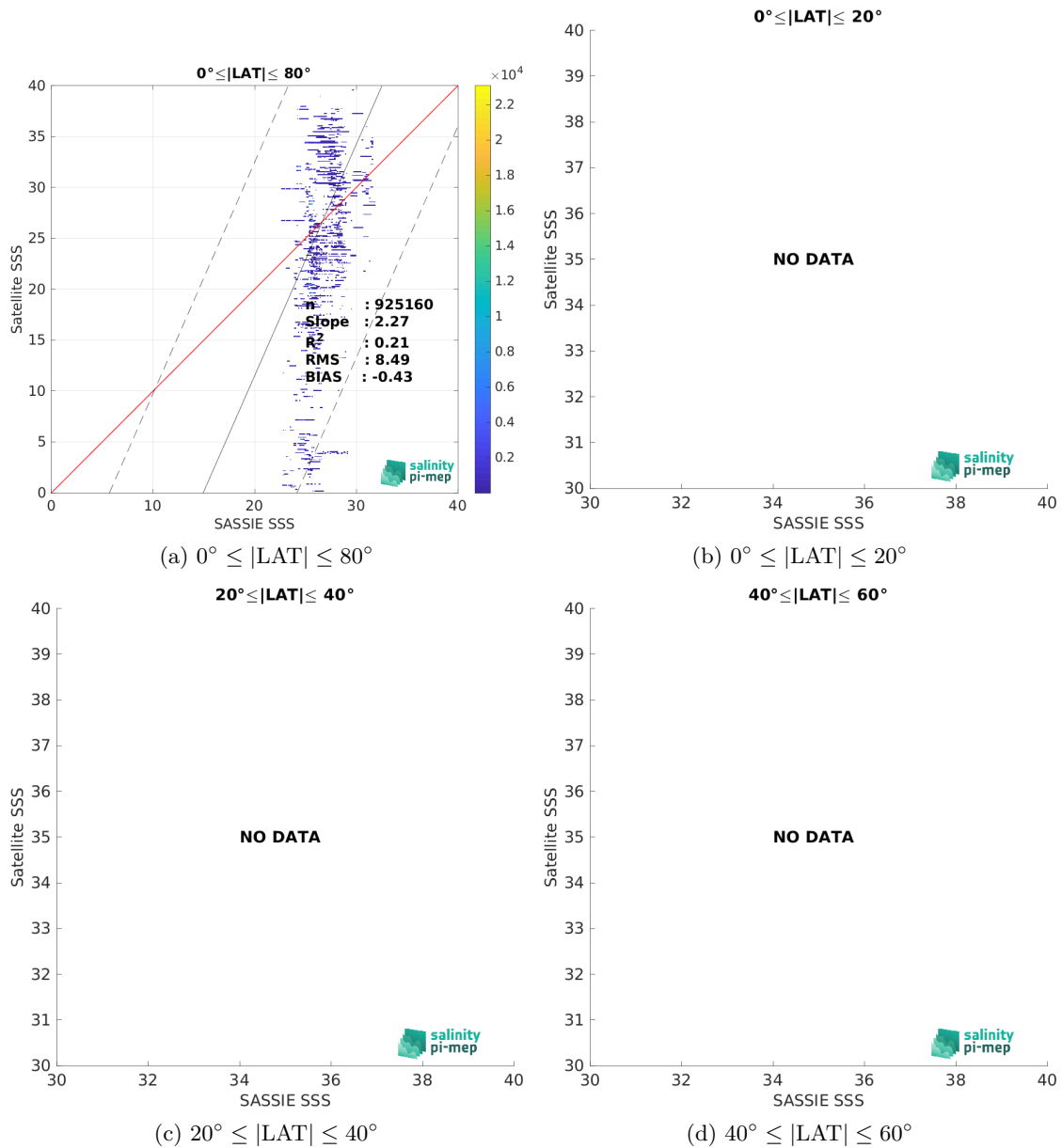
Figure 10: Contour maps of the concentration of SMOS SSS L2Q v331 - With FLAG (CMEMS-CATDS-CPDC) SSS (y-axis) versus SASSIE SSS (x-axis) at match-up pairs for different latitude bands. For each plot, the red line shows x=y . The black thin and dashed lines indicate a linear fit through the data cloud and the \pm 95\% confidence levels, respectively. The number match-up pairs n , the slope and R^2 coefficient of the linear fit, the root mean square (RMS) and the mean bias between satellite and in situ data are indicated for each latitude band in each plots.
