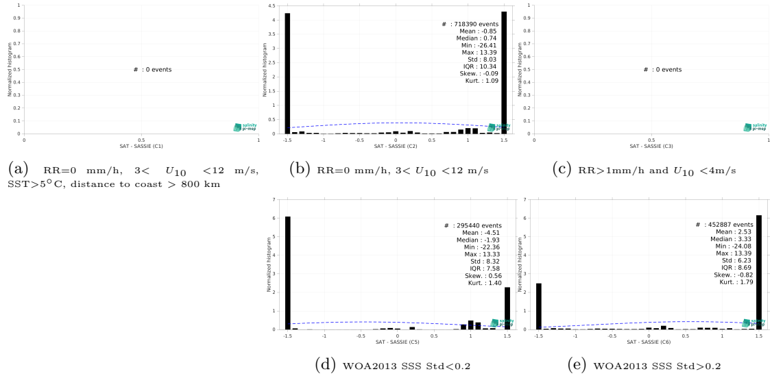
Figure 15: Normalized histogram of \Delta SSS (SMOS SSS L2Q v331 - With FLAG (CMEMS-CATDS-CPDC) - SASSIE) for 5 different subdatasets corresponding to: RR=0 mm/h, 3 < U_{10} < 12 m/s, SST > 5°C, distance to coast > 800 km (a), RR=0 mm/h, 3 < U_{10} < 12 m/s (b), RR > 1mm/h and U_{10} < 4 m/s (c), WOA2013 SSS Std < 0.2 (d), WOA2013 SSS Std > 0.2 (e).
