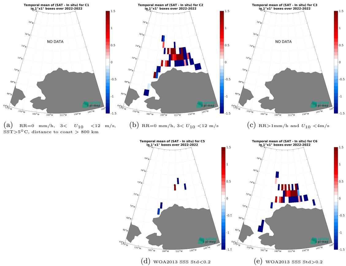
Figure 14: Temporal mean gridded over spatial boxes of size 1^\circ \times 1^\circ of \Delta SSS (SMOS SSS L2Q v331 - With FLAG (CMEMS-CATDS-CPDC) - SASSIE) for 5 different subdatasets corresponding to:RR=0 mm/h, 3 < U_{10} < 12 m/s, SST >5^\circ\text{C} , distance to coast > 800 km (a), RR=0 mm/h, 3 < U_{10} < 12 m/s (b), RR >1 mm/h and U_{10} < 4 m/s (c), WOA2013 SSS Std <0.2 (d), WOA2013 SSS Std >0.2 (e).
