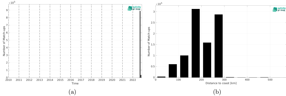
Figure 2: Number of match-ups between SASSIE and SMOS SSS L2Q v331 - With FLAG (CMEMS-CATDS-CPDC) SSS as a function of time (a) and as function of the distance to coast (b) over the Arctic Ocean Pi-MEP region and for the full satellite product period.
