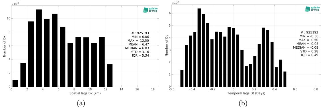
Figure 6: Histograms of the spatial (a) and temporal (b) lags between the location/time of the SASSIE measurement and the date of the corresponding SMOS SSS L2Q v331 - With FLAG (CMEMS-CATDS-CPDC) SSS pixel.
