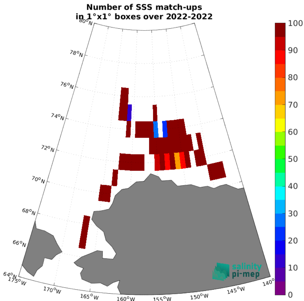
Figure 5: Number of SSS match-ups between SASSIE SSS and the SMOS SSS L2Q v331 - With FLAG (CMEMS-CATDS-CPDC) SSS product for the Arctic Ocean Pi-MEP region over 1^\circ \times 1^\circ boxes and for the full satellite product period.
