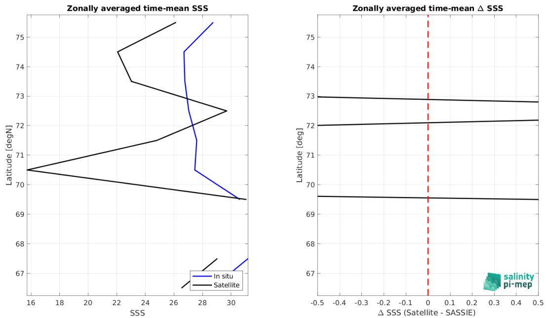
Figure 9: Left panel: Zonal mean SSS from SMOS SSS L2Q v331 - With FLAG (CMEMS-CATDS-CPDC) satellite product (black) and from SASSIE (blue). Right panel: Zonal mean of \Delta SSS (Satellite - SASSIE) for all the collected Pi-MEP match-up pairs estimated over the full satellite product period.
