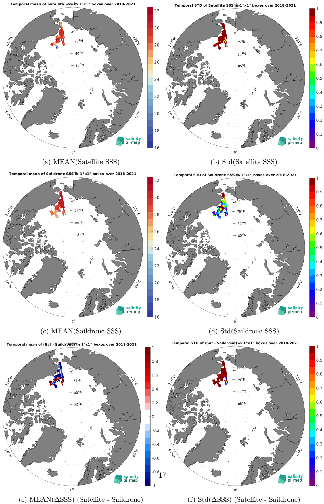
Figure 7: Temporal mean (left) and Std (right) of SSS from SMOS SSS L2Q v331 - With FLAG (CMEMS-CATDS-CPDC) (top), Saildrone (middle), and of \Delta SSS (Satellite - Saildrone). Only match-up pairs are used to generate these maps.
