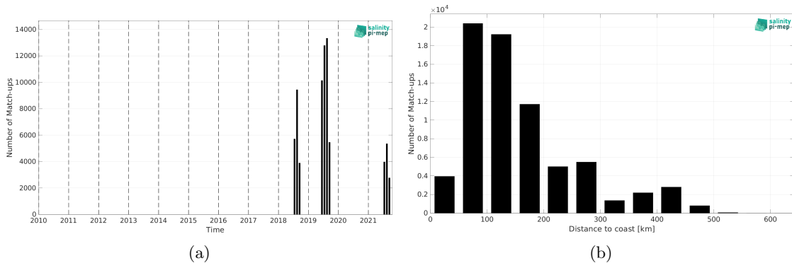
Figure 2: Number of match-ups between Saildrone and SMOS SSS L2Q v331 - With FLAG (CMEMS-CATDS-CPDC) SSS as a function of time (a) and as function of the distance to coast (b) over the Arctic Ocean Pi-MEP region and for the full satellite product period.
