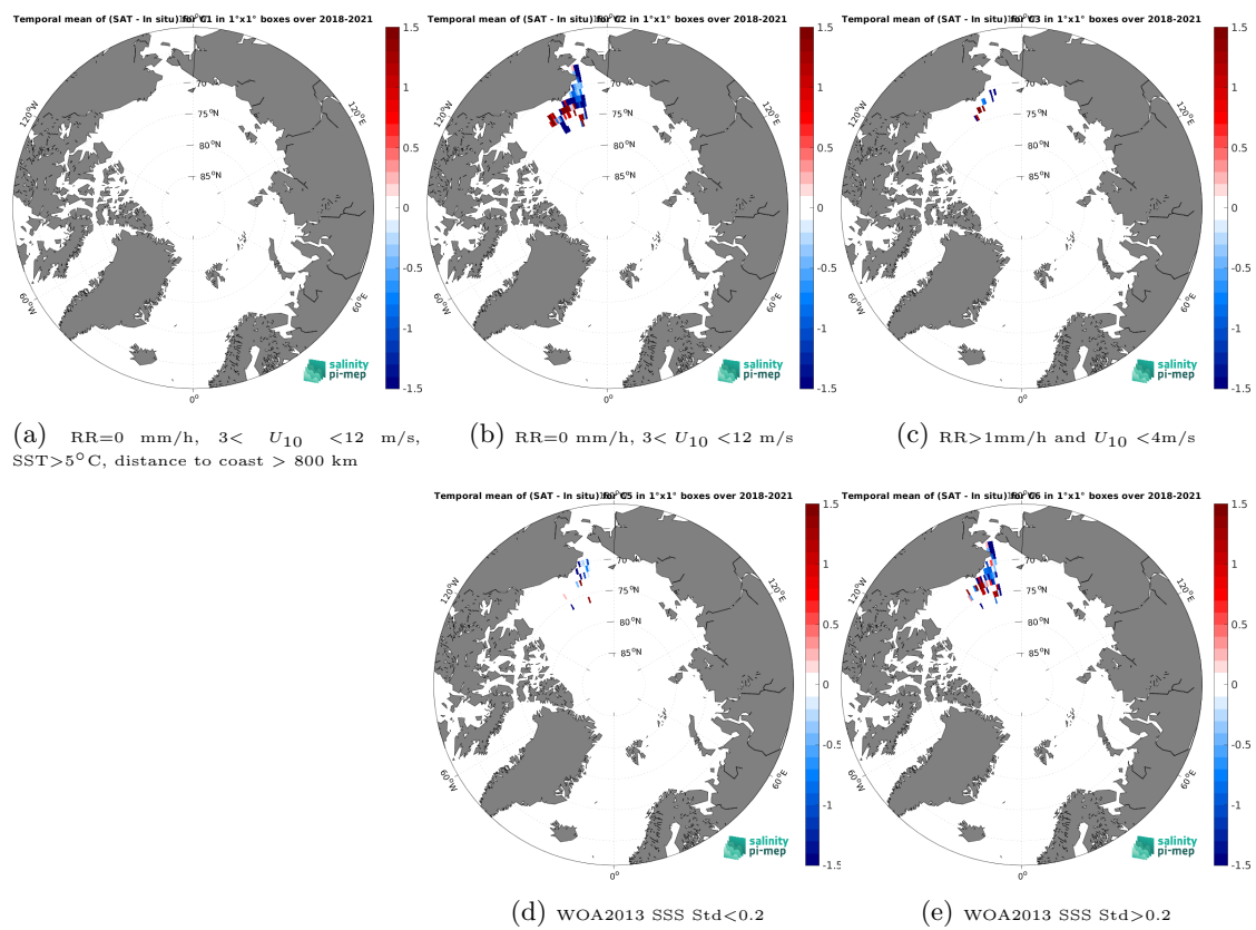
Figure 14: Temporal mean gridded over spatial boxes of size 1^\circ \times 1^\circ of \Delta SSS (SMOS SSS L2Q v331 - With FLAG (CMEMS-CATDS-CPDC) - Saildrone) for 5 different subdatasets corresponding to:RR=0 mm/h, 3 < U_{10} < 12 m/s, SST > 5°C, distance to coast > 800 km (a), RR=0 mm/h, 3 < U_{10} < 12 m/s (b), RR > 1mm/h and U_{10} < 4 m/s (c), WOA2013 SSS Std < 0.2 (d), WOA2013 SSS Std > 0.2 (e).
