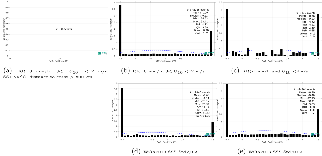
Figure 15: Normalized histogram of \Delta SSS (SMOS SSS L2Q v331 - With FLAG (CMEMS-CATDS-CPDC) - Saildrone) for 5 different subdatasets corresponding to: RR=0 mm/h, 3 < U_{10} < 12 m/s, SST > 5°C, distance to coast > 800 km (a), RR=0 mm/h, 3 < U_{10} < 12 m/s (b), RR > 1mm/h and U_{10} < 4 m/s (c), WOA2013 SSS Std < 0.2 (d), WOA2013 SSS Std > 0.2 (e).
