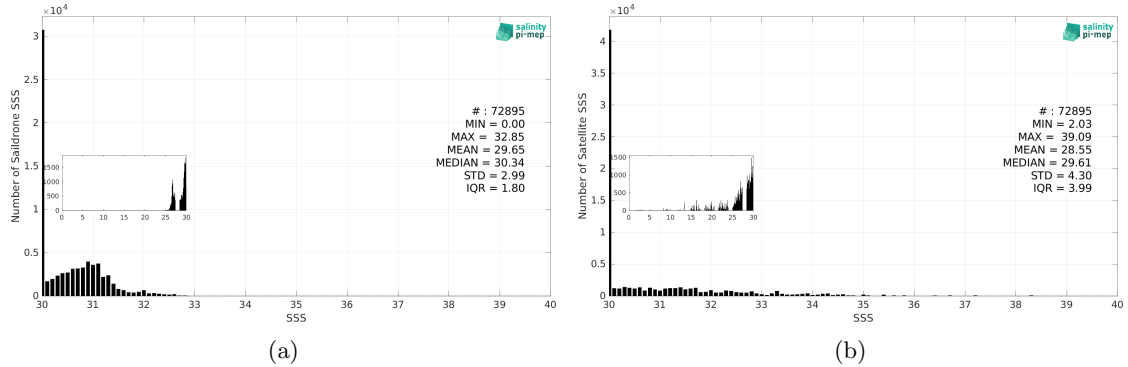
Figure 3: Histograms of SSS from Saildrone (a) and SMOS SSS L2Q v331 - With FLAG (CMEMS-CATDS-CPDC) (b) considering all match-up pairs per bins of 0.1 over the Arctic Ocean Pi-MEP region and for the full satellite product period.
