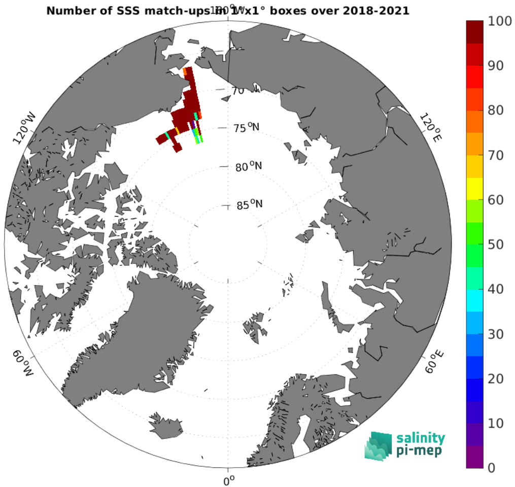
Figure 5: Number of SSS match-ups between Saildrone SSS and the SMOS SSS L2Q v331 - With FLAG (CMEMS-CATDS-CPDC) SSS product for the Arctic Ocean Pi-MEP region over 1^\circ \times 1^\circ boxes and for the full satellite product period.
