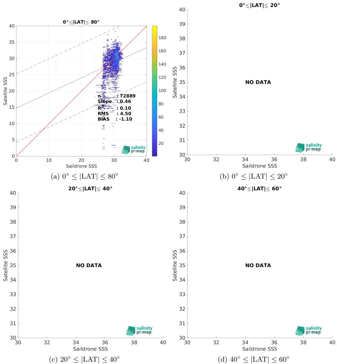
Figure 10: Contour maps of the concentration of SMOS SSS L2Q v331 - With FLAG (CMEMS-CATDS-CPDC) SSS (y-axis) versus Saildrone SSS (x-axis) at match-up pairs for different latitude bands. For each plot, the red line shows x=y . The black thin and dashed lines indicate a linear fit through the data cloud and the \pm 95\% confidence levels, respectively. The number match-up pairs n , the slope and R^2 coefficient of the linear fit, the root mean square (RMS) and the mean bias between satellite and in situ data are indicated for each latitude band in each plots.
