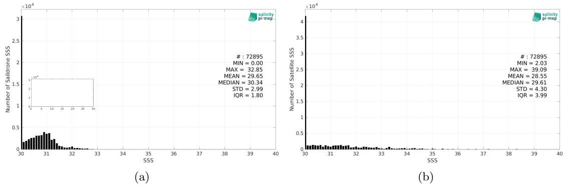
Figure 2: Histograms of SSS from Saildrone (a) and SMOS SSS L2Q v331 - With FLAG (CMEMS-CATDS-CPDC) (b) considering all match-up pairs per bins of 0.1 over the Arctic Ocean Pi-MEP region and for the full satellite product period.
