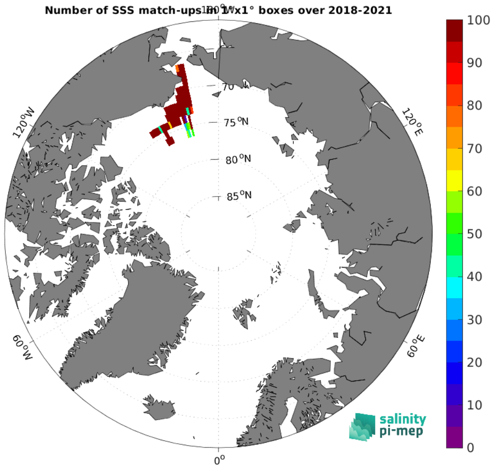
Figure 4: Number of SSS match-ups between Saildrone SSS and the SMOS SSS L2Q v331 - With FLAG (CMEMS-CATDS-CPDC) SSS product for the Arctic Ocean Pi-MEP region over 1^\circ \times 1^\circ boxes and for the full satellite product period.
