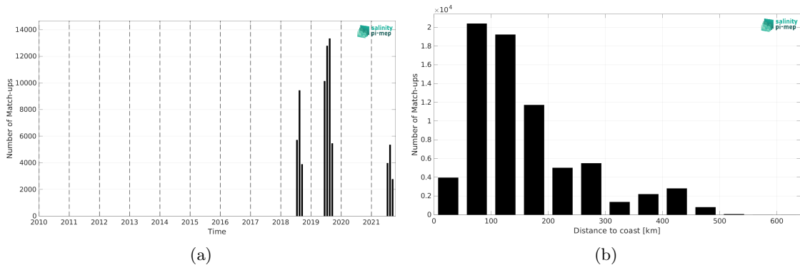
Figure 1: Number of match-ups between Saildrone and SMOS SSS L2Q v331 - With FLAG (CMEMS-CATDS-CPDC) SSS as a function of time (a) and as function of the distance to coast (b) over the Arctic Ocean Pi-MEP region and for the full satellite product period.
