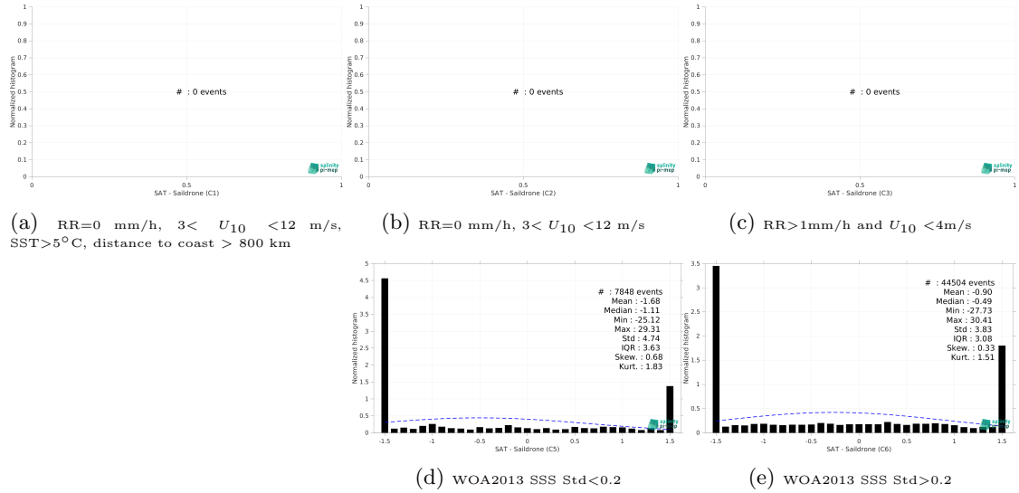
Figure 13: Normalized histogram of \Delta SSS (SMOS SSS L2Q v331 - With FLAG (CMEMS-CATDS-CPDC) - Salldrone) for 5 different subdatasets corresponding to: RR=0 mm/h, 3 < U_{10} < 12 m/s, SST > 5°C, distance to coast > 800 km (a), RR=0 mm/h, 3 < U_{10} < 12 m/s (b), RR > 1mm/h and U_{10} < 4 m/s (c), WOA2013 SSS Std < 0.2 (d), WOA2013 SSS Std > 0.2 (e).
