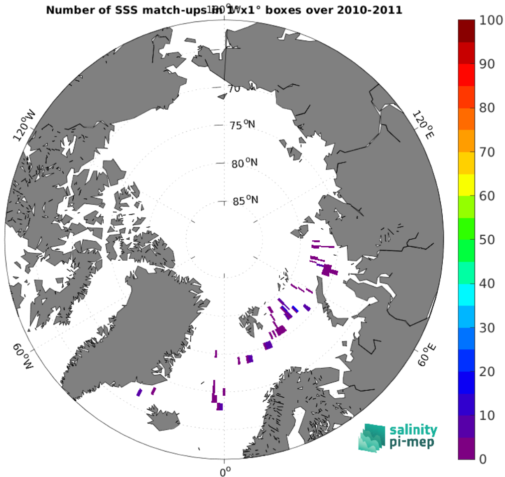
Figure 5: Number of SSS match-ups between Marine mammals SSS and the SMOS SSS L2Q v331 - With FLAG (CMEMS-CATDS-CPDC) SSS product for the Arctic Ocean Pi-MEP region over 1^\circ \times 1^\circ boxes and for the full satellite product period.
