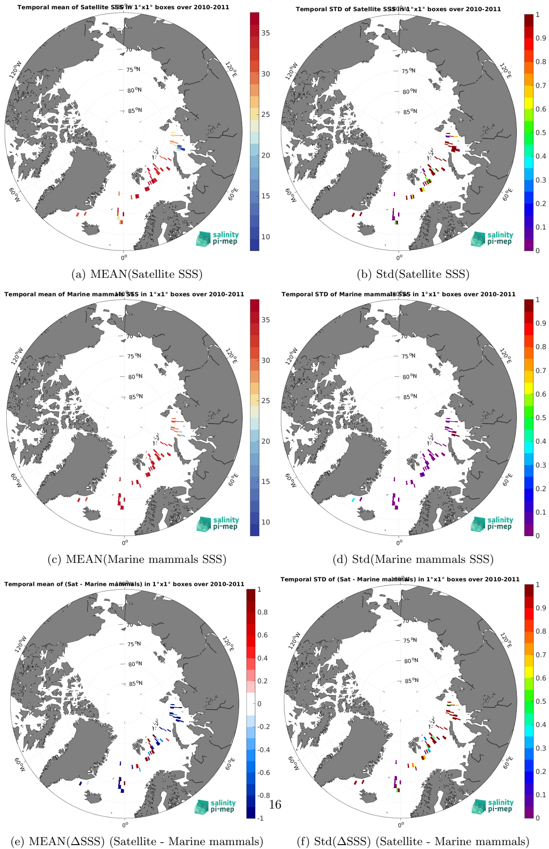
Figure 7: Temporal mean (left) and Std (right) of SSS from SMOS SSS L2Q v331 - With FLAG (CMEMS-CATDS-CPDC) (top), Marine mammals (middle), and of \Delta SSS (Satellite - Marine mammals). Only match-up pairs are used to generate these maps.
