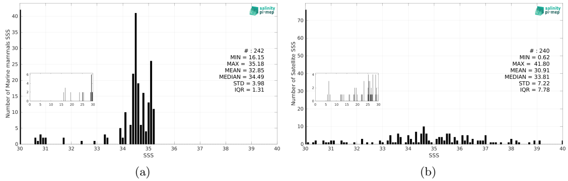
Figure 3: Histograms of SSS from Marine mammals (a) and SMOS SSS L2Q v331 - With FLAG (CMEMS-CATDS-CPDC) (b) considering all match-up pairs per bins of 0.1 over the Arctic Ocean Pi-MEP region and for the full satellite product period.
