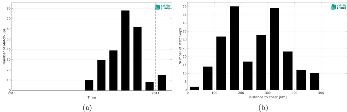
Figure 2: Number of match-ups between Marine mammals and SMOS SSS L2Q v331 - With FLAG (CMEMS-CATDS-CPDC) SSS as a function of time (a) and as function of the distance to coast (b) over the Arctic Ocean Pi-MEP region and for the full satellite product period.
