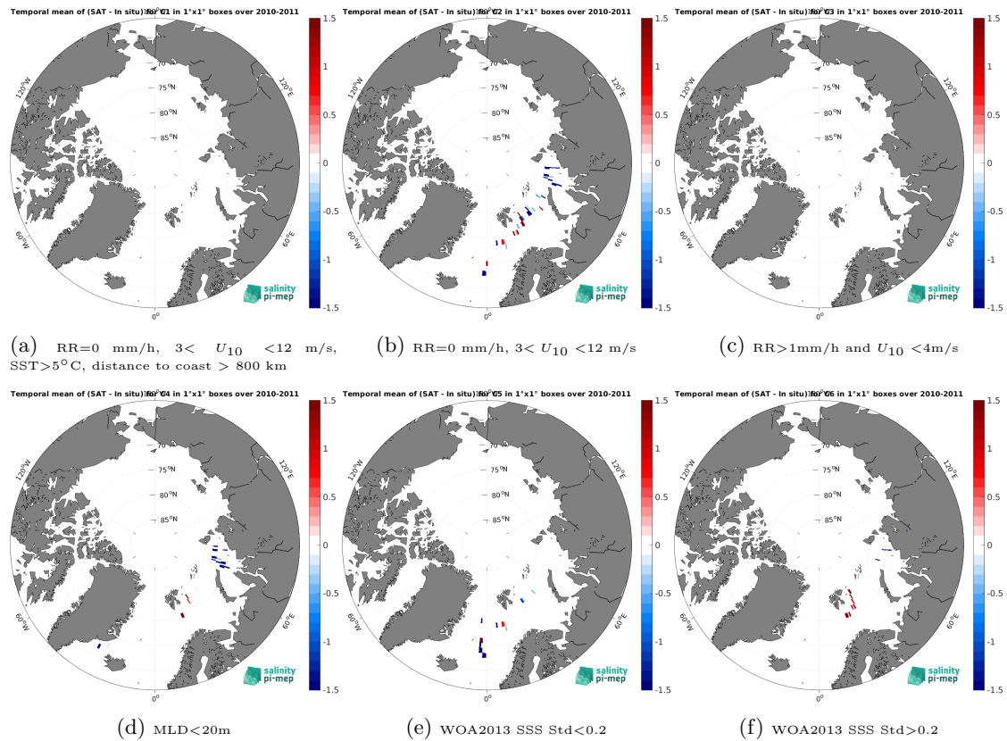
Figure 14: Temporal mean gridded over spatial boxes of size 1^\circ \times 1^\circ of \Delta SSS (SMOS SSS L2Q v331 - With FLAG (CMEMS-CATDS-CPDC) - Marine mammals) for 6 different subdatasets corresponding to:RR=0 mm/h, 3 < U_{10} < 12 m/s, SST>5°C, distance to coast > 800 km (a), RR=0 mm/h, 3 < U_{10} < 12 m/s (b), RR>1mm/h and U_{10} < 4 m/s (c),MLD<20m (d),WOA2013 SSS Std<0.2 (e),WOA2013 SSS Std>0.2 (f).
