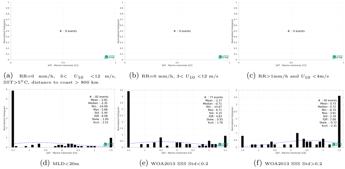
Figure 13: Normalized histogram of \Delta\text{SSS} (SMOS SSS L2Q v331 - With FLAG (CMEMS-CATDS-CPDC) - Marine mammals) for 6 different subdatasets corresponding to: RR=0 mm/h, 3 < U_{10} < 12 m/s, SST > 5^\circ\text{C} , distance to coast > 800 km (a), RR=0 mm/h, 3 < U_{10} < 12 m/s (b), RR > 1\text{mm/h} and U_{10} < 4\text{m/s} (c), MLD < 20\text{m} (d), WOA2013 SSS Std < 0.2 (e), WOA2013 SSS Std > 0.2 (f).
