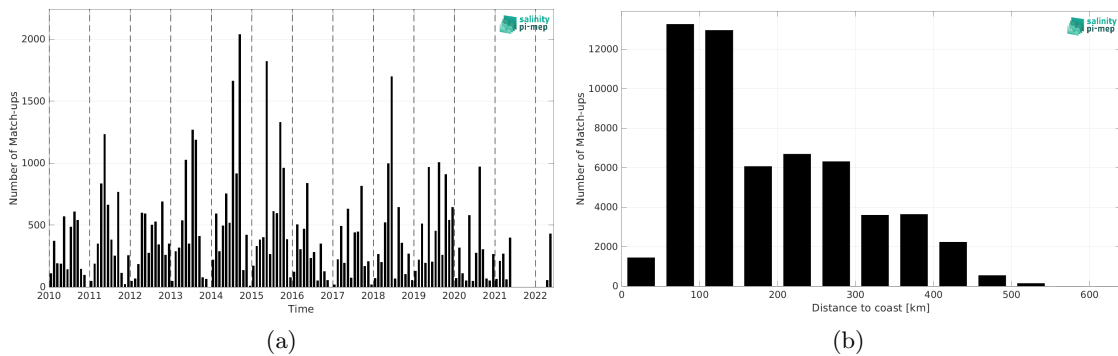
Figure 2: Number of match-ups between ICES and SMOS SSS L2Q v331 - With FLAG (CMEMS-CATDS-CPDC) SSS as a function of time (a) and as function of the distance to coast (b) over the Arctic Ocean Pi-MEP region and for the full satellite product period.
