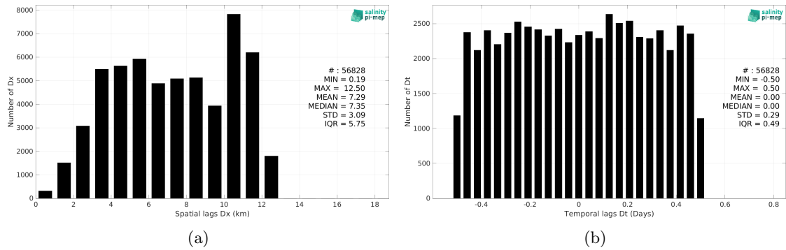
Figure 6: Histograms of the spatial (a) and temporal (b) lags between the location/time of the ICES measurement and the date of the corresponding SMOS SSS L2Q v331 - With FLAG (CMEMS-CATDS-CPDC) SSS pixel.
