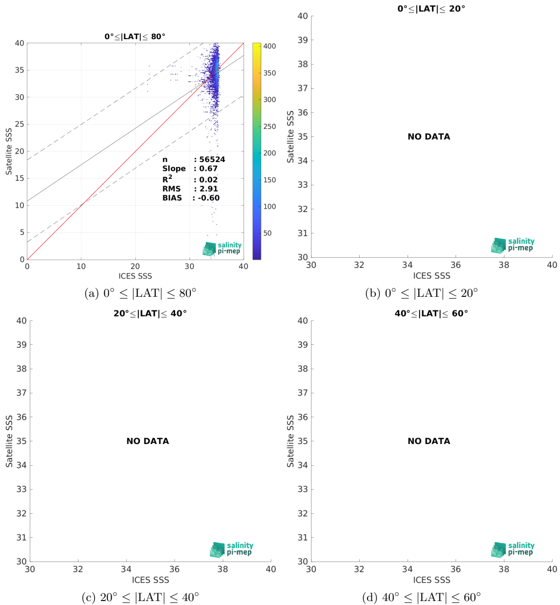
Figure 10: Contour maps of the concentration of SMOS SSS L2Q v331 - With FLAG (CMEMS-CATDS-CPDC) SSS (y-axis) versus ICES SSS (x-axis) at match-up pairs for different latitude bands. For each plot, the red line shows x=y . The black thin and dashed lines indicate a linear fit through the data cloud and the \pm 95\% confidence levels, respectively. The number match-up pairs n , the slope and R^2 coefficient of the linear fit, the root mean square (RMS) and the mean bias between satellite and in situ data are indicated for each latitude band in each plots.
