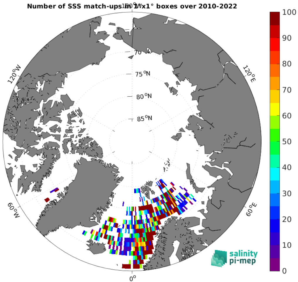
Figure 5: Number of SSS match-ups between ICES SSS and the SMOS SSS L2Q v331 - With FLAG (CMEMS-CATDS-CPDC) SSS product for the Arctic Ocean Pi-MEP region over 1^\circ \times 1^\circ boxes and for the full satellite product period.
