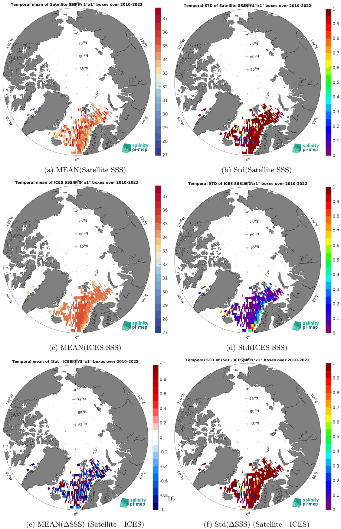
Figure 7: Temporal mean (left) and Std (right) of SSS from SMOS SSS L2Q v331 - With FLAG (CMEMS-CATDS-CPDC) (top), ICES (middle), and of \Delta SSS (Satellite - ICES). Only match-up pairs are used to generate these maps.
