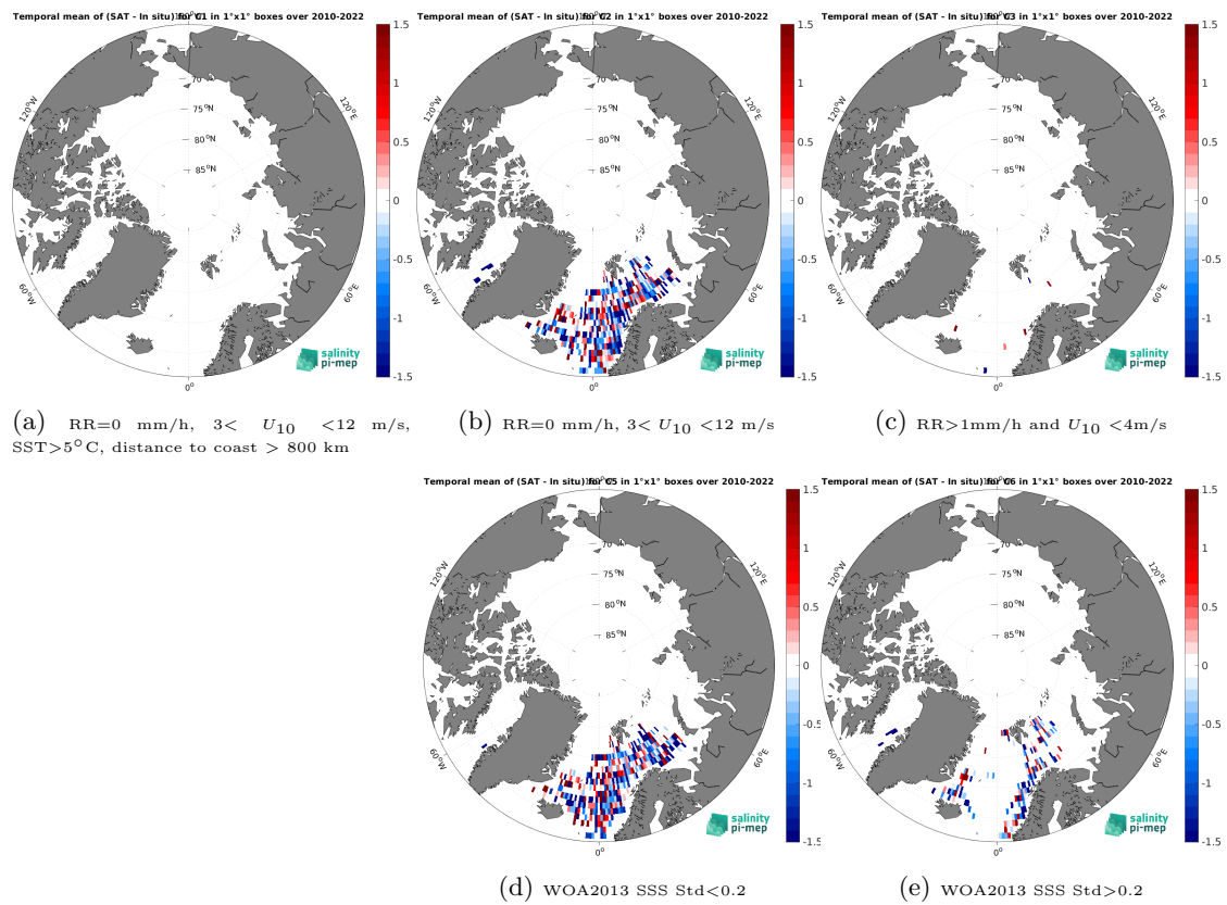
Figure 14: Temporal mean gridded over spatial boxes of size 1^\circ \times 1^\circ of \Delta SSS (SMOS SSS L2Q v331 - With FLAG (CMEMS-CATDS-CPDC) - ICES) for 5 different subdatasets corresponding to: RR=0 mm/h, 3 < U_{10} < 12 m/s, SST > 5^\circ\text{C} , distance to coast > 800 km (a), RR=0 mm/h, 3 < U_{10} < 12 m/s (b), RR > 1 mm/h and U_{10} < 4 m/s (c), WOA2013 SSS Std < 0.2 (d), WOA2013 SSS Std > 0.2 (e).
