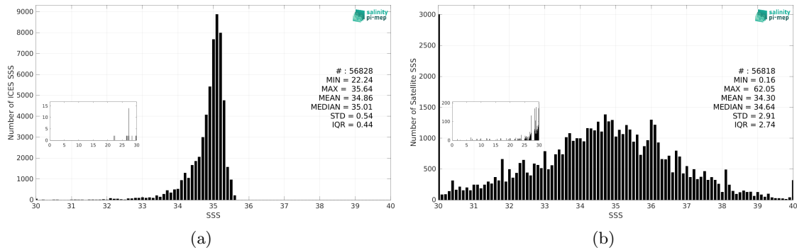
Figure 3: Histograms of SSS from ICES (a) and SMOS SSS L2Q v331 - With FLAG (CMEMS-CATDS-CPDC) (b) considering all match-up pairs per bins of 0.1 over the Arctic Ocean Pi-MEP region and for the full satellite product period.
