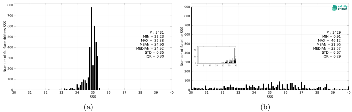
Figure 3: Histograms of SSS from Surface drifters (a) and SMOS SSS L2Q v331 - With FLAG (CMEMS-CATDS-CPDC) (b) considering all match-up pairs per bins of 0.1 over the Arctic Ocean Pi-MEP region and for the full satellite product period.
