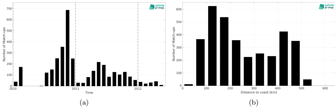
Figure 2: Number of match-ups between Surface drifters and SMOS SSS L2Q v331 - With FLAG (CMEMS-CATDS-CPDC) SSS as a function of time (a) and as function of the distance to coast (b) over the Arctic Ocean Pi-MEP region and for the full satellite product period.
