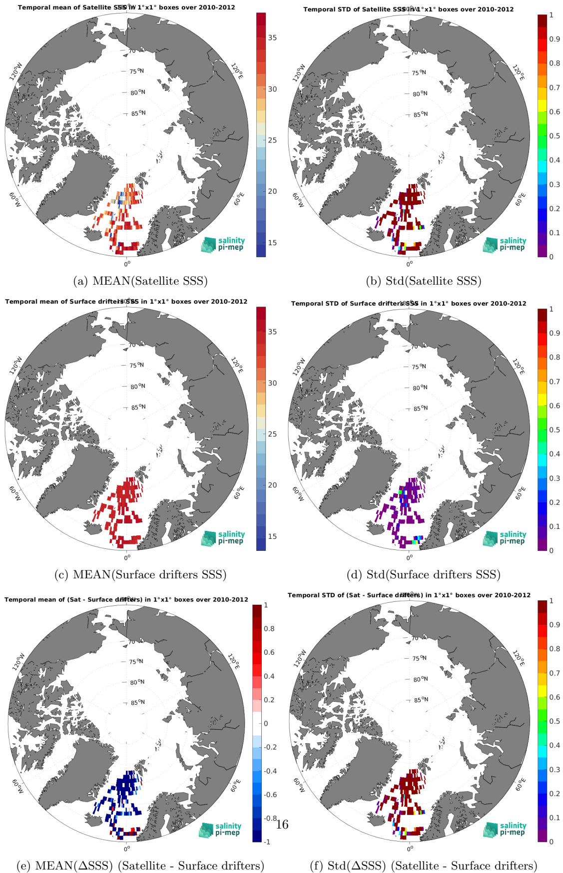
Figure 6: Temporal mean (left) and Std (right) of SSS from SMOS SSS L2Q v331 - With FLAG (CMEMS-CATDS-CPDC) (top), Surface drifters (middle), and of \Delta SSS (Satellite - Surface drifters). Only match-up pairs are used to generate these maps.
