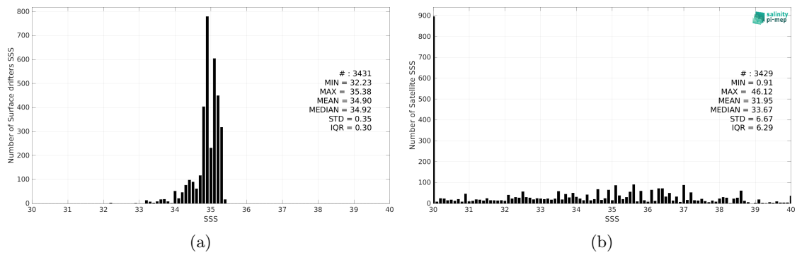
Figure 2: Histograms of SSS from Surface drifters (a) and SMOS SSS L2Q v331 - With FLAG (CMEMS-CATDS-CPDC) (b) considering all match-up pairs per bins of 0.1 over the Arctic Ocean Pi-MEP region and for the full satellite product period.
