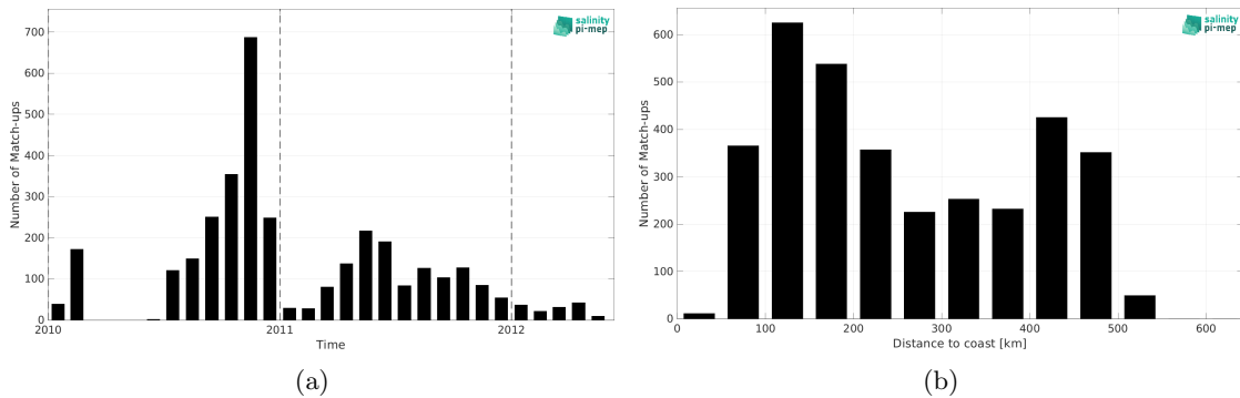
Figure 1: Number of match-ups between Surface drifters and SMOS SSS L2Q v331 - With FLAG (CMEMS-CATDS-CPDC) SSS as a function of time (a) and as function of the distance to coast (b) over the Arctic Ocean Pi-MEP region and for the full satellite product period.
