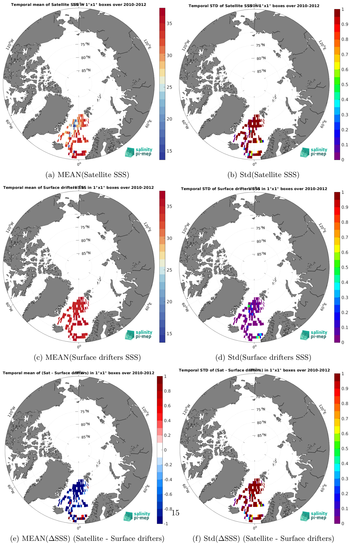
Figure 5: Temporal mean (left) and Std (right) of SSS from SMOS SSS L2Q v331 - With FLAG (CMEMS-CATDS-CPDC) (top), Surface drifters (middle), and of \Delta SSS (Satellite - Surface drifters). Only match-up pairs are used to generate these maps.
