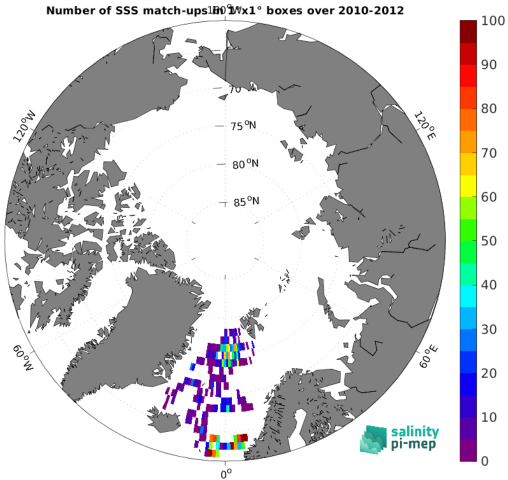
Figure 3: Number of SSS match-ups between Surface drifters SSS and the SMOS SSS L2Q v331 - With FLAG (CMEMS-CATDS-CPDC) SSS product for the Arctic Ocean Pi-MEP region over 1^{\circ} \times 1^{\circ} boxes and for the full satellite product period.
