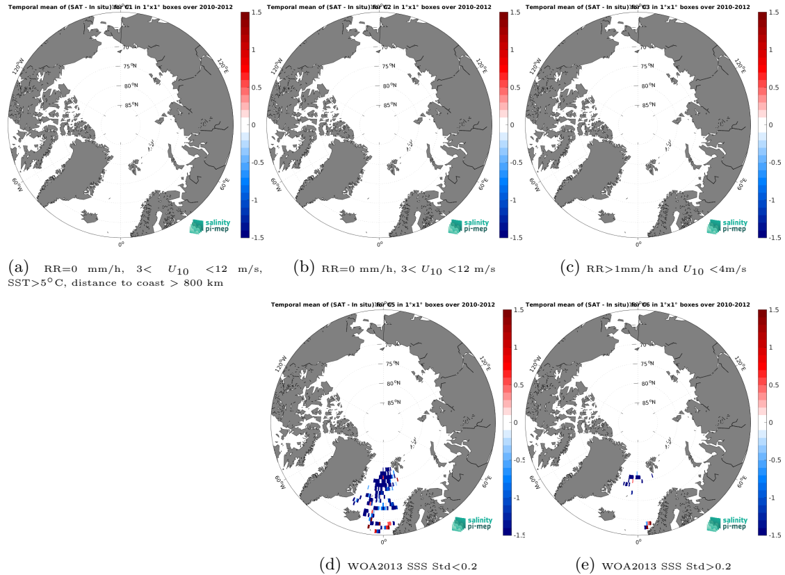
Figure 11: Temporal mean gridded over spatial boxes of size 1^{\circ}\times 1^{\circ} of \Delta\text{SSS} (SMOS SSS L2Q v331 - With FLAG (CMEMS-CATDS-CPDC) - Surface drifters) for 5 different subdatasets corresponding to:RR=0 mm/h, 3 < U_{10} < 12 m/s, SST > 5^{\circ}\text{C} , distance to coast > 800 km (a), RR=0 mm/h, 3 < U_{10} < 12 m/s (b), RR > 1 mm/h and U_{10} < 4 m/s (c), WOA2013 SSS Std < 0.2 (d), WOA2013 SSS Std > 0.2 (e).
