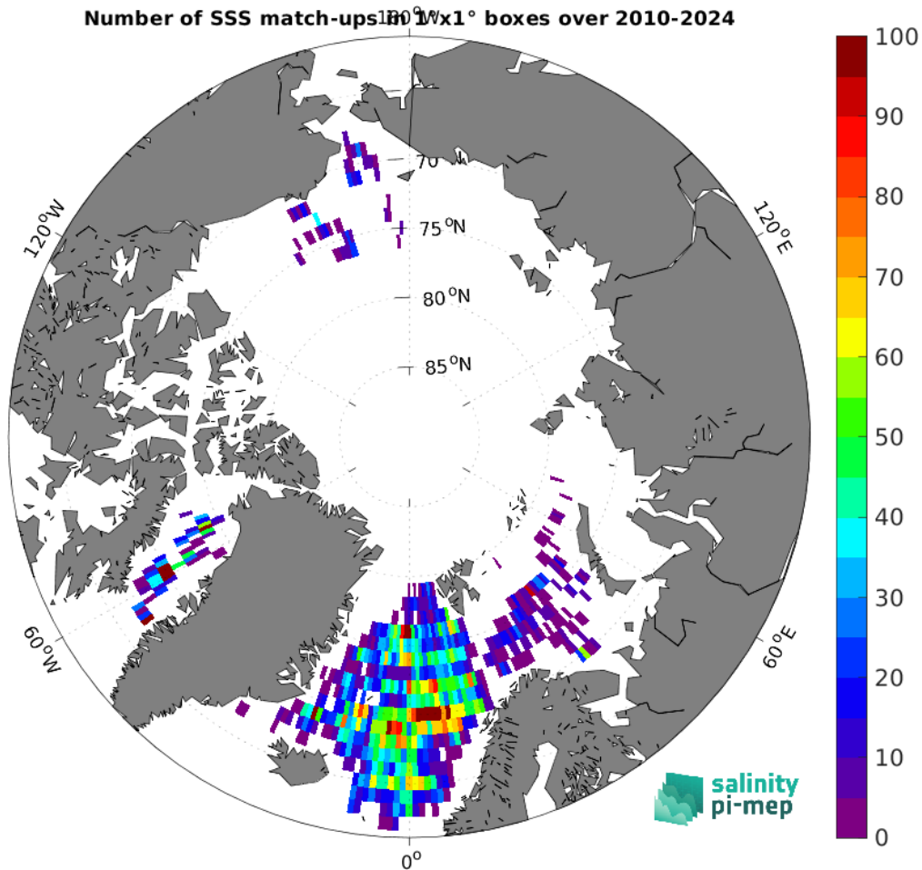
Figure 5: Number of SSS match-ups between Argo SSS and the SMOS SSS L2Q v331 - With FLAG (CMEMS-CATDS-CPDC) SSS product for the Arctic Ocean Pi-MEP region over 1^\circ \times 1^\circ boxes and for the full satellite product period.
