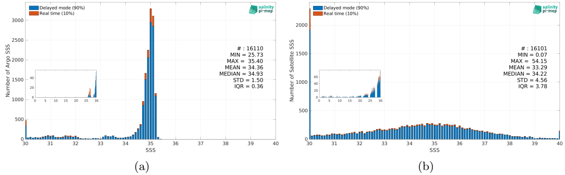
Figure 3: Histograms of SSS from Argo (a) and SMOS SSS L2Q v331 - With FLAG (CMEMS-CATDS-CPDC) (b) considering all match-up pairs per bins of 0.1 over the Arctic Ocean Pi-MEP region and for the full satellite product period.
