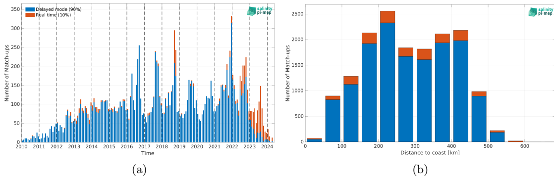
Figure 2: Number of match-ups between Argo and SMOS SSS L2Q v331 - With FLAG (CMEMS-CATDS-CPDC) SSS as a function of time (a) and as function of the distance to coast (b) over the Arctic Ocean Pi-MEP region and for the full satellite product period.
