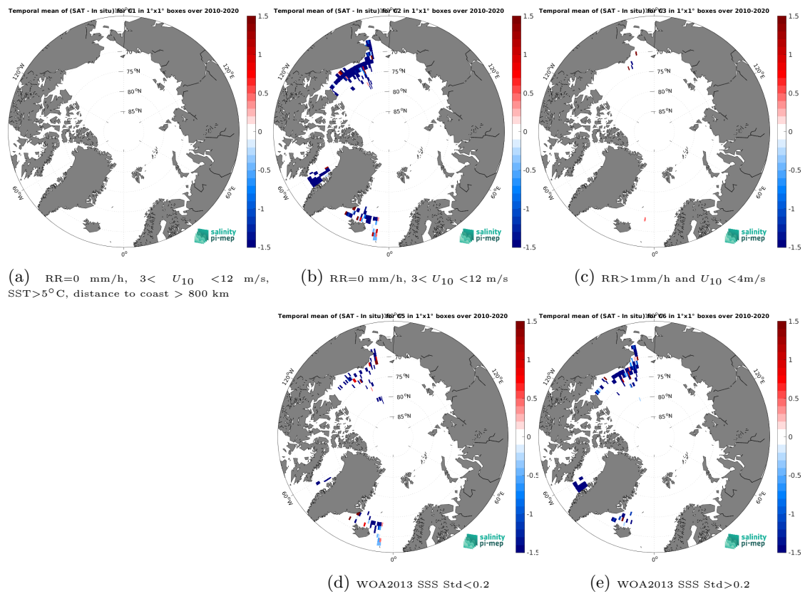
Figure 14: Temporal mean gridded over spatial boxes of size 1^\circ \times 1^\circ of \Delta SSS (SMOS SSS L2Q v331 - No FLAG (CMEMS-CATDS-CPDC) - TSG (SAMOS)) for 5 different subdatasets corresponding to:RR=0 mm/h, 3 < U_{10} < 12 m/s, SST > 5°C, distance to coast > 800 km (a), RR=0 mm/h, 3 < U_{10} < 12 m/s (b), RR > 1mm/h and U_{10} < 4 m/s (c), WOA2013 SSS Std < 0.2 (d), WOA2013 SSS Std > 0.2 (e).
