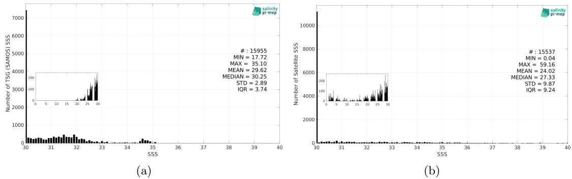
Figure 3: Histograms of SSS from TSG (SAMOS) (a) and SMOS SSS L2Q v331 - No FLAG (CMEMS-CATDS-CPDC) (b) considering all match-up pairs per bins of 0.1 over the Arctic Ocean Pi-MEP region and for the full satellite product period.
