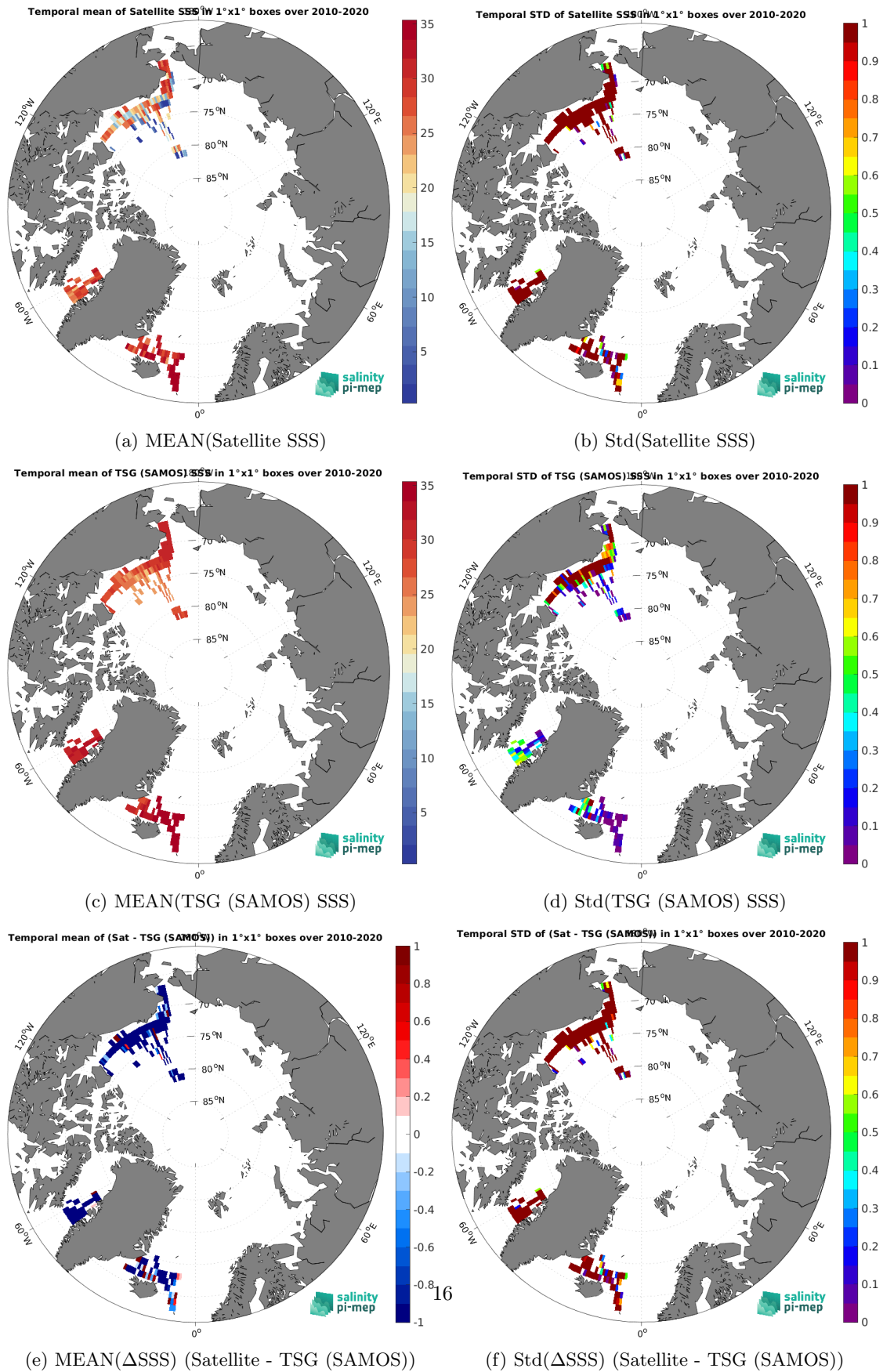
Figure 7: Temporal mean (left) and Std (right) of SSS from SMOS SSS L2Q v331 - No FLAG (CMEMS-CATDS-CPDC) (top), TSG (SAMOS) (middle), and of \Delta SSS (Satellite - TSG (SAMOS)). Only match-up pairs are used to generate these maps.
