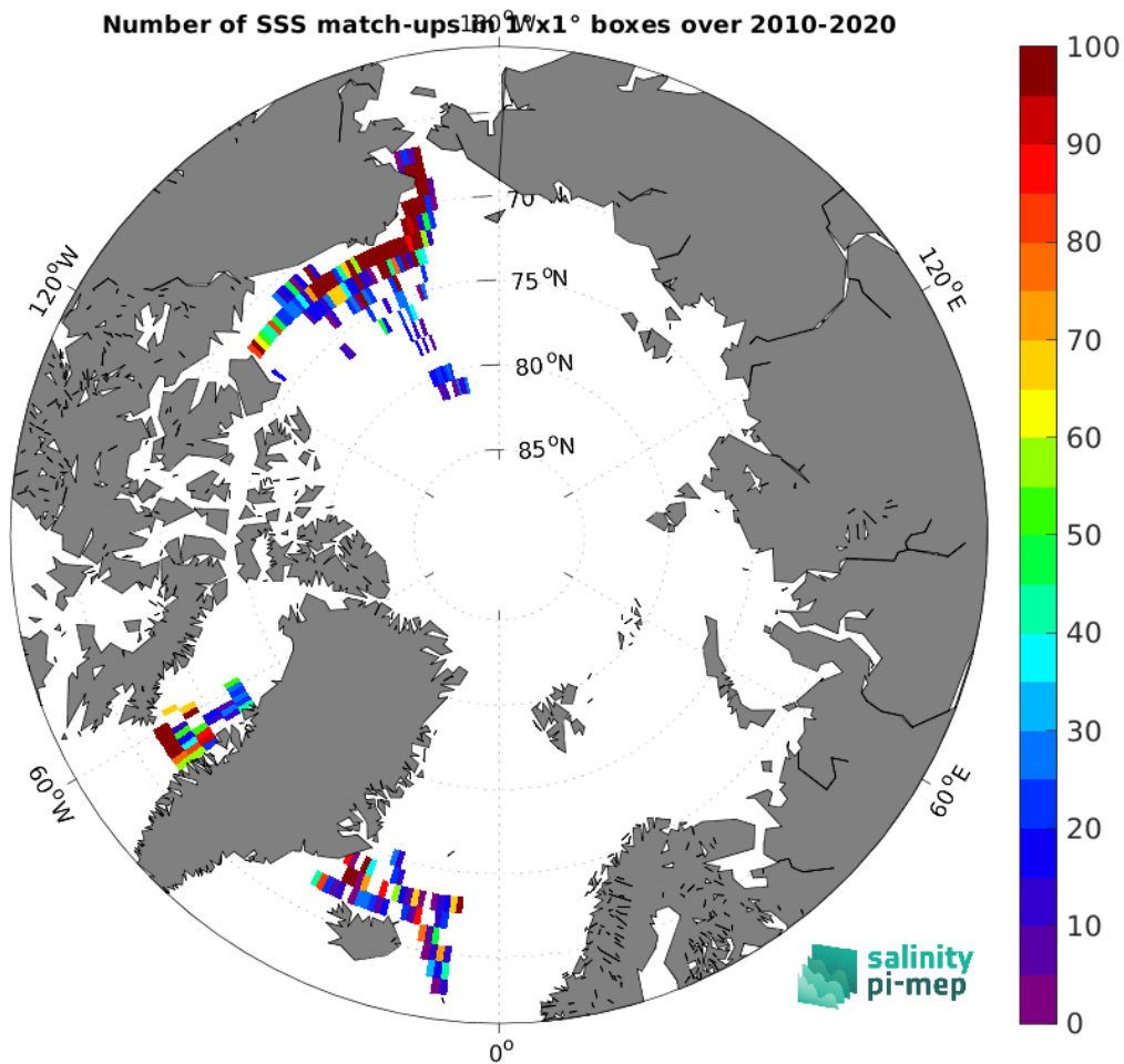
Figure 5: Number of SSS match-ups between TSG (SAMOS) SSS and the SMOS SSS L2Q v331 - No FLAG (CMEMS-CATDS-CPDC) SSS product for the Arctic Ocean Pi-MEP region over 1^\circ \times 1^\circ boxes and for the full satellite product period.
