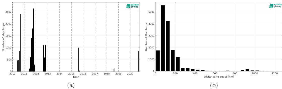
Figure 2: Number of match-ups between TSG (SAMOS) and SMOS SSS L2Q v331 - No FLAG (CMEMS-CATDS-CPDC) SSS as a function of time (a) and as function of the distance to coast (b) over the Arctic Ocean Pi-MEP region and for the full satellite product period.
