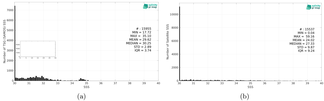
Figure 2: Histograms of SSS from TSG (SAMOS) (a) and SMOS SSS L2Q v331 - No FLAG (CMEMS-CATDS-CPDC) (b) considering all match-up pairs per bins of 0.1 over the Arctic Ocean Pi-MEP region and for the full satellite product period.
