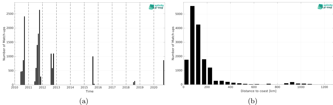
Figure 1: Number of match-ups between TSG (SAMOS) and SMOS SSS L2Q v331 - No FLAG (CMEMS-CATDS-CPDC) SSS as a function of time (a) and as function of the distance to coast (b) over the Arctic Ocean Pi-MEP region and for the full satellite product period.
