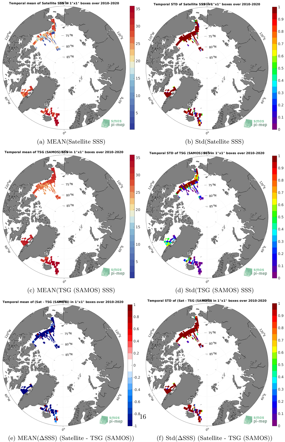
Figure 6: Temporal mean (left) and Std (right) of SSS from SMOS SSS L2Q v331 - No FLAG (CMEMS-CATDS-CPDC) (top), TSG (SAMOS) (middle), and of \Delta SSS (Satellite - TSG (SAMOS)). Only match-up pairs are used to generate these maps.
