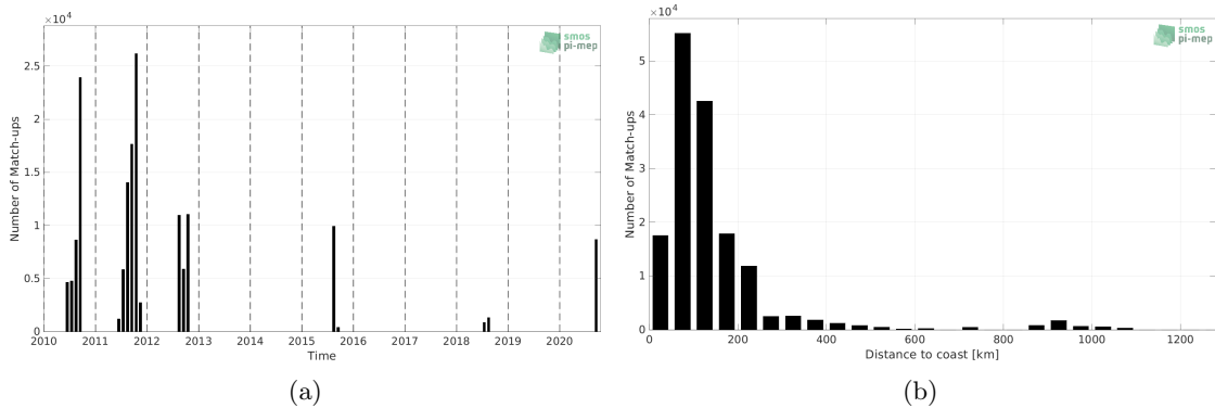
Figure 1: Number of match-ups between TSG (SAMOS) and SMOS SSS L2Q v331 - No FLAG (CMEMS-CATDS-CPDC) SSS as a function of time (a) and as function of the distance to coast (b) over the Arctic Ocean Pi-MEP region and for the full satellite product period.
