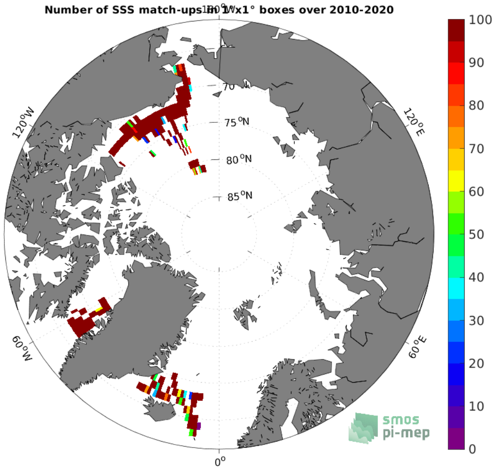
Figure 4: Number of SSS match-ups between TSG (SAMOS) SSS and the SMOS SSS L2Q v331 - No FLAG (CMEMS-CATDS-CPDC) SSS product for the Arctic Ocean Pi-MEP region over 1^\circ \times 1^\circ boxes and for the full satellite product period.
