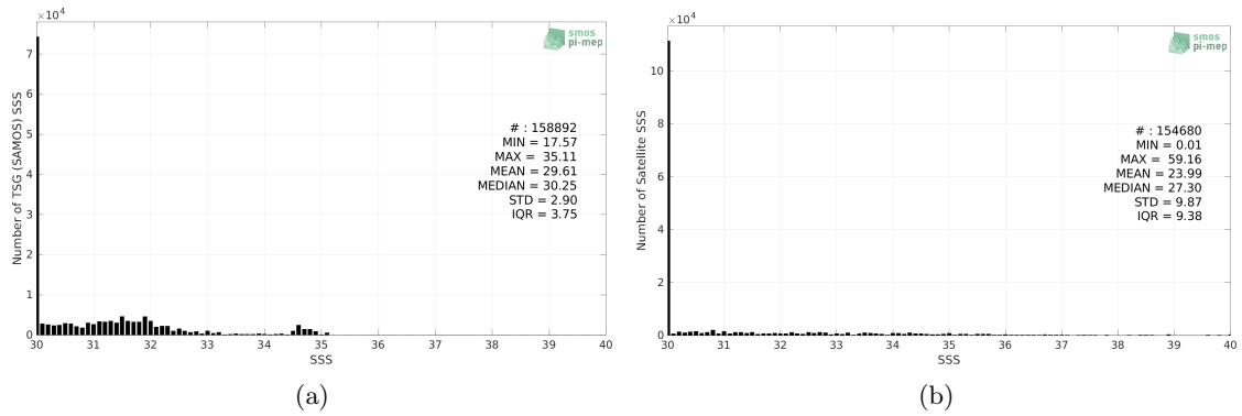
Figure 2: Histograms of SSS from TSG (SAMOS) (a) and SMOS SSS L2Q v331 - No FLAG (CMEMS-CATDS-CPDC) (b) considering all match-up pairs per bins of 0.1 over the Arctic Ocean Pi-MEP region and for the full satellite product period.
