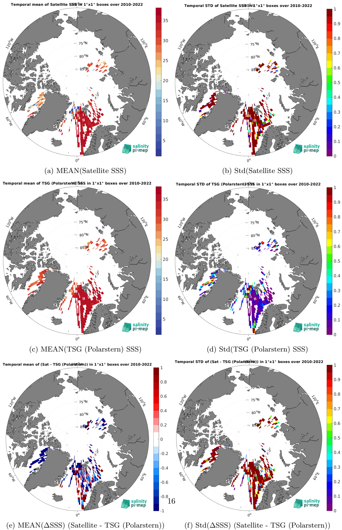
Figure 7: Temporal mean (left) and Std (right) of SSS from SMOS SSS L2Q v331 - No FLAG (CMEMS-CATDS-CPDC) (top), TSG (Polarstern) (middle), and of \Delta SSS (Satellite - TSG (Polarstern)). Only match-up pairs are used to generate these maps.
