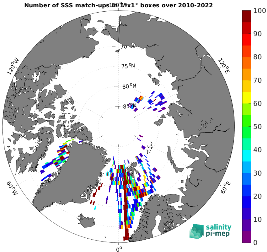
Figure 5: Number of SSS match-ups between TSG (Polarstern) SSS and the SMOS SSS L2Q v331 - No FLAG (CMEMS-CATDS-CPDC) SSS product for the Arctic Ocean Pi-MEP region over 1^\circ \times 1^\circ boxes and for the full satellite product period.
