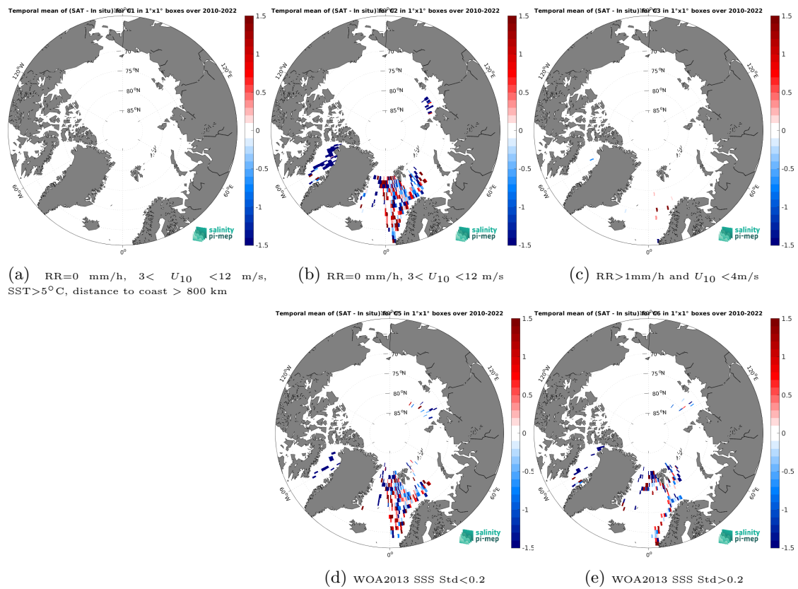
Figure 14: Temporal mean gridded over spatial boxes of size 1^\circ \times 1^\circ of \Delta\text{SSS} (SMOS SSS L2Q v331 - No FLAG (CMEMS-CATDS-CPDC) - TSG (Polarstern)) for 5 different subdatasets corresponding to: RR=0 mm/h, 3 < U_{10} < 12 m/s, SST > 5^\circ\text{C} , distance to coast > 800 km (a), RR=0 mm/h, 3 < U_{10} < 12 m/s (b), RR > 1 mm/h and U_{10} < 4 m/s (c), WOA2013 SSS Std < 0.2 (d), WOA2013 SSS Std > 0.2 (e).
