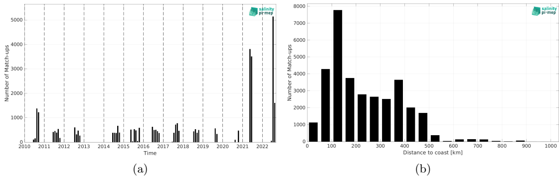
Figure 2: Number of match-ups between TSG (Polarstern) and SMOS SSS L2Q v331 - No FLAG (CMEMS-CATDS-CPDC) SSS as a function of time (a) and as function of the distance to coast (b) over the Arctic Ocean Pi-MEP region and for the full satellite product period.
