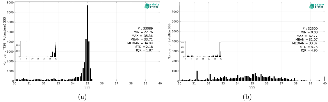
Figure 3: Histograms of SSS from TSG (Polarstern) (a) and SMOS SSS L2Q v331 - No FLAG (CMEMS-CATDS-CPDC) (b) considering all match-up pairs per bins of 0.1 over the Arctic Ocean Pi-MEP region and for the full satellite product period.
