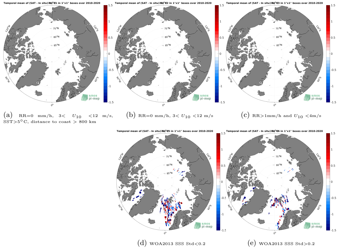
Figure 12: Temporal mean gridded over spatial boxes of size 1^{\circ}\times 1^{\circ} of \Delta\text{SSS} (SMOS SSS L2Q v331 - No FLAG (CMEMS-CATDS-CPDC) - TSG (Polarstern)) for 5 different subdatasets corresponding to:RR=0 mm/h, 3 < U_{10} < 12 m/s, SST >5^{\circ}\text{C} , distance to coast > 800 km (a), RR=0 mm/h, 3 < U_{10} < 12 m/s (b), RR >1 mm/h and U_{10} < 4 m/s (c), WOA2013 SSS Std <0.2 (d), WOA2013 SSS Std >0.2 (e).
