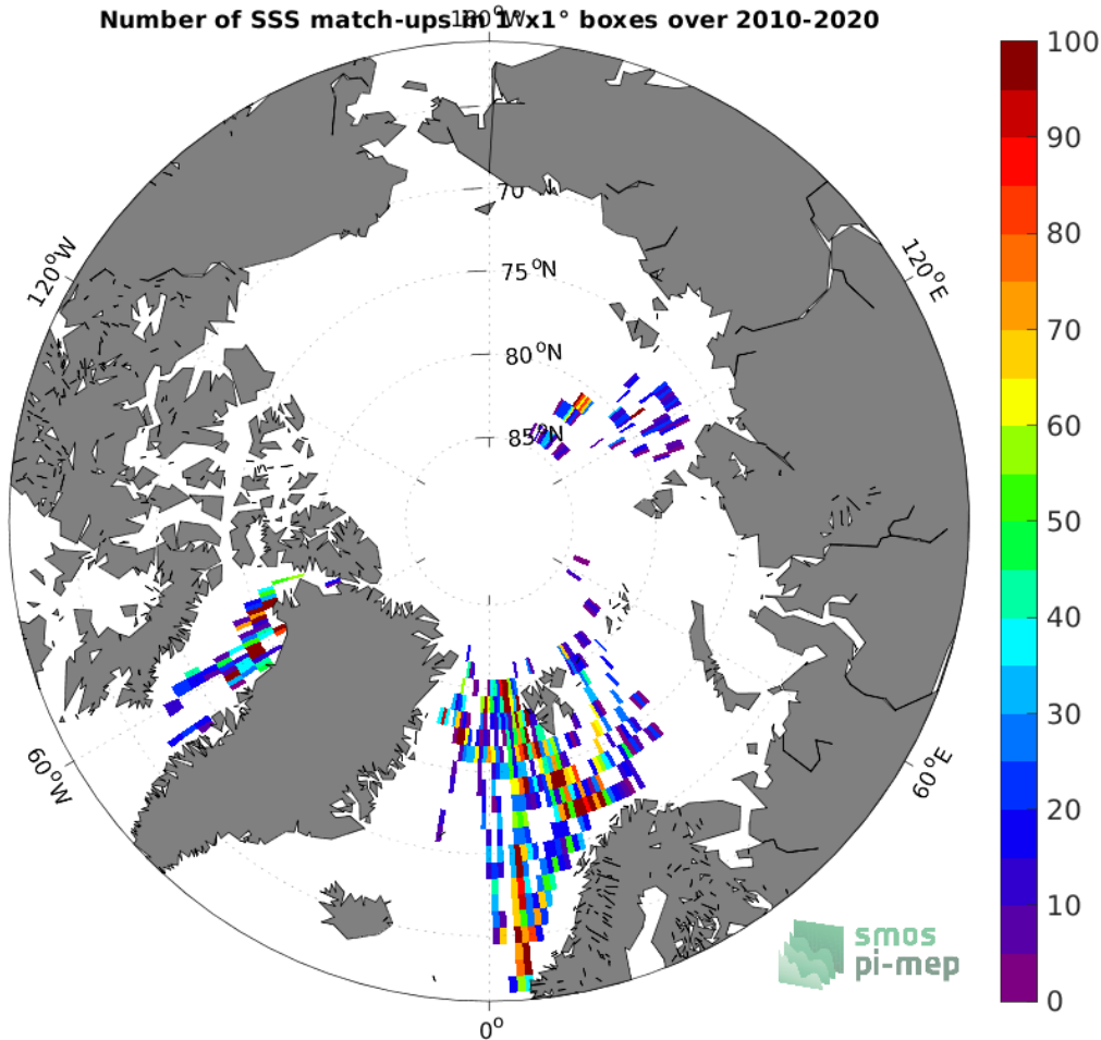
Figure 4: Number of SSS match-ups between TSG (Polarstern) SSS and the SMOS SSS L2Q v331 - No FLAG (CMEMS-CATDS-CPDC) SSS product for the Arctic Ocean Pi-MEP region over 1^\circ \times 1^\circ boxes and for the full satellite product period.
