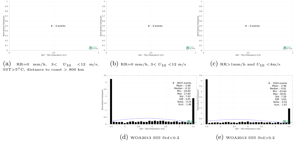
Figure 13: Normalized histogram of \Delta SSS (SMOS SSS L2Q v331 - No FLAG (CMEMS-CATDS-CPDC) - TSG (Polarstern)) for 5 different subdatasets corresponding to: RR=0 mm/h, 3 < U_{10} < 12 m/s, SST>5°C, distance to coast > 800 km (a), RR=0 mm/h, 3 < U_{10} < 12 m/s (b), RR>1mm/h and U_{10} < 4 m/s (c), WOA2013 SSS Std<0.2 (d), WOA2013 SSS Std>0.2 (e).
