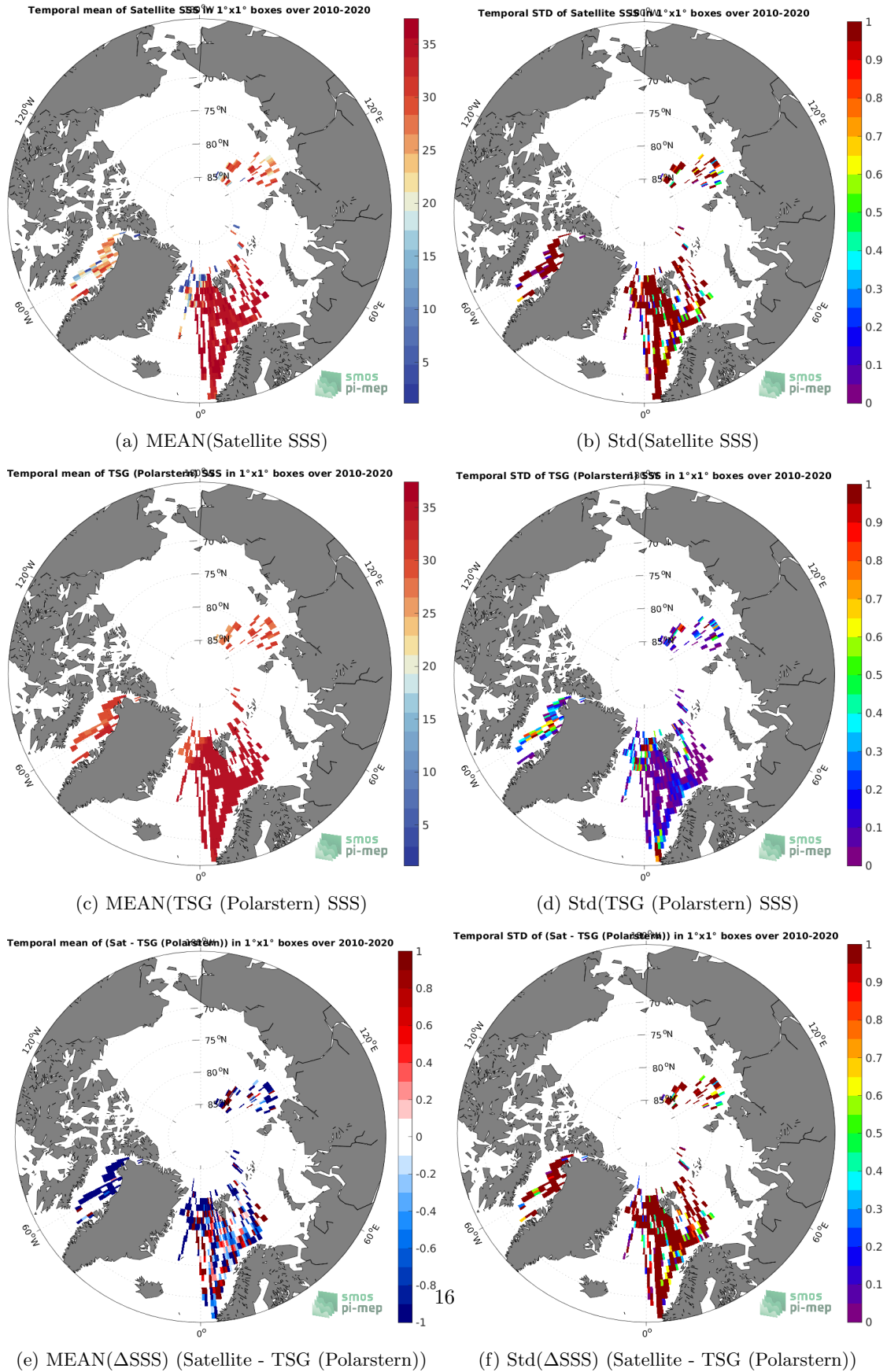
Figure 6: Temporal mean (left) and Std (right) of SSS from SMOS SSS L2Q v331 - No FLAG (CMEMS-CATDS-CPDC) (top), TSG (Polarstern) (middle), and of \Delta SSS (Satellite - TSG (Polarstern)). Only match-up pairs are used to generate these maps.
