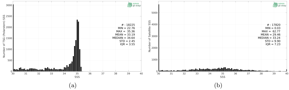
Figure 2: Histograms of SSS from TSG (Polarstern) (a) and SMOS SSS L2Q v331 - No FLAG (CMEMS-CATDS-CPDC) (b) considering all match-up pairs per bins of 0.1 over the Arctic Ocean Pi-MEP region and for the full satellite product period.
