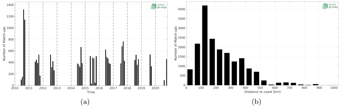
Figure 1: Number of match-ups between TSG (Polarstern) and SMOS SSS L2Q v331 - No FLAG (CMEMS-CATDS-CPDC) SSS as a function of time (a) and as function of the distance to coast (b) over the Arctic Ocean Pi-MEP region and for the full satellite product period.
