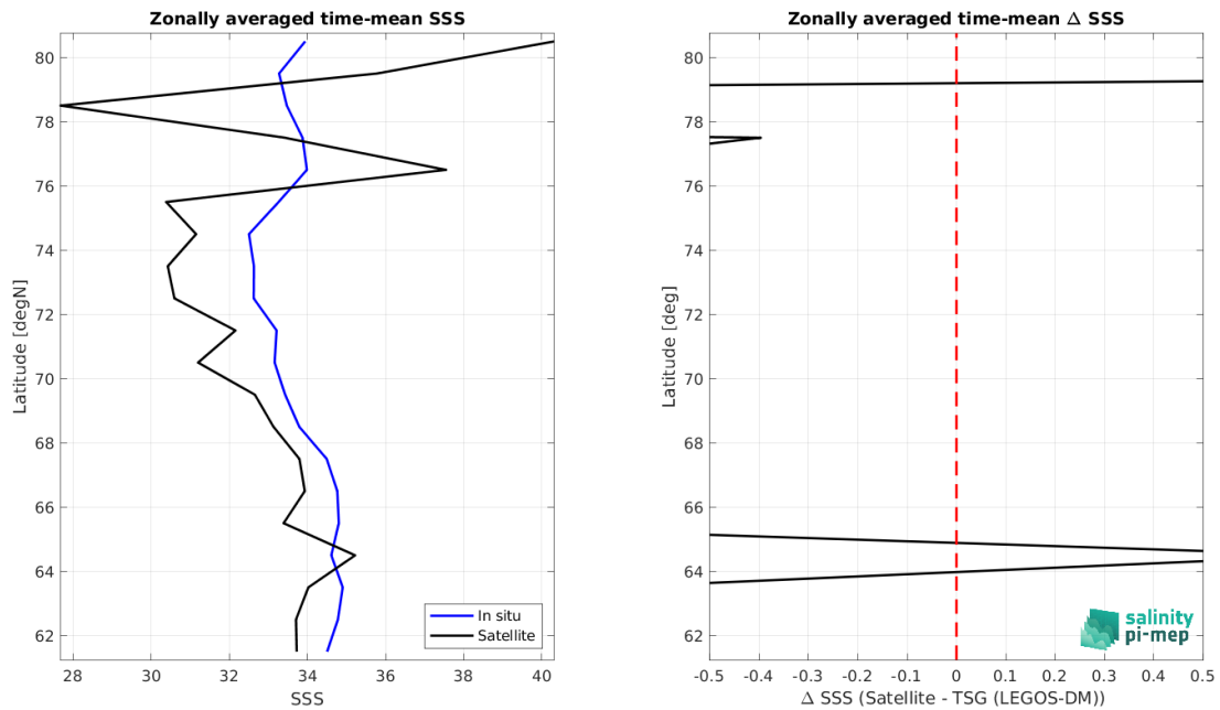
Figure 9: Left panel: Zonal mean SSS from SMOS SSS L2Q v331 - No FLAG (CMEMS-CATDS-CPDC) satellite product (black) and from TSG (LEGOS-DM) (blue). Right panel: Zonal mean of \Delta SSS (Satellite - TSG (LEGOS-DM)) for all the collected Pi-MEP match-up pairs estimated over the full satellite product period.
