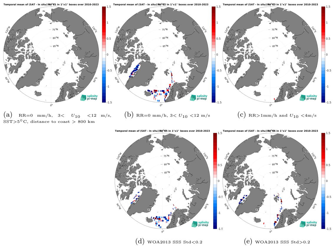
Figure 14: Temporal mean gridded over spatial boxes of size 1^\circ \times 1^\circ of \Delta\text{SSS} (SMOS SSS L2Q v331 - No FLAG (CMEMS-CATDS-CPDC) - TSG (LEGOS-DM)) for 5 different subdatasets corresponding to: RR=0 mm/h, 3 < U_{10} < 12 m/s, SST > 5°C, distance to coast > 800 km (a), RR=0 mm/h, 3 < U_{10} < 12 m/s (b), RR > 1mm/h and U_{10} < 4 m/s (c), WOA2013 SSS Std < 0.2 (d), WOA2013 SSS Std > 0.2 (e).
