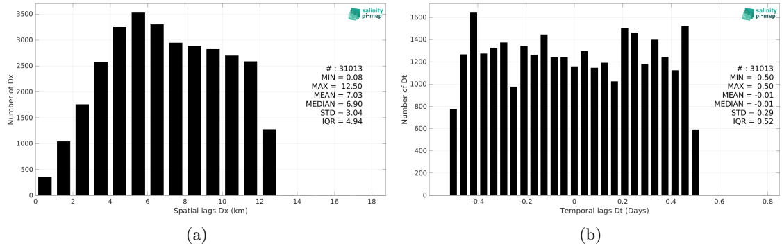
Figure 6: Histograms of the spatial (a) and temporal (b) lags between the location/time of the TSG (LEGOS-DM) measurement and the date of the corresponding SMOS SSS L2Q v331 - No FLAG (CMEMS-CATDS-CPDC) SSS pixel.
