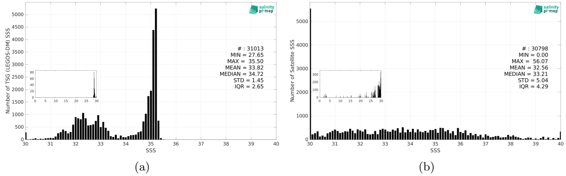
Figure 3: Histograms of SSS from TSG (LEGOS-DM) (a) and SMOS SSS L2Q v331 - No FLAG (CMEMS-CATDS-CPDC) (b) considering all match-up pairs per bins of 0.1 over the Arctic Ocean Pi-MEP region and for the full satellite product period.
