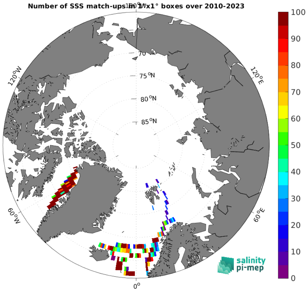
Figure 5: Number of SSS match-ups between TSG (LEGOS-DM) SSS and the SMOS SSS L2Q v331 - No FLAG (CMEMS-CATDS-CPDC) SSS product for the Arctic Ocean Pi-MEP region over 1^\circ \times 1^\circ boxes and for the full satellite product period.
