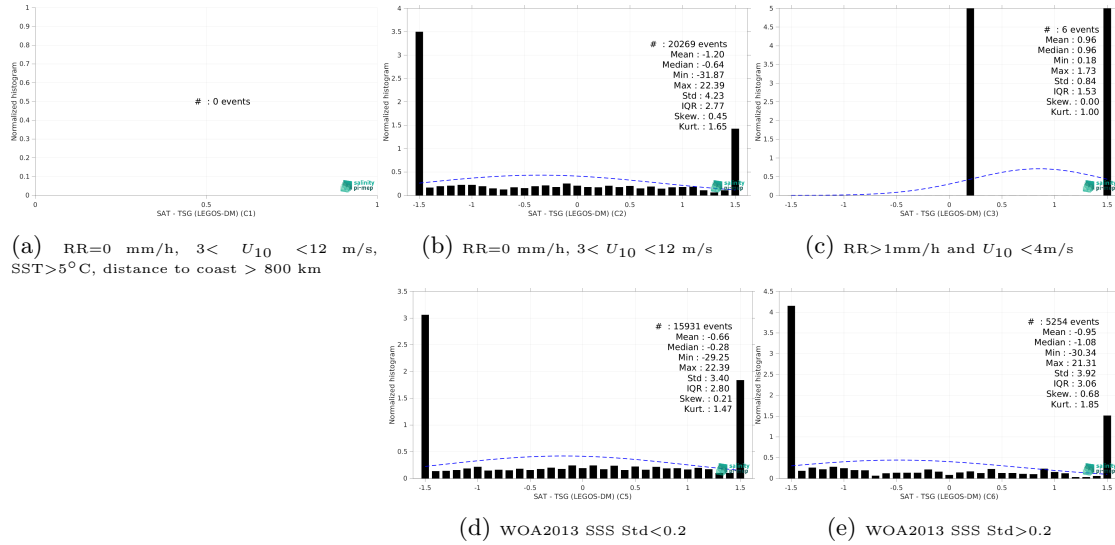
Figure 15: Normalized histogram of \Delta SSS (SMOS SSS L2Q v331 - No FLAG (CMEMS-CATDS-CPDC) - TSG (LEGOS-DM)) for 5 different subdatasets corresponding to: RR=0 mm/h, 3 < U_{10} < 12 m/s, SST > 5°C, distance to coast > 800 km (a), RR=0 mm/h, 3 < U_{10} < 12 m/s (b), RR > 1mm/h and U_{10} < 4 m/s (c), WOA2013 SSS Std < 0.2 (d), WOA2013 SSS Std > 0.2 (e).
