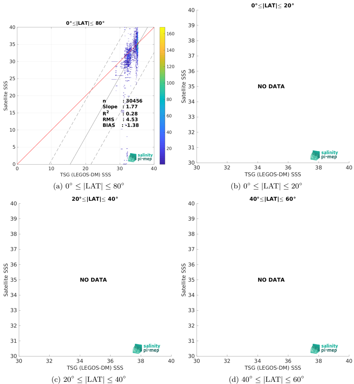
Figure 10: Contour maps of the concentration of SMOS SSS L2Q v331 - No FLAG (CMEMS-CATDS-CPDC) SSS (y-axis) versus TSG (LEGOS-DM) SSS (x-axis) at match-up pairs for different latitude bands. For each plot, the red line shows x=y . The black thin and dashed lines indicate a linear fit through the data cloud and the \pm 95\% confidence levels, respectively. The number match-up pairs n , the slope and R^2 coefficient of the linear fit, the root mean square (RMS) and the mean bias between satellite and in situ data are indicated for each latitude band in each plots.
