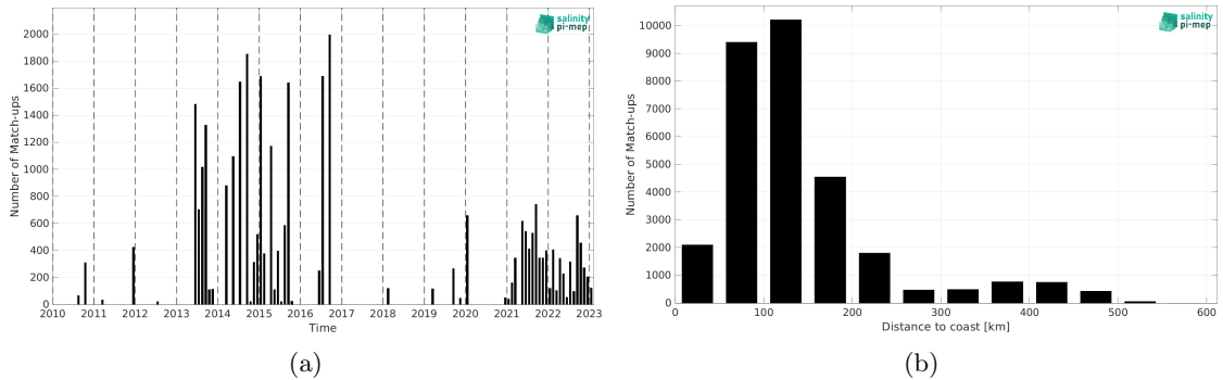
Figure 1: Number of match-ups between TSG (LEGOS-DM) and SMOS SSS L2Q v331 - No FLAG (CMEMS-CATDS-CPDC) SSS as a function of time (a) and as function of the distance to coast (b) over the Arctic Ocean Pi-MEP region and for the full satellite product period.
