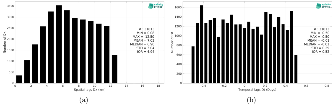
Figure 5: Histograms of the spatial (a) and temporal (b) lags between the location/time of the TSG (LEGOS-DM) measurement and the date of the corresponding SMOS SSS L2Q v331 - No FLAG (CMEMS-CATDS-CPDC) SSS pixel.
