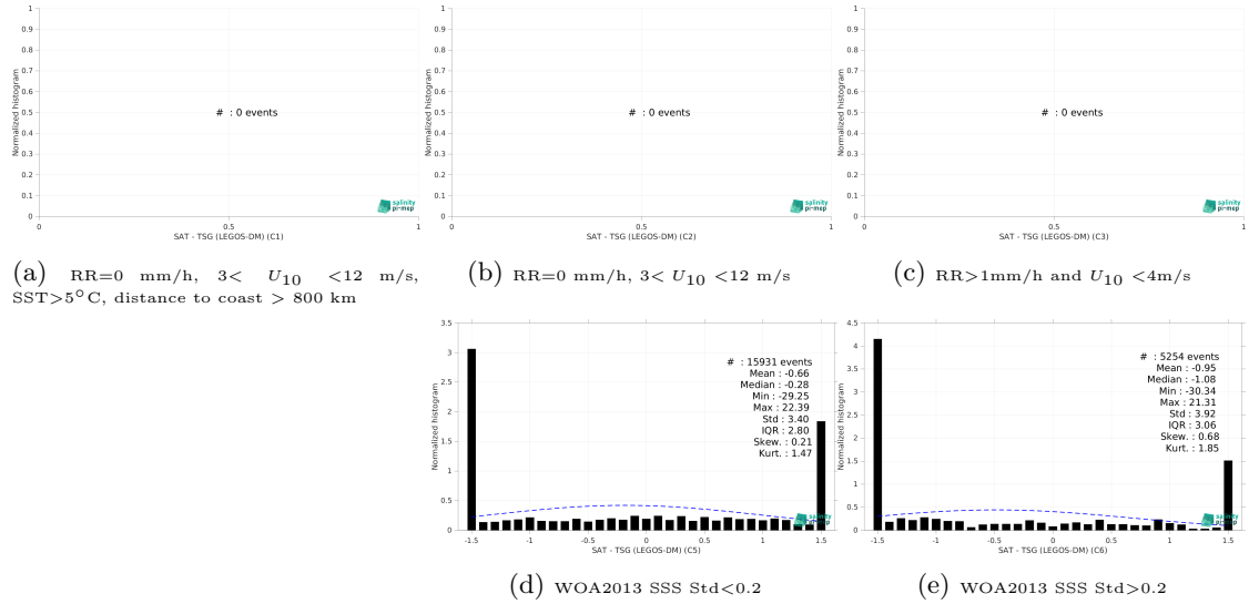
Figure 13: Normalized histogram of \Delta SSS (SMOS SSS L2Q v331 - No FLAG (CMEMS-CATDS-CPDC) - TSG (LEGOS-DM)) for 5 different subdatasets corresponding to: RR=0 mm/h, 3 < U_{10} < 12 m/s, SST > 5°C, distance to coast > 800 km (a), RR=0 mm/h, 3 < U_{10} < 12 m/s (b), RR > 1mm/h and U_{10} < 4 m/s (c), WOA2013 SSS Std < 0.2 (d), WOA2013 SSS Std > 0.2 (e).
