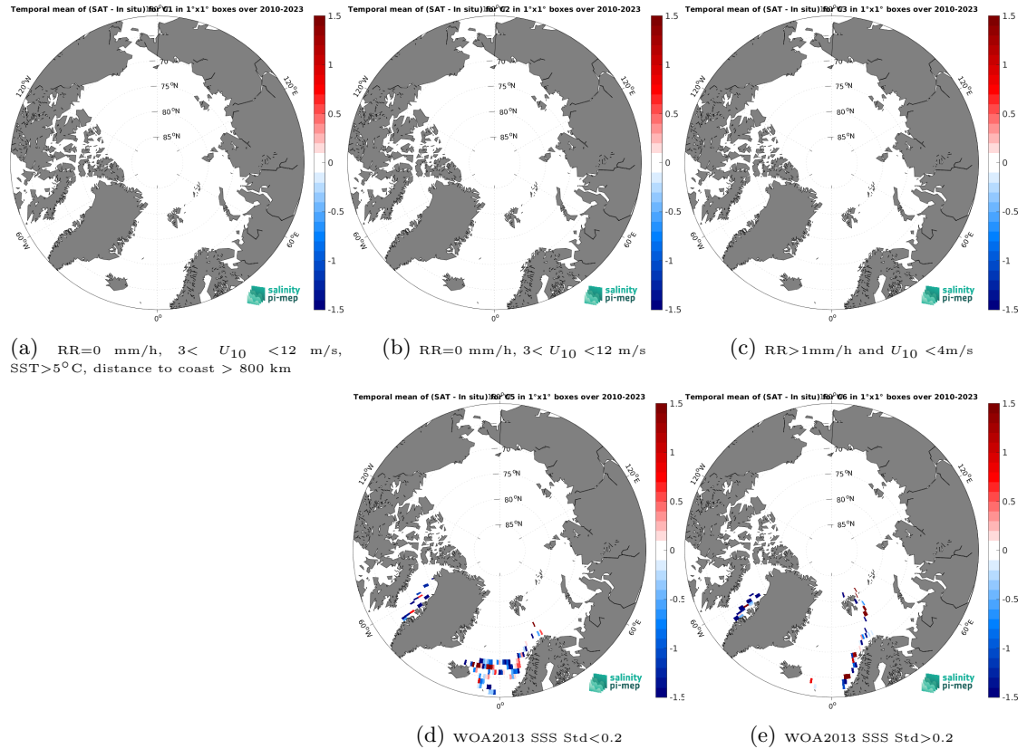
Figure 12: Temporal mean gridded over spatial boxes of size 1^{\circ}\times 1^{\circ} of \Delta\text{SSS} (SMOS SSS L2Q v331 - No FLAG (CMEMS-CATDS-CPDC) - TSG (LEGOS-DM)) for 5 different subdatasets corresponding to:RR=0 mm/h, 3 < U_{10} < 12 m/s, SST >5^{\circ}\text{C} , distance to coast > 800 km (a), RR=0 mm/h, 3 < U_{10} < 12 m/s (b), RR >1 mm/h and U_{10} < 4 m/s (c), WOA2013 SSS Std <0.2 (d), WOA2013 SSS Std >0.2 (e).
