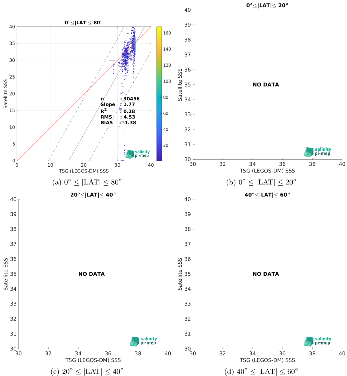
Figure 9: Contour maps of the concentration of SMOS SSS L2Q v331 - No FLAG (CMEMS-CATDS-CPDC) SSS (y-axis) versus TSG (LEGOS-DM) SSS (x-axis) at match-up pairs for different latitude bands. For each plot, the red line shows x=y . The black thin and dashed lines indicate a linear fit through the data cloud and the \pm 95\% confidence levels, respectively. The number match-up pairs n , the slope and R^2 coefficient of the linear fit, the root mean square (RMS) and the mean bias between satellite and in situ data are indicated for each latitude band in each plots.
