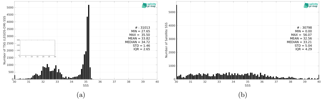
Figure 2: Histograms of SSS from TSG (LEGOS-DM) (a) and SMOS SSS L2Q v331 - No FLAG (CMEMS-CATDS-CPDC) (b) considering all match-up pairs per bins of 0.1 over the Arctic Ocean Pi-MEP region and for the full satellite product period.
