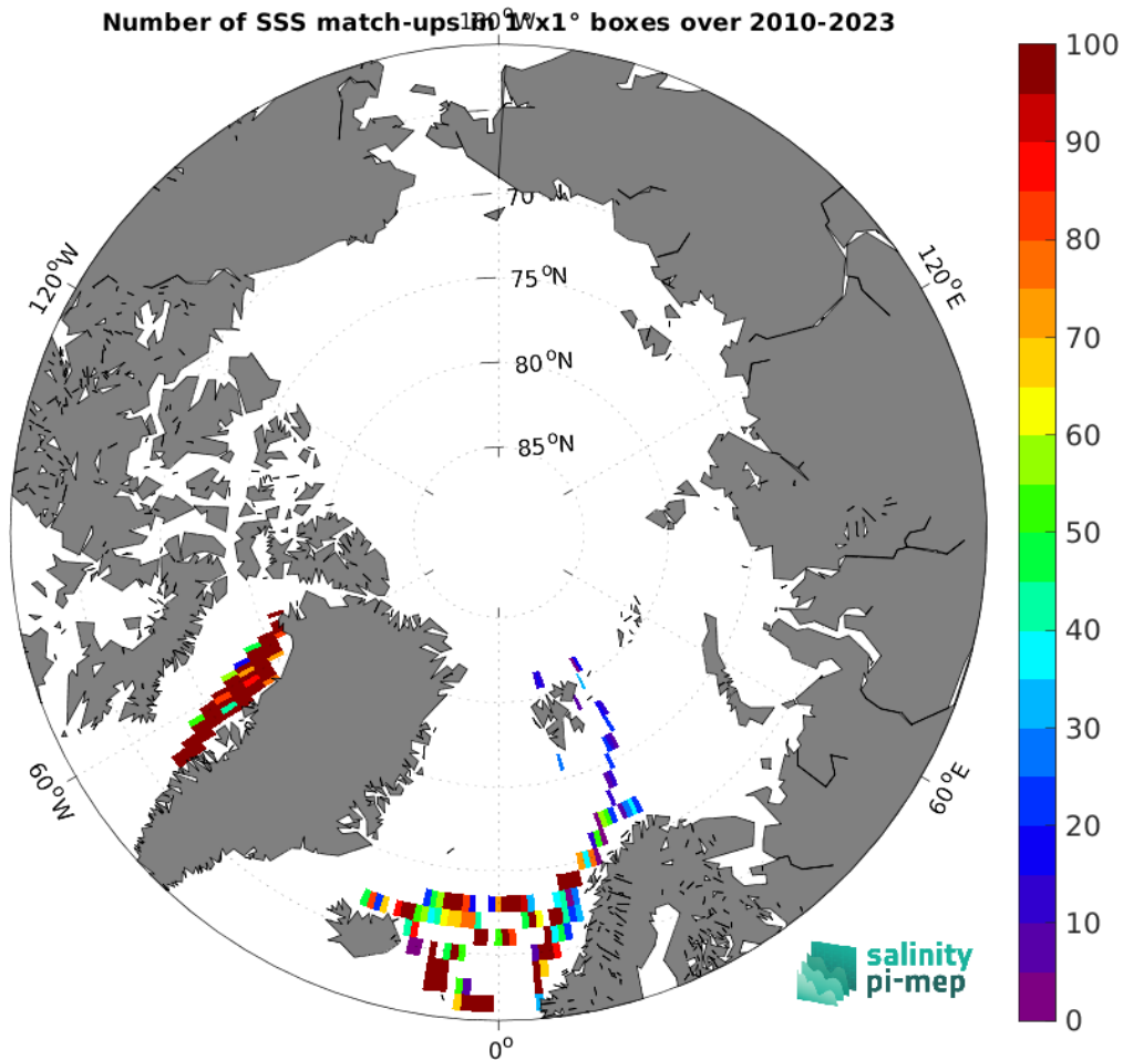
Figure 4: Number of SSS match-ups between TSG (LEGOS-DM) SSS and the SMOS SSS L2Q v331 - No FLAG (CMEMS-CATDS-CPDC) SSS product for the Arctic Ocean Pi-MEP region over 1^\circ \times 1^\circ boxes and for the full satellite product period.
