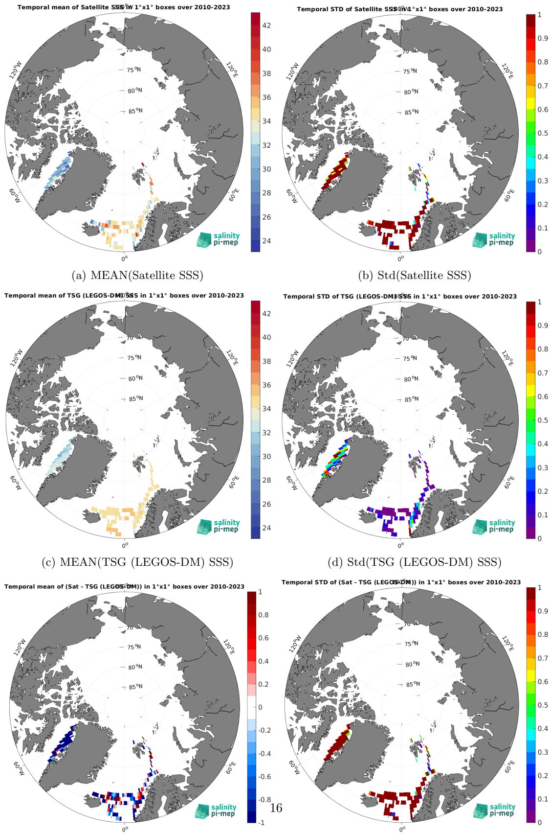
Figure 6: Temporal mean (left) and Std (right) of SSS from SMOS SSS L2Q v331 - No FLAG (CMEMS-CATDS-CPDC) (top), TSG (LEGOS-DM) (middle), and of \Delta SSS (Satellite - TSG (LEGOS-DM)). Only match-up pairs are used to generate these maps.
