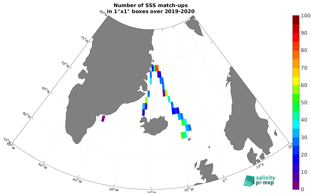
Figure 5: Number of SSS match-ups between TSG (Lauge-Koch) SSS and the SMOS SSS L2Q v331 - No FLAG (CMEMS-CATDS-CPDC) SSS product for the Arctic Ocean Pi-MEP region over 1^\circ \times 1^\circ boxes and for the full satellite product period.
