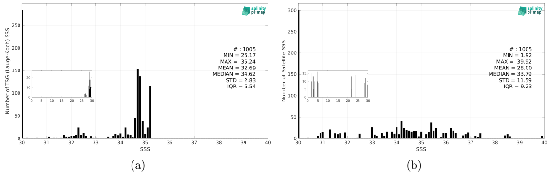
Figure 3: Histograms of SSS from TSG (Lauge-Koch) (a) and SMOS SSS L2Q v331 - No FLAG (CMEMS-CATDS-CPDC) (b) considering all match-up pairs per bins of 0.1 over the Arctic Ocean Pi-MEP region and for the full satellite product period.
