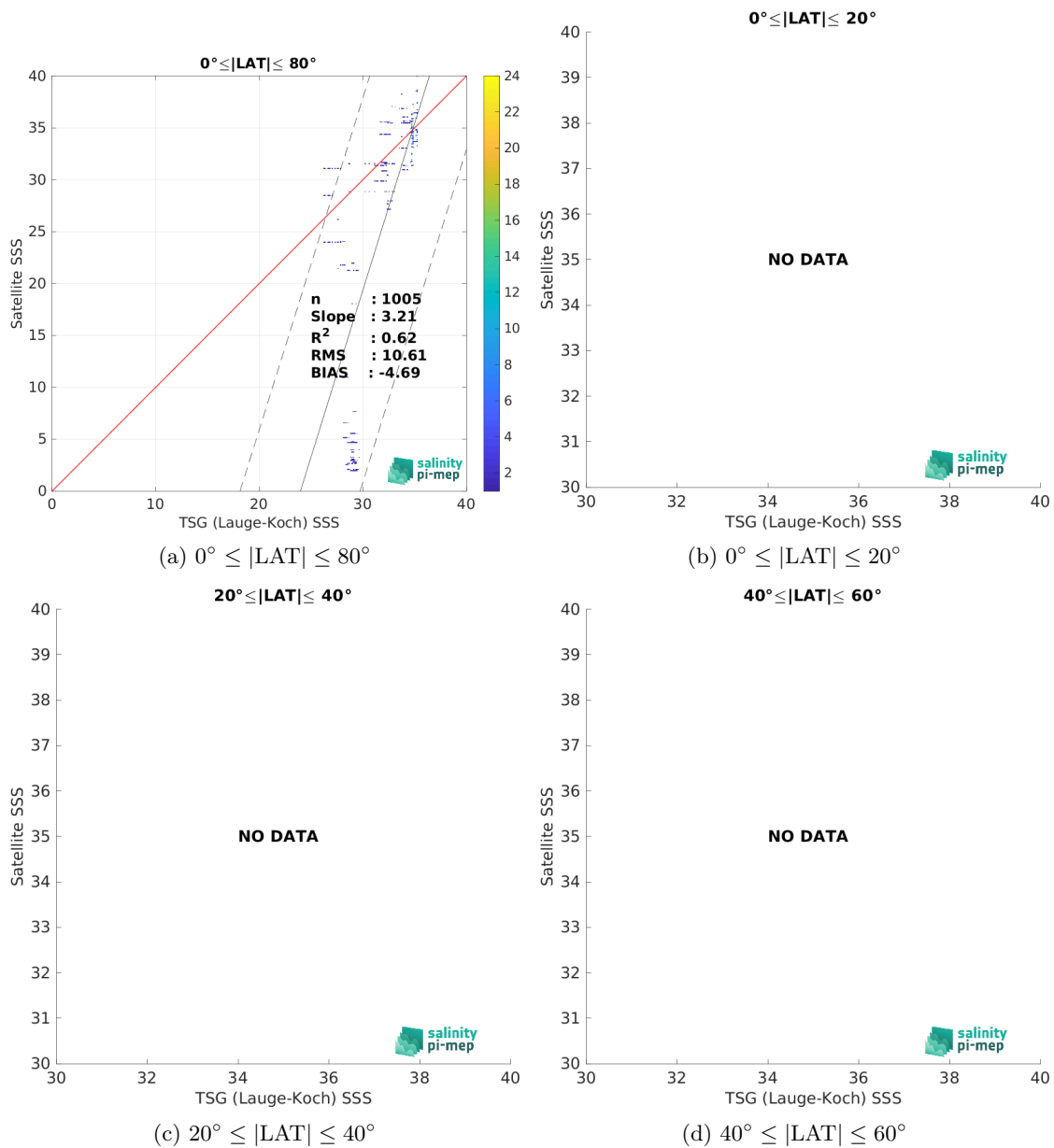
Figure 9: Contour maps of the concentration of SMOS SSS L2Q v331 - No FLAG (CMEMS-CATDS-CPDC) SSS (y-axis) versus TSG (Lauge-Koch) SSS (x-axis) at match-up pairs for different latitude bands. For each plot, the red line shows x=y . The black thin and dashed lines indicate a linear fit through the data cloud and the \pm 95\% confidence levels, respectively. The number match-up pairs n , the slope and R^2 coefficient of the linear fit, the root mean square (RMS) and the mean bias between satellite and in situ data are indicated for each latitude band in each plots.
