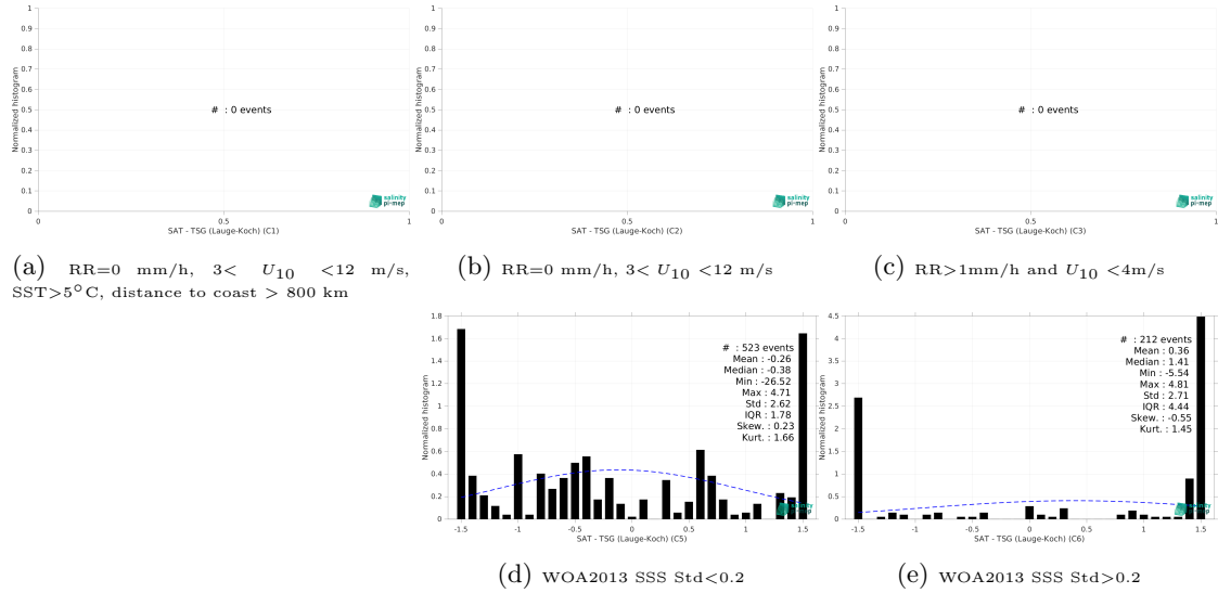
Figure 13: Normalized histogram of \Delta SSS (SMOS SSS L2Q v331 - No FLAG (CMEMS-CATDS-CPDC) - TSG (Laue-Koch)) for 5 different subdatasets corresponding to: RR=0 mm/h, 3 < U_{10} < 12 m/s, SST >5^{\circ} C, distance to coast > 800 km (a), RR=0 mm/h, 3 < U_{10} < 12 m/s (b), RR >1 mm/h and U_{10} < 4 m/s (c), WOA2013 SSS Std <0.2 (d), WOA2013 SSS Std >0.2 (e).
