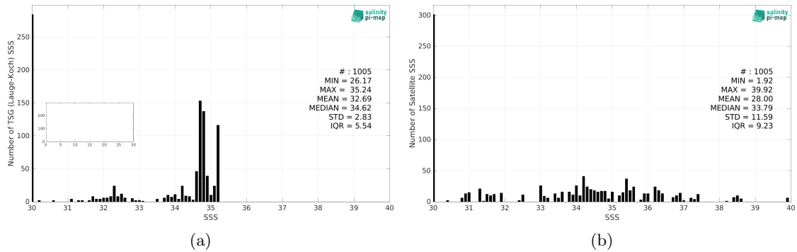
Figure 2: Histograms of SSS from TSG (Lauge-Koch) (a) and SMOS SSS L2Q v331 - No FLAG (CMEMS-CATDS-CPDC) (b) considering all match-up pairs per bins of 0.1 over the Arctic Ocean Pi-MEP region and for the full satellite product period.
