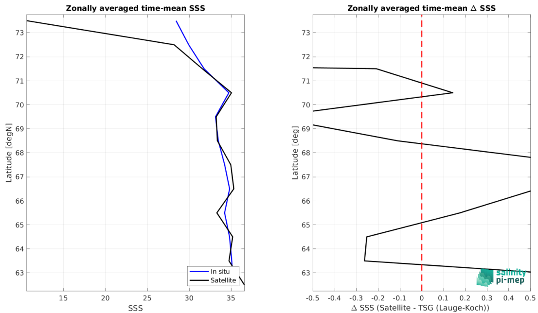
Figure 8: Left panel: Zonal mean SSS from SMOS SSS L2Q v331 - No FLAG (CMEMS-CATDS-CPDC) satellite product (black) and from TSG (Lauge-Koch) (blue). Right panel: Zonal mean of \Delta SSS (Satellite - TSG (Lauge-Koch)) for all the collected Pi-MEP match-up pairs estimated over the full satellite product period.
