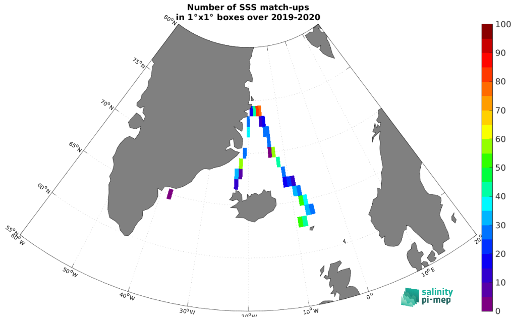
Figure 4: Number of SSS match-ups between TSG (Lauge-Koch) SSS and the SMOS SSS L2Q v331 - No FLAG (CMEMS-CATDS-CPDC) SSS product for the Arctic Ocean Pi-MEP region over 1^\circ \times 1^\circ boxes and for the full satellite product period.
