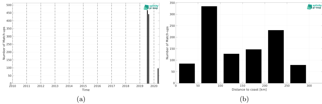
Figure 1: Number of match-ups between TSG (Lauge-Koch) and SMOS SSS L2Q v331 - No FLAG (CMEMS-CATDS-CPDC) SSS as a function of time (a) and as function of the distance to coast (b) over the Arctic Ocean Pi-MEP region and for the full satellite product period.
