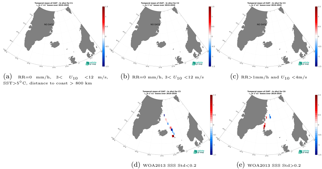
Figure 12: Temporal mean gridded over spatial boxes of size 1^{\circ}\times 1^{\circ} of \Delta\text{SSS} (SMOS SSS L2Q v331 - No FLAG (CMEMS-CATDS-CPDC) - TSG (Lauge-Koch)) for 5 different subdatasets corresponding to:RR=0 mm/h, 3 < U_{10} < 12 m/s, SST >5^{\circ}\text{C} , distance to coast > 800 km (a), RR=0 mm/h, 3 < U_{10} < 12 m/s (b), RR >1 mm/h and U_{10} < 4 m/s (c), WOA2013 SSS Std <0.2 (d), WOA2013 SSS Std >0.2 (e).
