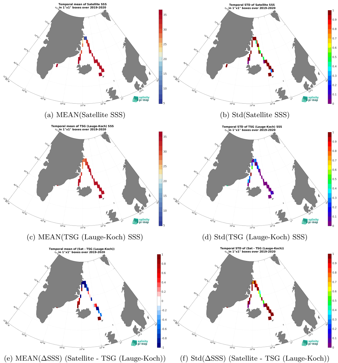
Figure 6: Temporal mean (left) and Std (right) of SSS from SMOS SSS L2Q v331 - No FLAG (CMEMS-CATDS-CPDC) (top), TSG (Lauge-Koch) (middle), and of \Delta SSS (Satellite - TSG (Lauge-Koch)). Only match-up pairs are used to generate these maps.
