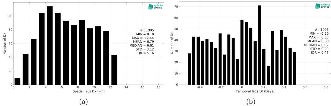
Figure 5: Histograms of the spatial (a) and temporal (b) lags between the location/time of the TSG (Lauge-Koch) measurement and the date of the corresponding SMOS SSS L2Q v331 - No FLAG (CMEMS-CATDS-CPDC) SSS pixel.
