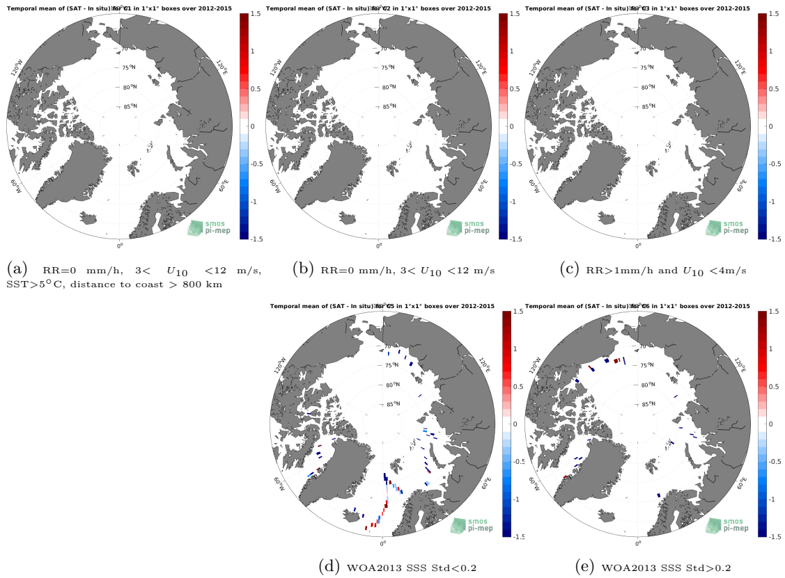
Figure 12: Temporal mean gridded over spatial boxes of size 1^\circ \times 1^\circ of \Delta SSS (SMOS SSS L2Q v331 - No FLAG (CMEMS-CATDS-CPDC) - TSG (GOSUD-Sailing-ship)) for 5 different sub-datasets corresponding to: RR=0 mm/h, 3 < U_{10} < 12 m/s, SST>5°C, distance to coast > 800 km (a), RR=0 mm/h, 3 < U_{10} < 12 m/s (b), RR>1mm/h and U_{10} < 4 m/s (c), WOA2013 SSS Std<0.2 (d), WOA2013 SSS Std>0.2 (e).
