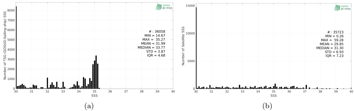
Figure 2: Histograms of SSS from TSG (GOSUD-Sailing-ship) (a) and SMOS SSS L2Q v331 - No FLAG (CMEMS-CATDS-CPDC) (b) considering all match-up pairs per bins of 0.1 over the Arctic Ocean Pi-MEP region and for the full satellite product period.
