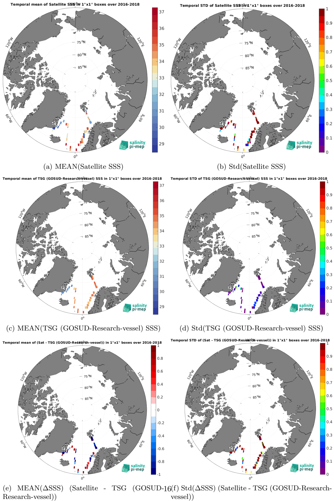
Figure 7: Temporal mean (left) and Std (right) of SSS from SMOS SSS L2Q v331 - No FLAG (CMEMS-CATDS-CPDC) (top), TSG (GOSUD-Research-vessel) (middle), and of \Delta SSS (Satellite - TSG (GOSUD-Research-vessel)). Only match-up pairs are used to generate these maps.
