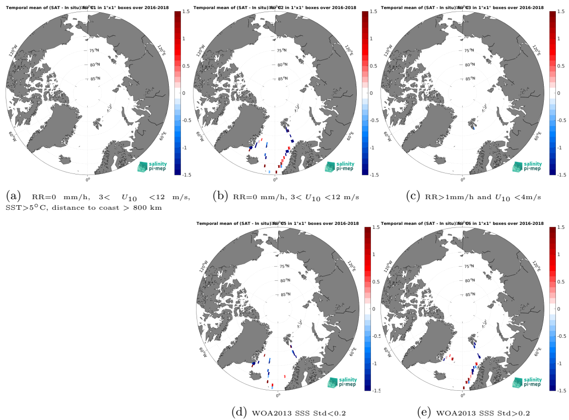
Figure 14: Temporal mean gridded over spatial boxes of size 1^\circ \times 1^\circ of \Delta\text{SSS} (SMOS SSS L2Q v331 - No FLAG (CMEMS-CATDS-CPDC) - TSG (GOSUD-Research-vessel)) for 5 different subdatasets corresponding to:RR=0 mm/h, 3 < U_{10} < 12 m/s, SST > 5°C, distance to coast > 800 km (a), RR=0 mm/h, 3 < U_{10} < 12 m/s (b), RR > 1mm/h and U_{10} < 4 m/s (c), WOA2013 SSS Std < 0.2 (d), WOA2013 SSS Std > 0.2 (e).
