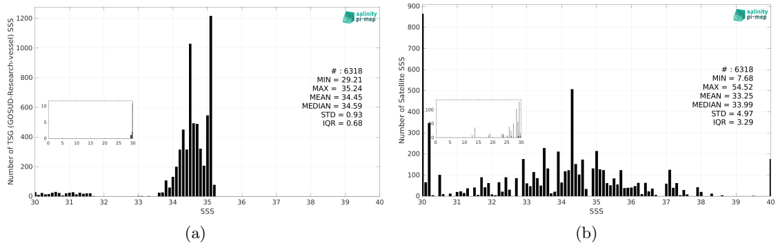
Figure 3: Histograms of SSS from TSG (GOSUD-Research-vessel) (a) and SMOS SSS L2Q v331 - No FLAG (CMEMS-CATDS-CPDC) (b) considering all match-up pairs per bins of 0.1 over the Arctic Ocean Pi-MEP region and for the full satellite product period.
