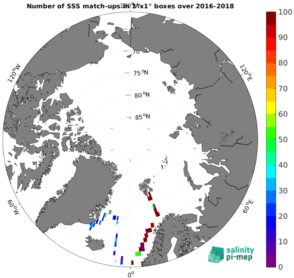
Figure 5: Number of SSS match-ups between TSG (GOSUD-Research-vessel) SSS and the SMOS SSS L2Q v331 - No FLAG (CMEMS-CATDS-CPDC) SSS product for the Arctic Ocean Pi-MEP region over 1^{\circ} \times 1^{\circ} boxes and for the full satellite product period.
