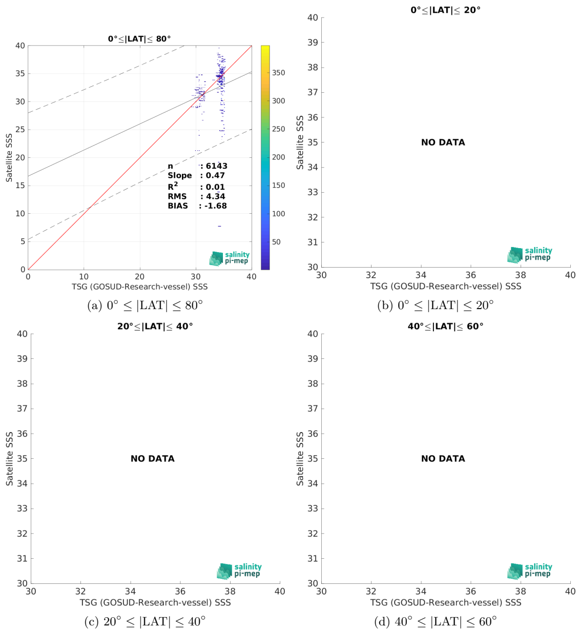
Figure 10: Contour maps of the concentration of SMOS SSS L2Q v331 - No FLAG (CMEMS-CATDS-CPDC) SSS (y-axis) versus TSG (GOSUD-Research-vessel) SSS (x-axis) at match-up pairs for different latitude bands. For each plot, the red line shows x=y . The black thin and dashed lines indicate a linear fit through the data cloud and the \pm 95\% confidence levels, respectively. The number match-up pairs n , the slope and R^2 coefficient of the linear fit, the root mean square (RMS) and the mean bias between satellite and in situ data are indicated for each latitude band in each plots.
