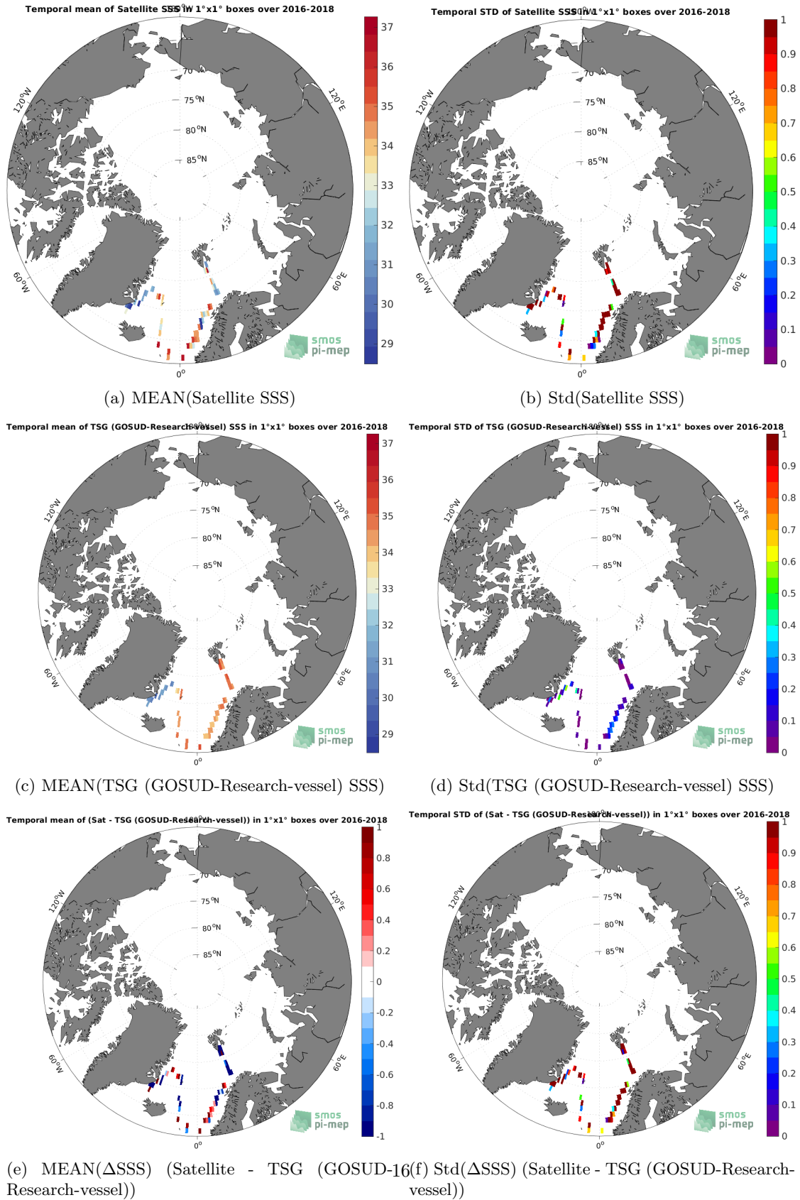
Figure 6: Temporal mean (left) and Std (right) of SSS from SMOS SSS L2Q v331 - No FLAG (CMEMS-CATDS-CPDC) (top), TSG (GOSUD-Research-vessel) (middle), and of \Delta SSS (Satellite - TSG (GOSUD-Research-vessel)). Only match-up pairs are used to generate these maps.
