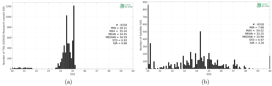
Figure 2: Histograms of SSS from TSG (GOSUD-Research-vessel) (a) and SMOS SSS L2Q v331 - No FLAG (CMEMS-CATDS-CPDC) (b) considering all match-up pairs per bins of 0.1 over the Arctic Ocean Pi-MEP region and for the full satellite product period.
