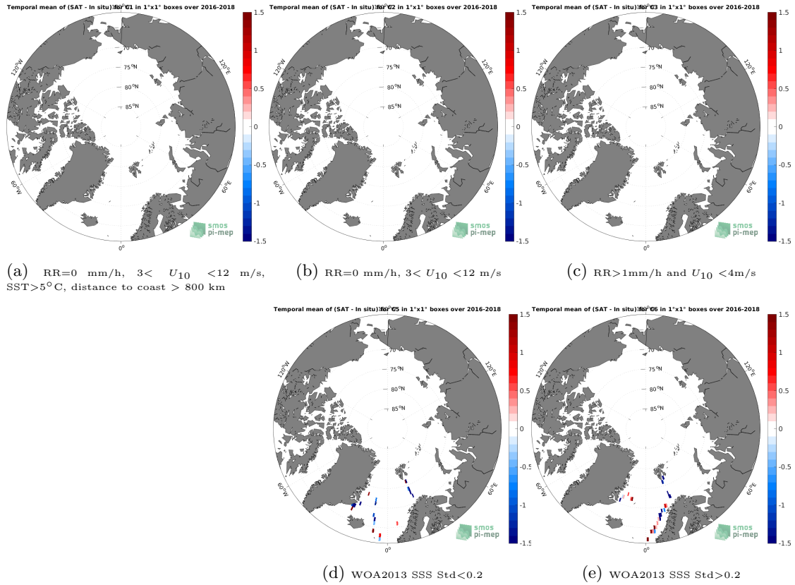
Figure 12: Temporal mean gridded over spatial boxes of size 1^\circ \times 1^\circ of \Delta SSS (SMOS SSS L2Q v331 - No FLAG (CMEMS-CATDS-CPDC) - TSG (GOSUD-Research-vessel)) for 5 different subdatasets corresponding to: RR=0 mm/h, 3 < U_{10} < 12 m/s, SST>5°C, distance to coast > 800 km (a), RR=0 mm/h, 3 < U_{10} < 12 m/s (b), RR>1mm/h and U_{10} < 4 m/s (c), WOA2013 SSS Std<0.2 (d), WOA2013 SSS Std>0.2 (e).
