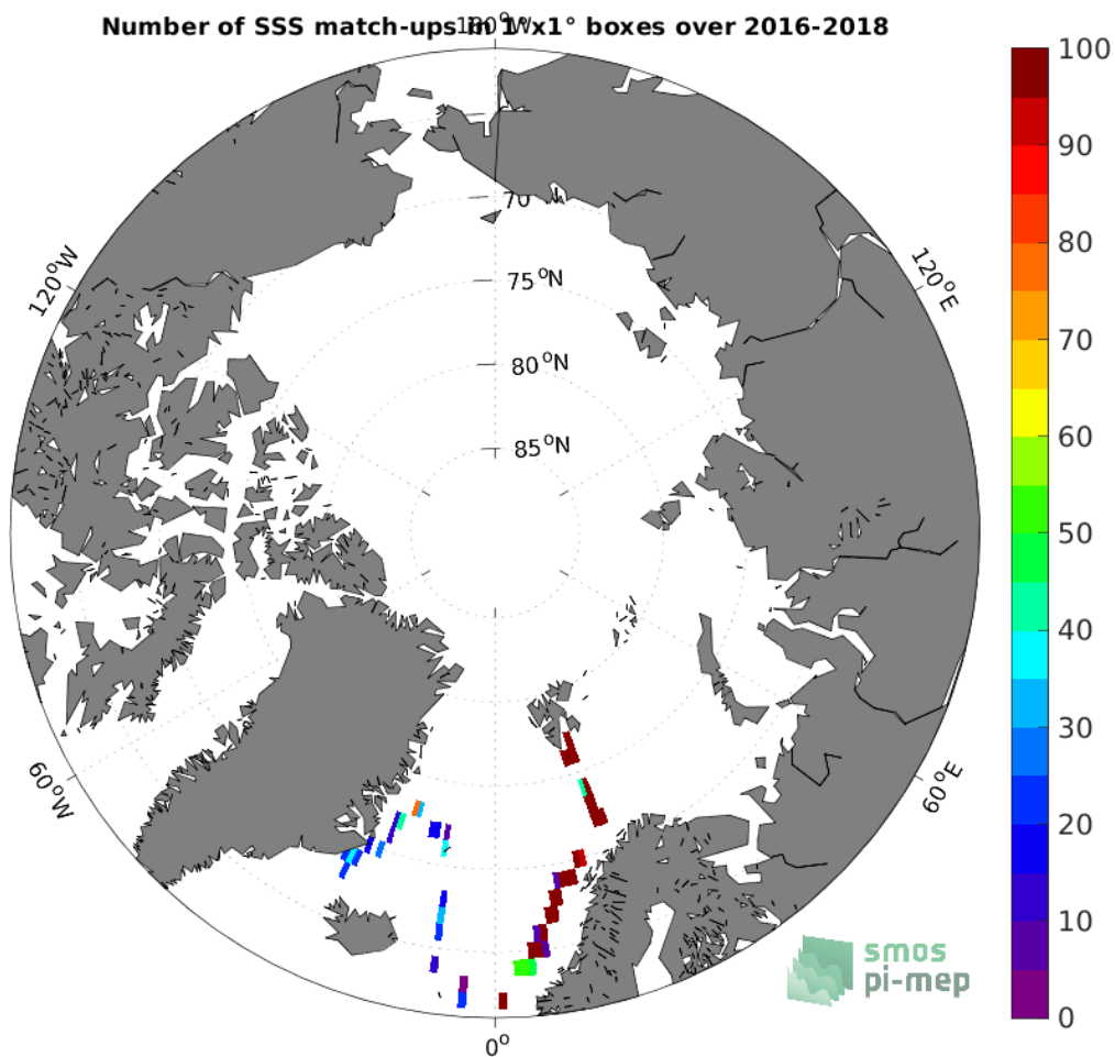
Figure 4: Number of SSS match-ups between TSG (GOSUD-Research-vessel) SSS and the SMOS SSS L2Q v331 - No FLAG (CMEMS-CATDS-CPDC) SSS product for the Arctic Ocean Pi-MEP region over 1^{\circ} \times 1^{\circ} boxes and for the full satellite product period.
