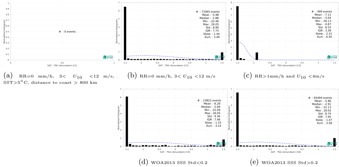
Figure 15: Normalized histogram of \Delta SSS (SMOS SSS L2Q v331 - No FLAG (CMEMS-CATDS-CPDC) - TSG (Amundsen)) for 5 different subdatasets corresponding to: RR=0 mm/h, 3 < U_{10} < 12 m/s, SST>5°C, distance to coast > 800 km (a), RR=0 mm/h, 3 < U_{10} < 12 m/s (b), RR>1mm/h and U_{10} < 4 m/s (c), WOA2013 SSS Std<0.2 (d), WOA2013 SSS Std>0.2 (e).
