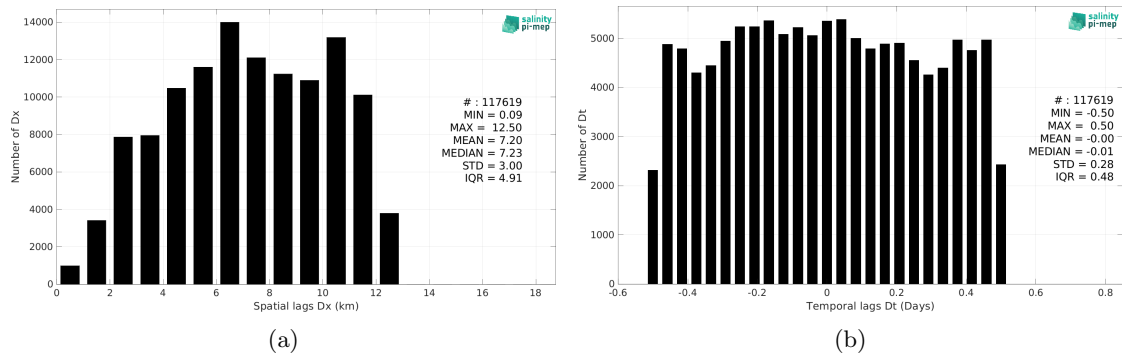
Figure 6: Histograms of the spatial (a) and temporal (b) lags between the location/time of the TSG (Amundsen) measurement and the date of the corresponding SMOS SSS L2Q v331 - No FLAG (CMEMS-CATDS-CPDC) SSS pixel.
