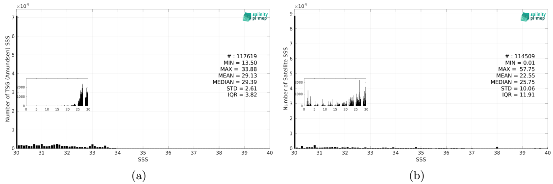
Figure 3: Histograms of SSS from TSG (Amundsen) (a) and SMOS SSS L2Q v331 - No FLAG (CMEMS-CATDS-CPDC) (b) considering all match-up pairs per bins of 0.1 over the Arctic Ocean Pi-MEP region and for the full satellite product period.
