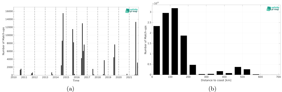
Figure 2: Number of match-ups between TSG (Amundsen) and SMOS SSS L2Q v331 - No FLAG (CMEMS-CATDS-CPDC) SSS as a function of time (a) and as function of the distance to coast (b) over the Arctic Ocean Pi-MEP region and for the full satellite product period.
