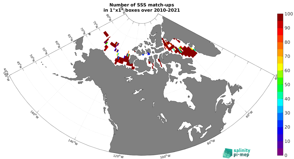
Figure 5: Number of SSS match-ups between TSG (Amundsen) SSS and the SMOS SSS L2Q v331 - No FLAG (CMEMS-CATDS-CPDC) SSS product for the Arctic Ocean Pi-MEP region over 1°×1° boxes and for the full satellite product period.
