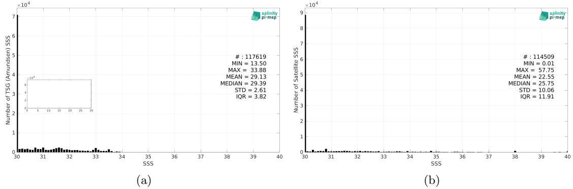
Figure 2: Histograms of SSS from TSG (Amundsen) (a) and SMOS SSS L2Q v331 - No FLAG (CMEMS-CATDS-CPDC) (b) considering all match-up pairs per bins of 0.1 over the Arctic Ocean Pi-MEP region and for the full satellite product period.
