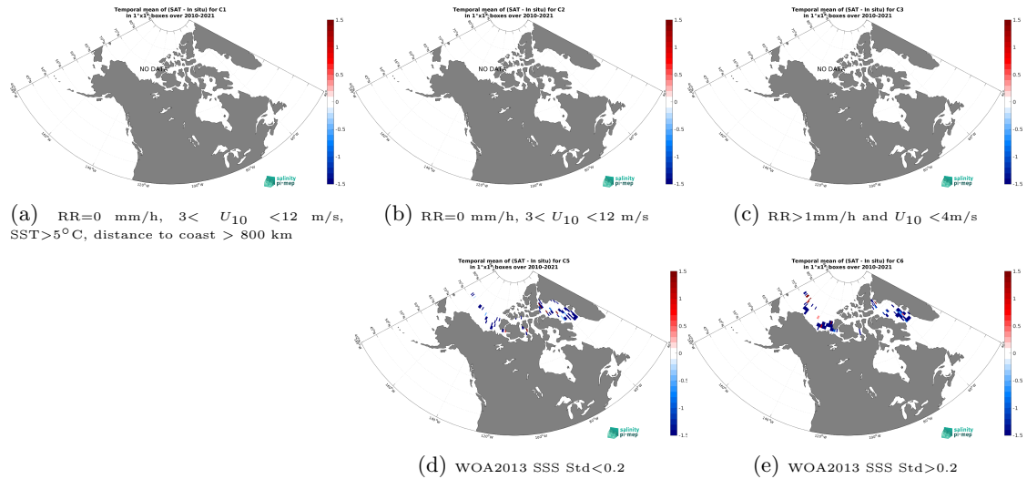
Figure 12: Temporal mean gridded over spatial boxes of size 1^{\circ}\times 1^{\circ} of \Delta\text{SSS} (SMOS SSS L2Q v331 - No FLAG (CMEMS-CATDS-CPDC) - TSG (Amundsen)) for 5 different subdatasets corresponding to:RR=0 mm/h, 3 < U_{10} < 12 m/s, SST >5^{\circ}\text{C} , distance to coast > 800 km (a), RR=0 mm/h, 3 < U_{10} < 12 m/s (b), RR >1 mm/h and U_{10} < 4 m/s (c), WOA2013 SSS Std <0.2 (d), WOA2013 SSS Std >0.2 (e).
