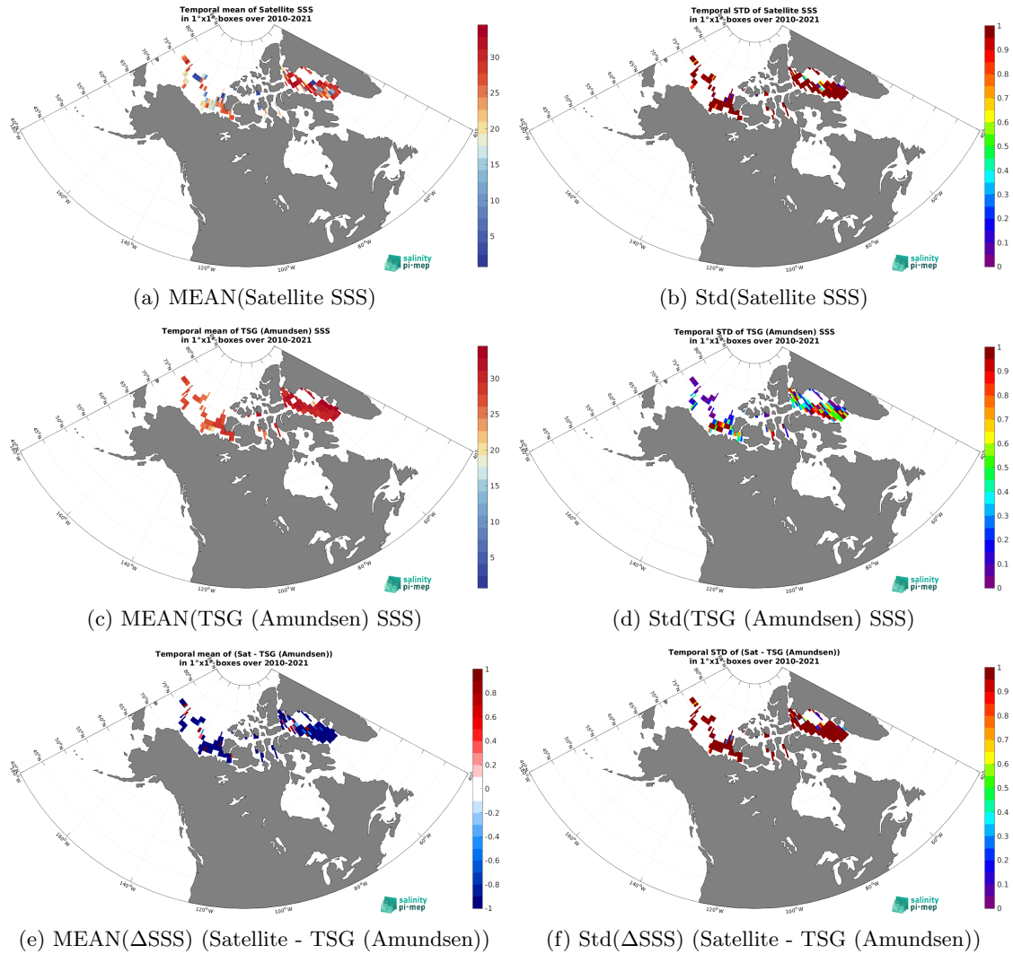
Figure 6: Temporal mean (left) and Std (right) of SSS from SMOS SSS L2Q v331 - No FLAG (CMEMS-CATDS-CPDC) (top), TSG (Amundsen) (middle), and of \Delta SSS (Satellite - TSG (Amundsen)). Only match-up pairs are used to generate these maps.
