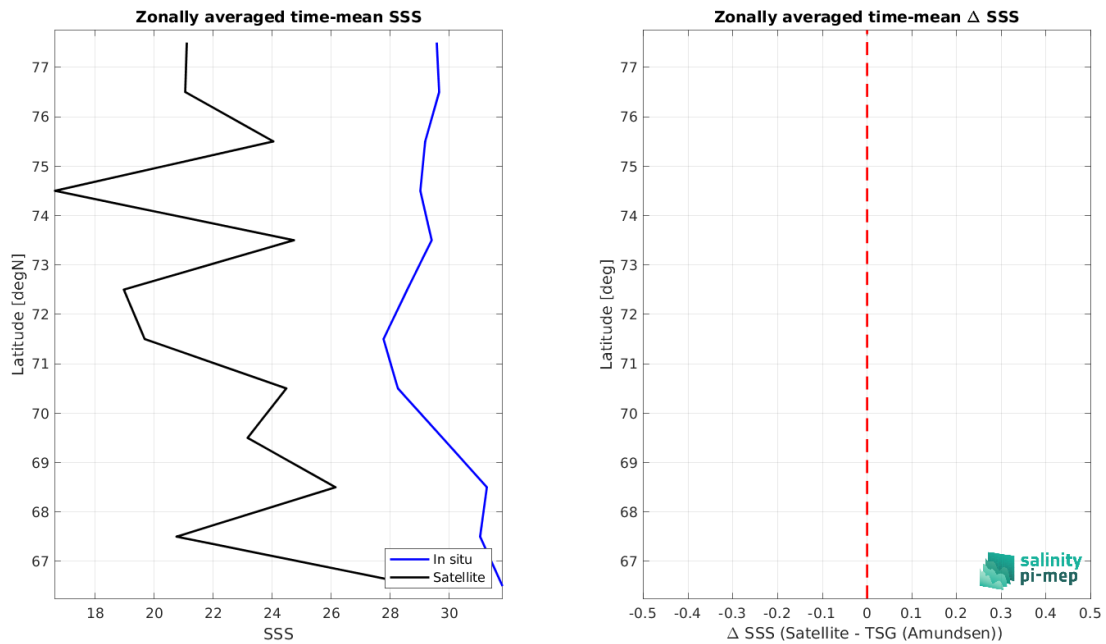
Figure 8: Left panel: Zonal mean SSS from SMOS SSS L2Q v331 - No FLAG (CMEMS-CATDS-CPDC) satellite product (black) and from TSG (Amundsen) (blue). Right panel: Zonal mean of \Delta SSS (Satellite - TSG (Amundsen)) for all the collected Pi-MEP match-up pairs estimated over the full satellite product period.
