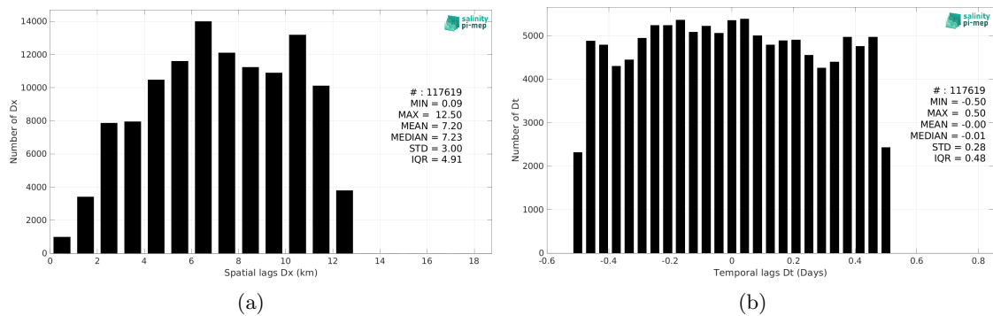
Figure 5: Histograms of the spatial (a) and temporal (b) lags between the location/time of the TSG (Amundsen) measurement and the date of the corresponding SMOS SSS L2Q v331 - No FLAG (CMEMS-CATDS-CPDC) SSS pixel.
