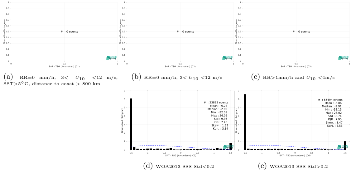
Figure 13: Normalized histogram of \Delta SSS (SMOS SSS L2Q v331 - No FLAG (CMEMS-CATDS-CPDC) - TSG (Amundsen)) for 5 different subdatasets corresponding to: RR=0 mm/h, 3 < U_{10} < 12 m/s, SST>5°C, distance to coast > 800 km (a), RR=0 mm/h, 3 < U_{10} < 12 m/s (b), RR>1mm/h and U_{10} < 4 m/s (c), WOA2013 SSS Std<0.2 (d), WOA2013 SSS Std>0.2 (e).
