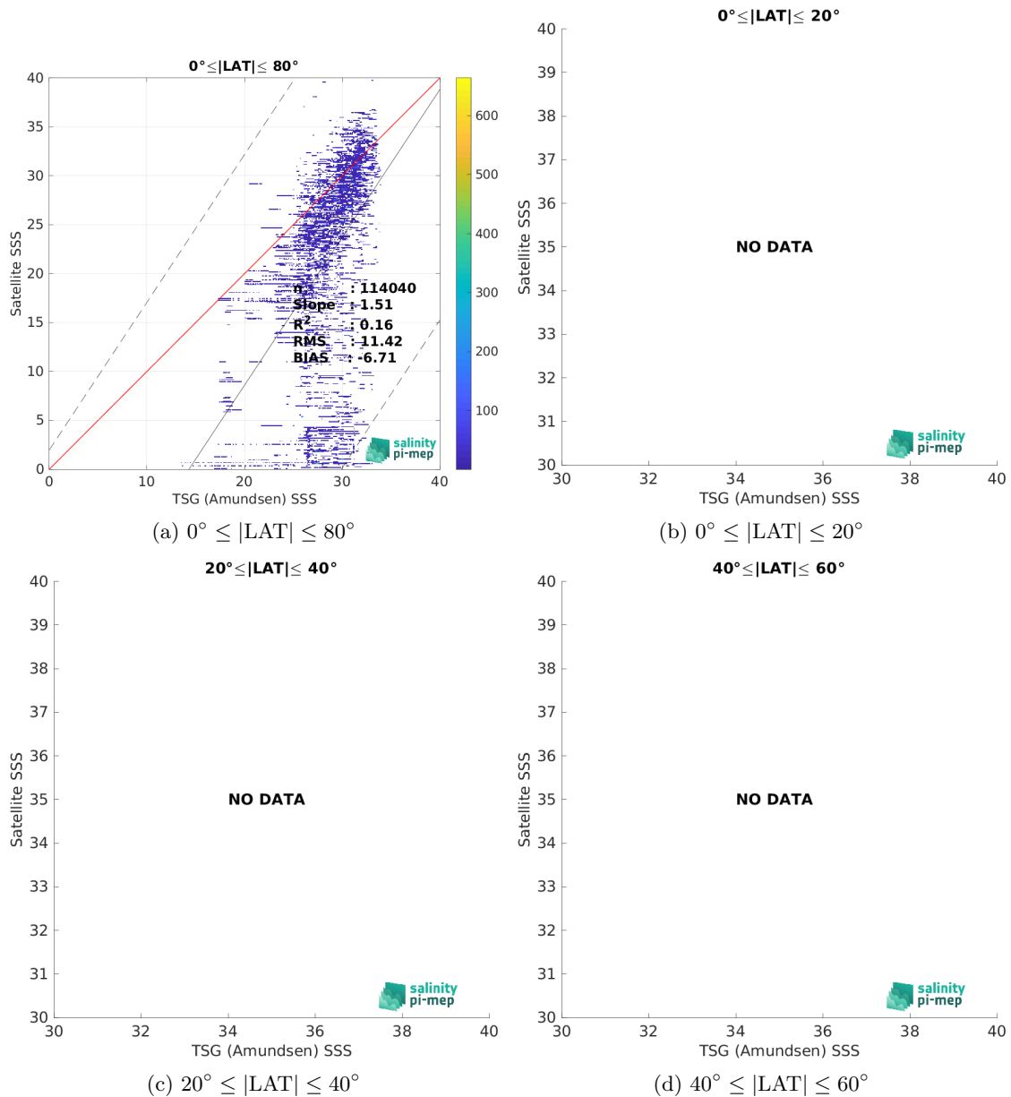
Figure 9: Contour maps of the concentration of SMOS SSS L2Q v331 - No FLAG (CMEMS-CATDS-CPDC) SSS (y-axis) versus TSG (Amundsen) SSS (x-axis) at match-up pairs for different latitude bands. For each plot, the red line shows x=y . The black thin and dashed lines indicate a linear fit through the data cloud and the \pm 95\% confidence levels, respectively. The number match-up pairs n , the slope and R^2 coefficient of the linear fit, the root mean square (RMS) and the mean bias between satellite and in situ data are indicated for each latitude band in each plots.
