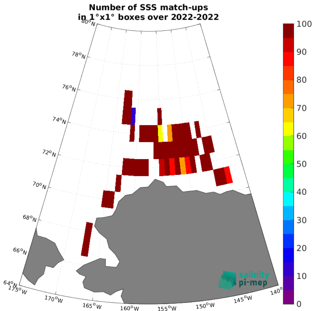
Figure 5: Number of SSS match-ups between SASSIE SSS and the SMOS SSS L2Q v331 - No FLAG (CMEMS-CATDS-CPDC) SSS product for the Arctic Ocean Pi-MEP region over 1^\circ \times 1^\circ boxes and for the full satellite product period.
