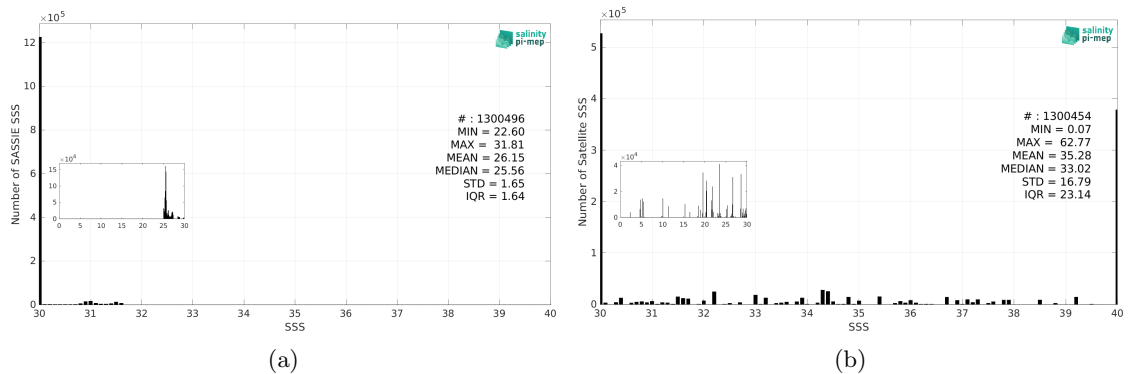
Figure 3: Histograms of SSS from SASSIE (a) and SMOS SSS L2Q v331 - No FLAG (CMEMS-CATDS-CPDC) (b) considering all match-up pairs per bins of 0.1 over the Arctic Ocean Pi-MEP region and for the full satellite product period.
