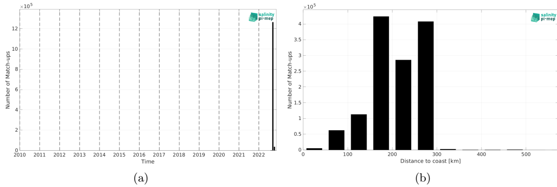
Figure 2: Number of match-ups between SASSIE and SMOS SSS L2Q v331 - No FLAG (CMEMS-CATDS-CPDC) SSS as a function of time (a) and as function of the distance to coast (b) over the Arctic Ocean Pi-MEP region and for the full satellite product period.
