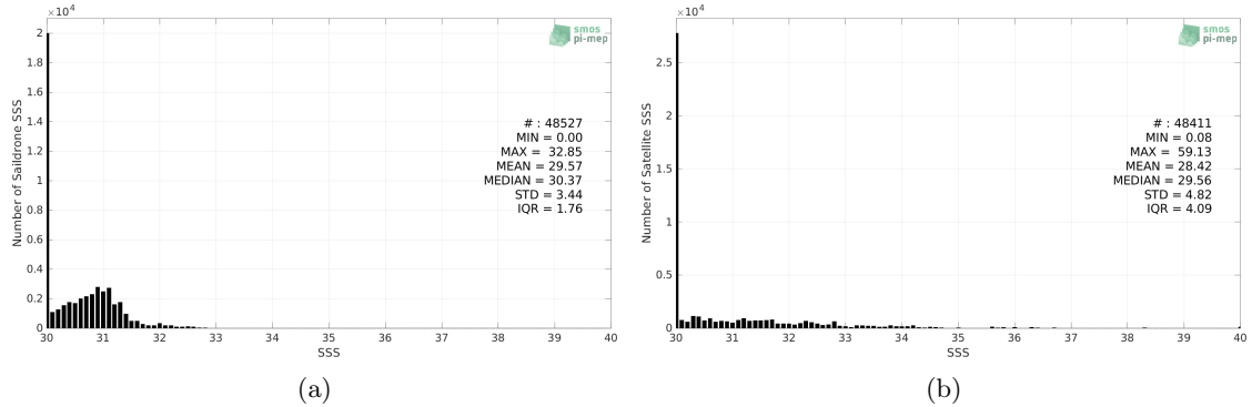
Figure 2: Histograms of SSS from Saildrone (a) and SMOS SSS L2Q v331 - No FLAG (CMEMS-CATDS-CPDC) (b) considering all match-up pairs per bins of 0.1 over the Arctic Ocean Pi-MEP region and for the full satellite product period.
