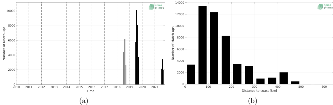
Figure 1: Number of match-ups between Saildrone and SMOS SSS L2Q v331 - No FLAG (CMEMS-CATDS-CPDC) SSS as a function of time (a) and as function of the distance to coast (b) over the Arctic Ocean Pi-MEP region and for the full satellite product period.
