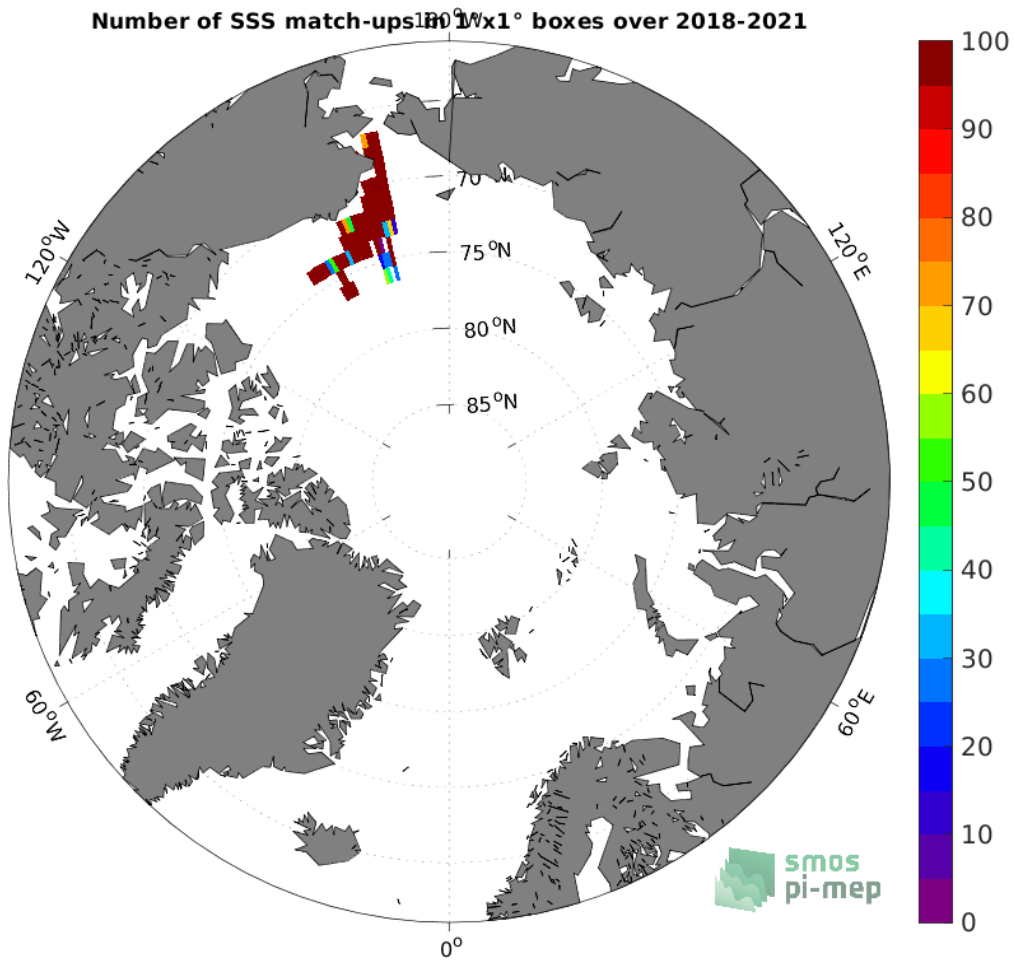
Figure 4: Number of SSS match-ups between Saifdrone SSS and the SMOS SSS L2Q v331 - No FLAG (CMEMS-CATDS-CPDC) SSS product for the Arctic Ocean Pi-MEP region over 1^\circ \times 1^\circ boxes and for the full satellite product period.
