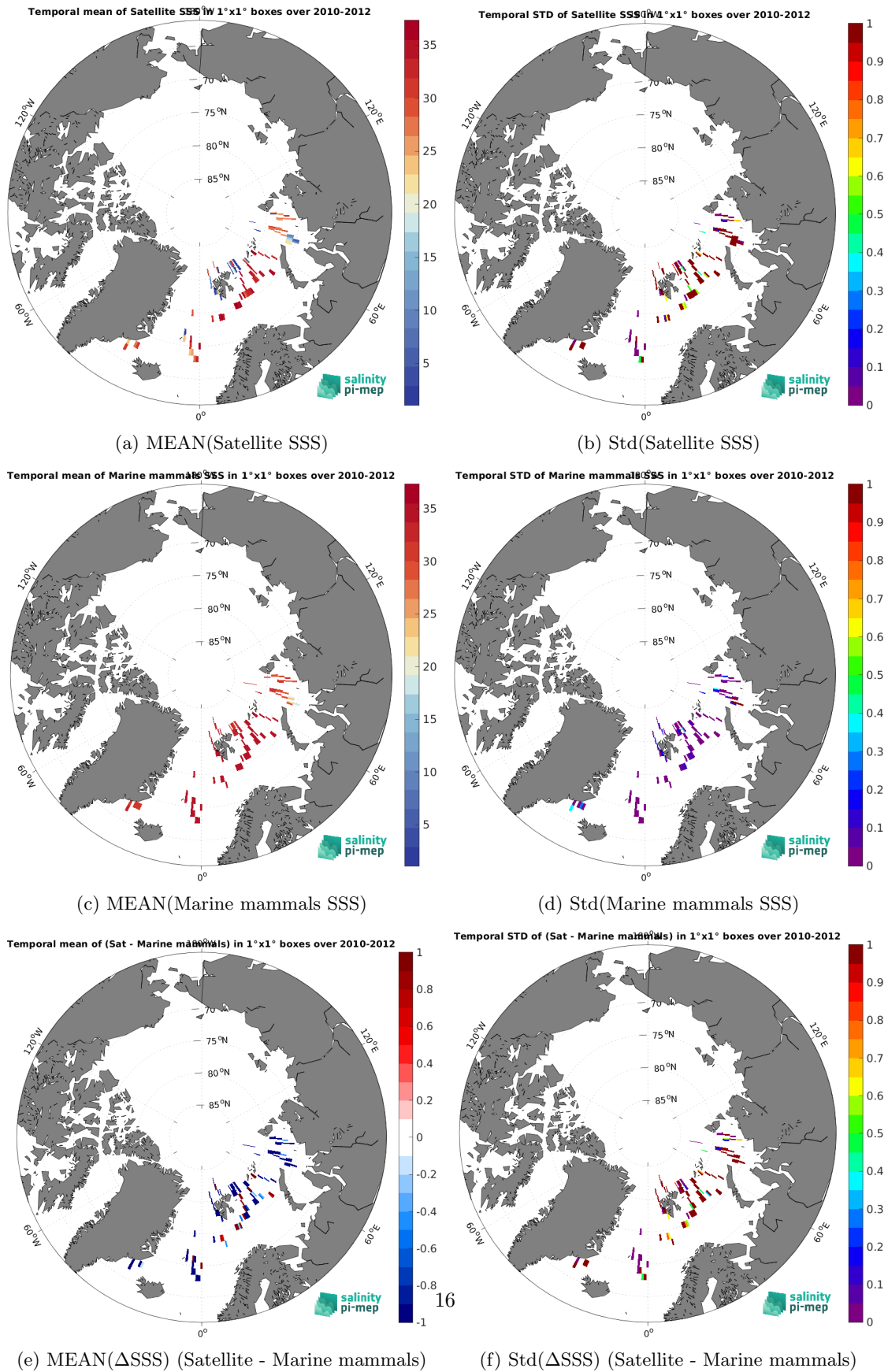
Figure 7: Temporal mean (left) and Std (right) of SSS from SMOS SSS L2Q v331 - No FLAG (CMEMS-CATDS-CPDC) (top), Marine mammals (middle), and of \Delta SSS (Satellite - Marine mammals). Only match-up pairs are used to generate these maps.
