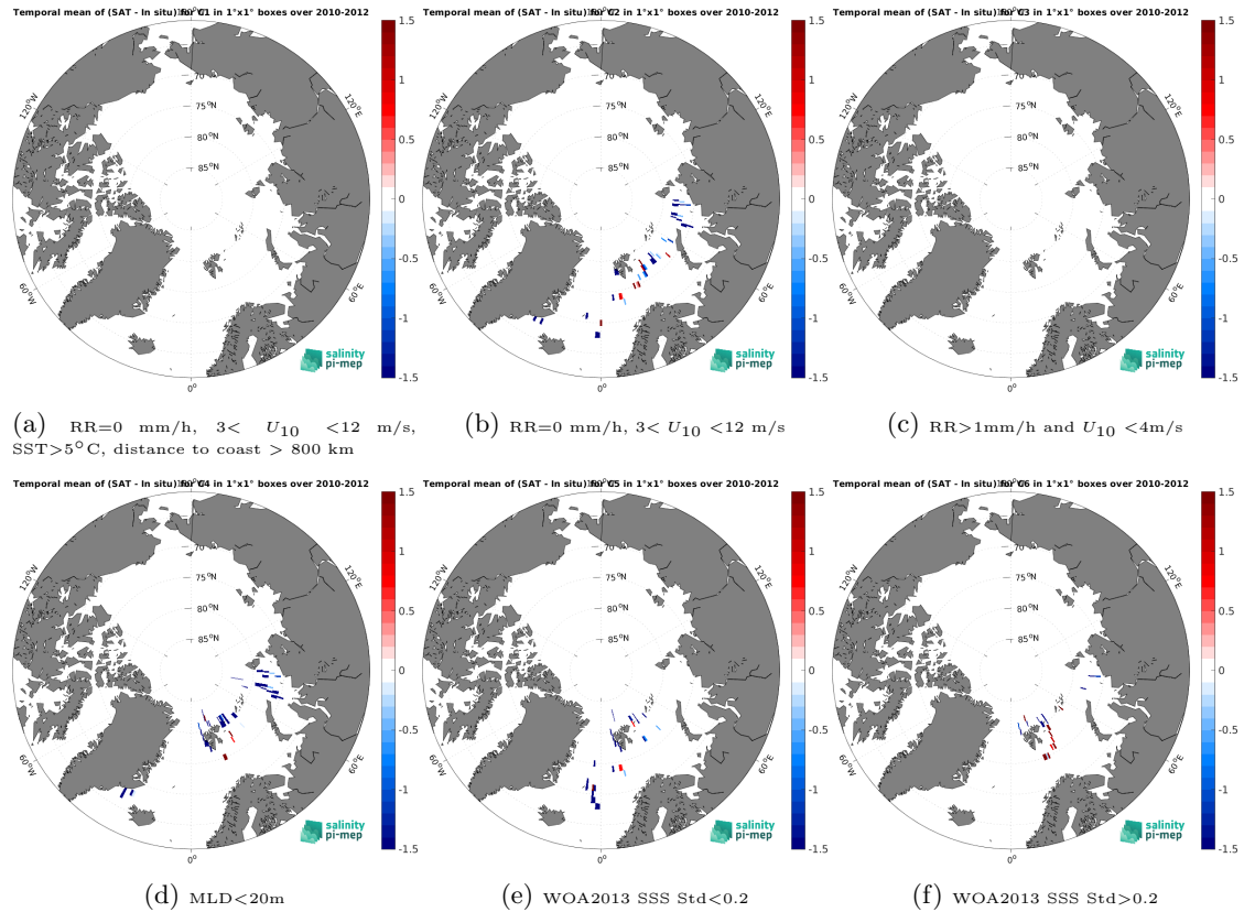
Figure 14: Temporal mean gridded over spatial boxes of size 1^\circ \times 1^\circ of \Delta SSS (SMOS SSS L2Q v331 - No FLAG (CMEMS-CATDS-CPDC) - Marine mammals) for 6 different subdatasets corresponding to:RR=0 mm/h, 3 < U_{10} < 12 m/s, SST >5^\circ C, distance to coast > 800 km (a), RR=0 mm/h, 3 < U_{10} < 12 m/s (b), RR >1 mm/h and U_{10} < 4 m/s (c),MLD <20 m (d),WOA2013 SSS Std <0.2 (e),WOA2013 SSS Std >0.2 (f).
