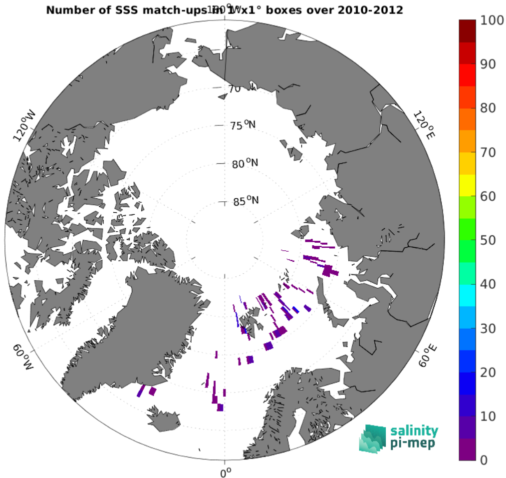
Figure 5: Number of SSS match-ups between Marine mammals SSS and the SMOS SSS L2Q v331 - No FLAG (CMEMS-CATDS-CPDC) SSS product for the Arctic Ocean Pi-MEP region over 1^\circ \times 1^\circ boxes and for the full satellite product period.
