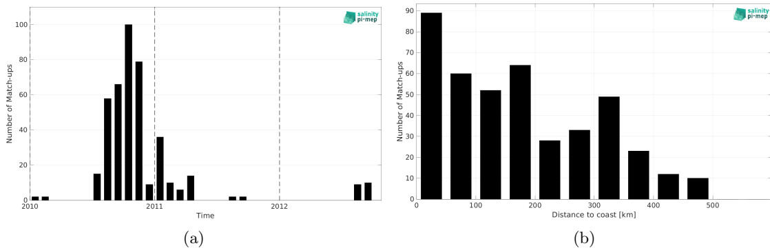
Figure 2: Number of match-ups between Marine mammals and SMOS SSS L2Q v331 - No FLAG (CMEMS-CATDS-CPDC) SSS as a function of time (a) and as function of the distance to coast (b) over the Arctic Ocean Pi-MEP region and for the full satellite product period.
