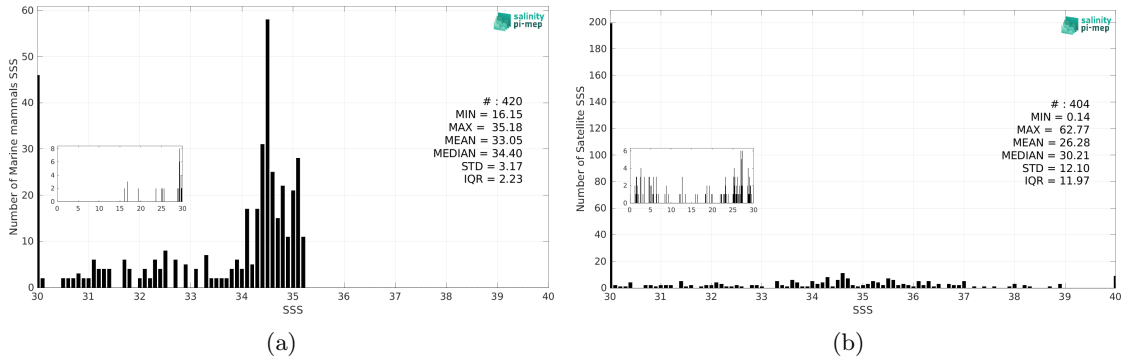
Figure 3: Histograms of SSS from Marine mammals (a) and SMOS SSS L2Q v331 - No FLAG (CMEMS-CATDS-CPDC) (b) considering all match-up pairs per bins of 0.1 over the Arctic Ocean Pi-MEP region and for the full satellite product period.
