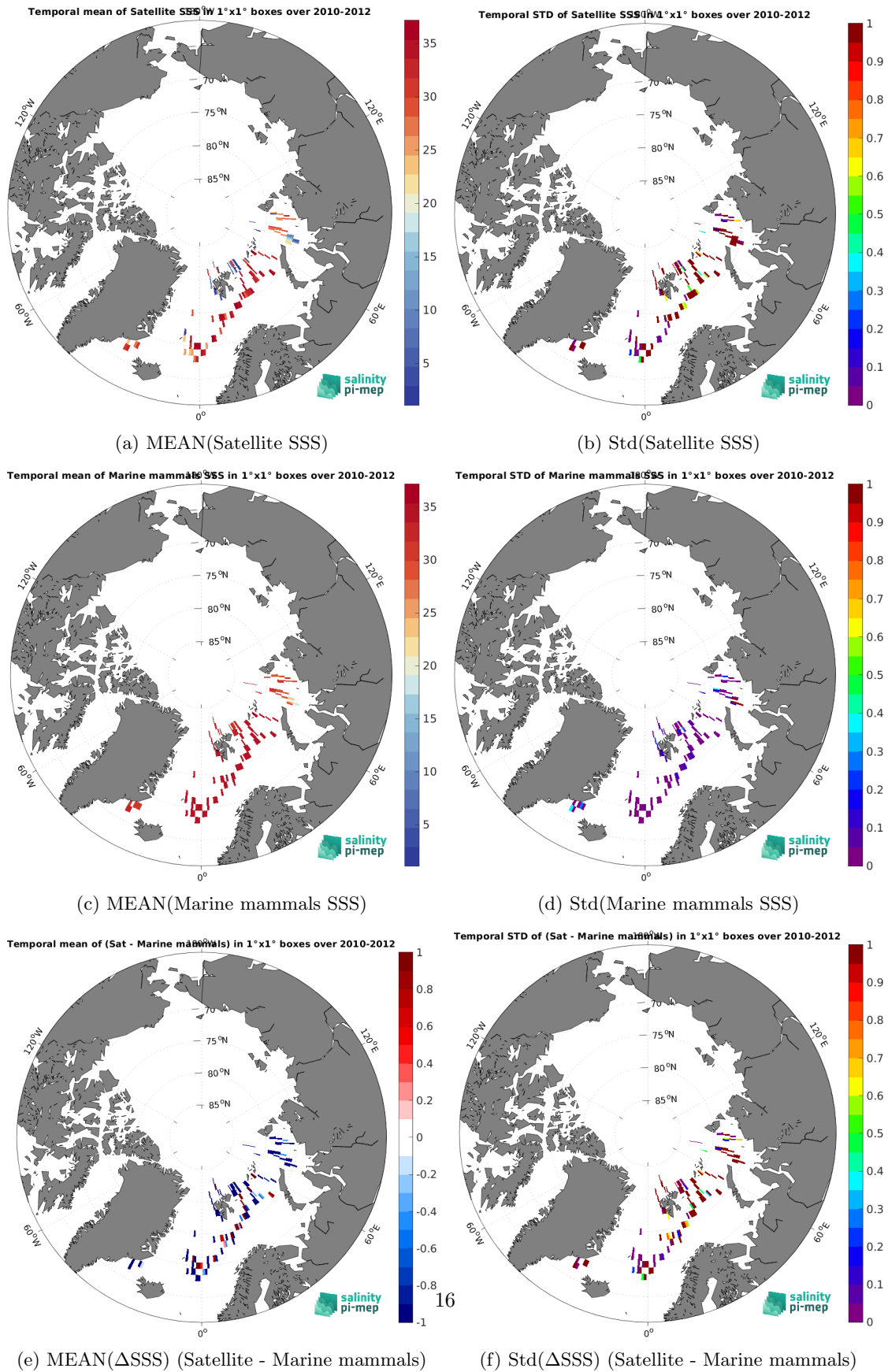
Figure 6: Temporal mean (left) and Std (right) of SSS from SMOS SSS L2Q v331 - No FLAG (CMEMS-CATDS-CPDC) (top), Marine mammals (middle), and of \Delta SSS (Satellite - Marine mammals). Only match-up pairs are used to generate these maps.
