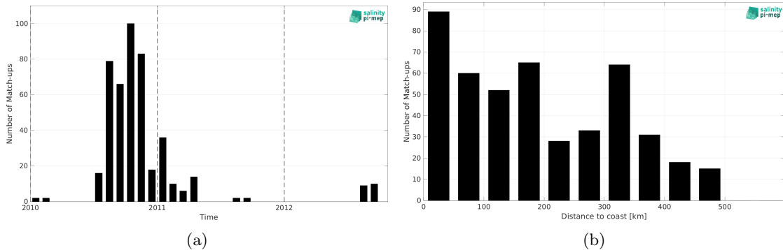
Figure 1: Number of match-ups between Marine mammals and SMOS SSS L2Q v331 - No FLAG (CMEMS-CATDS-CPDC) SSS as a function of time (a) and as function of the distance to coast (b) over the Arctic Ocean Pi-MEP region and for the full satellite product period.
