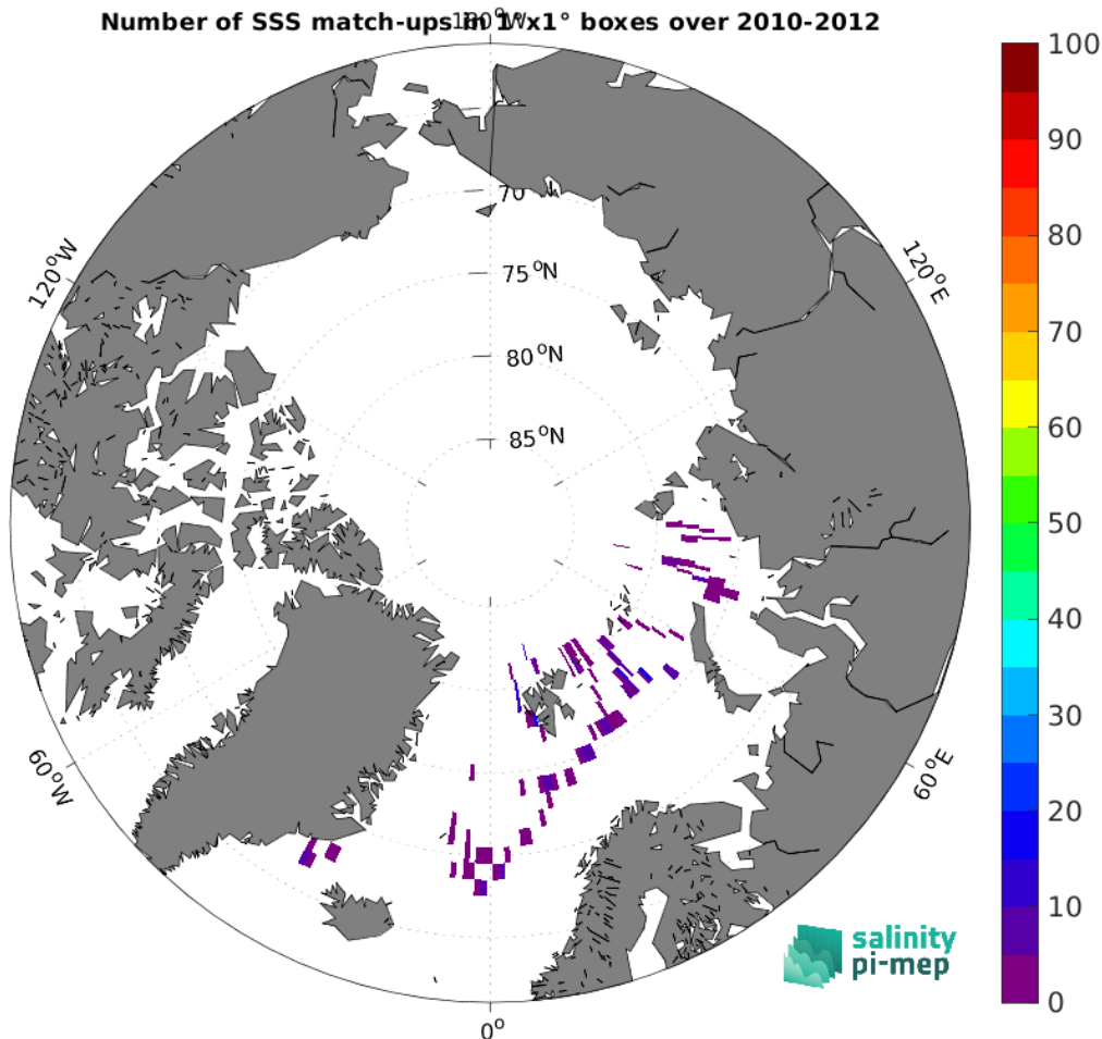
Figure 4: Number of SSS match-ups between Marine mammals SSS and the SMOS SSS L2Q v331 - No FLAG (CMEMS-CATDS-CPDC) SSS product for the Arctic Ocean Pi-MEP region over 1^\circ \times 1^\circ boxes and for the full satellite product period.
