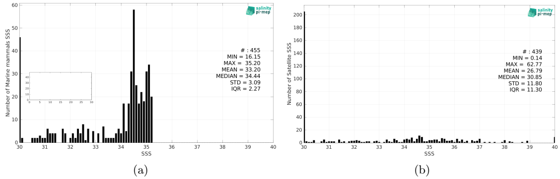
Figure 2: Histograms of SSS from Marine mammals (a) and SMOS SSS L2Q v331 - No FLAG (CMEMS-CATDS-CPDC) (b) considering all match-up pairs per bins of 0.1 over the Arctic Ocean Pi-MEP region and for the full satellite product period.
