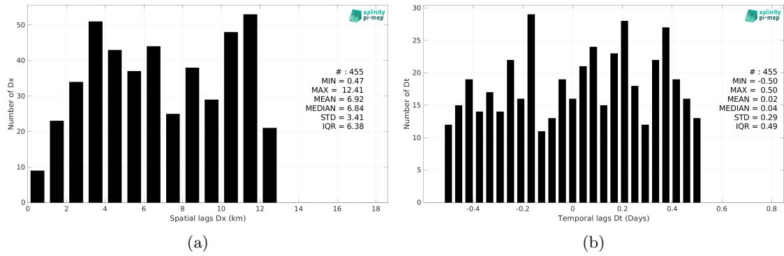
Figure 5: Histograms of the spatial (a) and temporal (b) lags between the location/time of the Marine mammals measurement and the date of the corresponding SMOS SSS L2Q v331 - No FLAG (CMEMS-CATDS-CPDC) SSS pixel.
