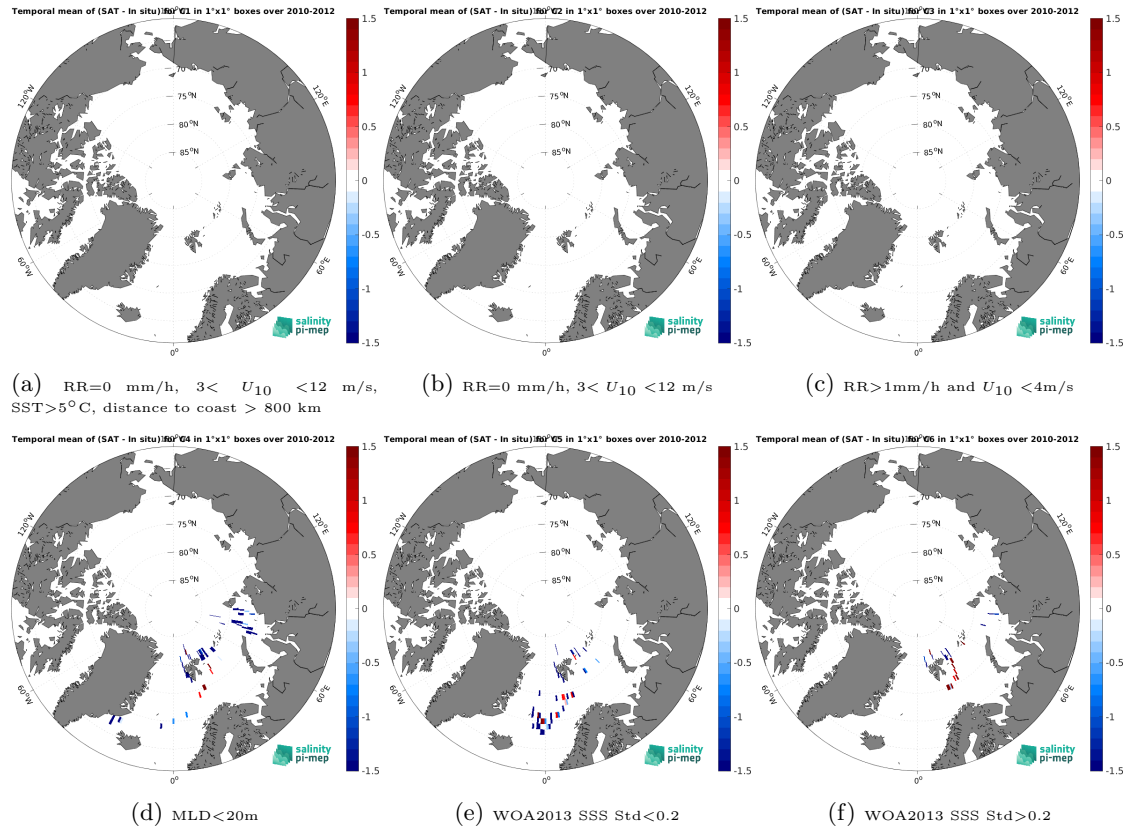
Figure 12: Temporal mean gridded over spatial boxes of size 1^{\circ}\times 1^{\circ} of \Delta\text{SSS} (SMOS SSS L2Q v331 - No FLAG (CMEMS-CATDS-CPDC) - Marine mammals) for 6 different subdatasets corresponding to:RR=0 mm/h, 3 < U_{10} < 12 m/s, SST >5^{\circ}\text{C} , distance to coast > 800 km (a), RR=0 mm/h, 3 < U_{10} < 12 m/s (b), RR >1 mm/h and U_{10} < 4 m/s (c),MLD <20 m (d),WOA2013 SSS Std <0.2 (e),WOA2013 SSS Std >0.2 (f).
