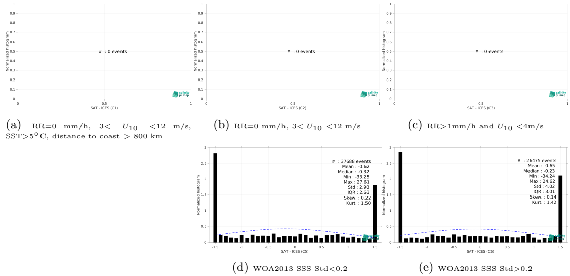
Figure 13: Normalized histogram of \Delta SSS (SMOS SSS L2Q v331 - No FLAG (CMEMS-CATDS-CPDC) - ICES) for 5 different subdatasets corresponding to: RR=0 mm/h, 3 < U_{10} < 12 m/s, SST > 5°C, distance to coast > 800 km (a), RR=0 mm/h, 3 < U_{10} < 12 m/s (b), RR > 1mm/h and U_{10} < 4 m/s (c), WOA2013 SSS Std < 0.2 (d), WOA2013 SSS Std > 0.2 (e).
