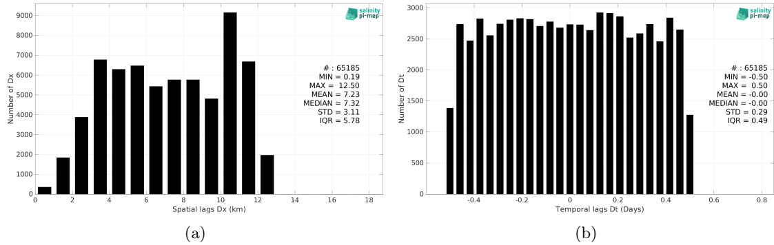
Figure 5: Histograms of the spatial (a) and temporal (b) lags between the location/time of the ICES measurement and the date of the corresponding SMOS SSS L2Q v331 - No FLAG (CMEMS-CATDS-CPDC) SSS pixel.
