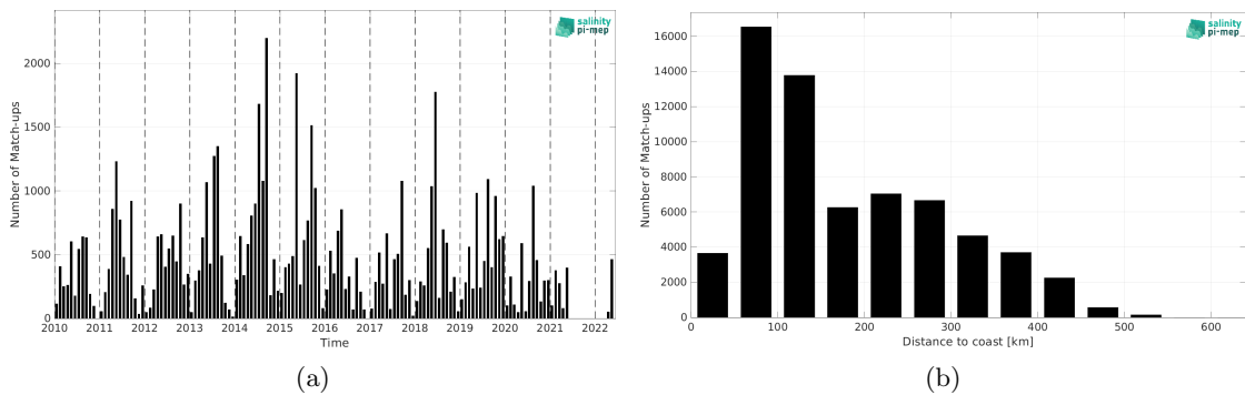
Figure 1: Number of match-ups between ICES and SMOS SSS L2Q v331 - No FLAG (CMEMS-CATDS-CPDC) SSS as a function of time (a) and as function of the distance to coast (b) over the Arctic Ocean Pi-MEP region and for the full satellite product period.
