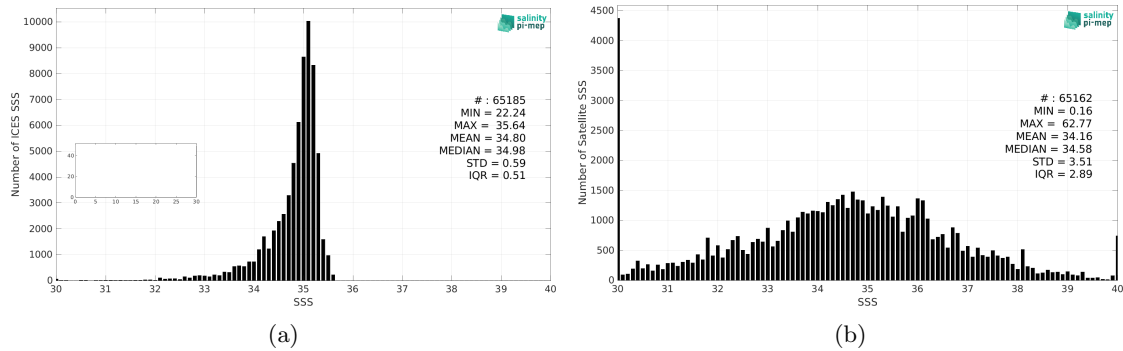
Figure 2: Histograms of SSS from ICES (a) and SMOS SSS L2Q v331 - No FLAG (CMEMS-CATDS-CPDC) (b) considering all match-up pairs per bins of 0.1 over the Arctic Ocean Pi-MEP region and for the full satellite product period.
