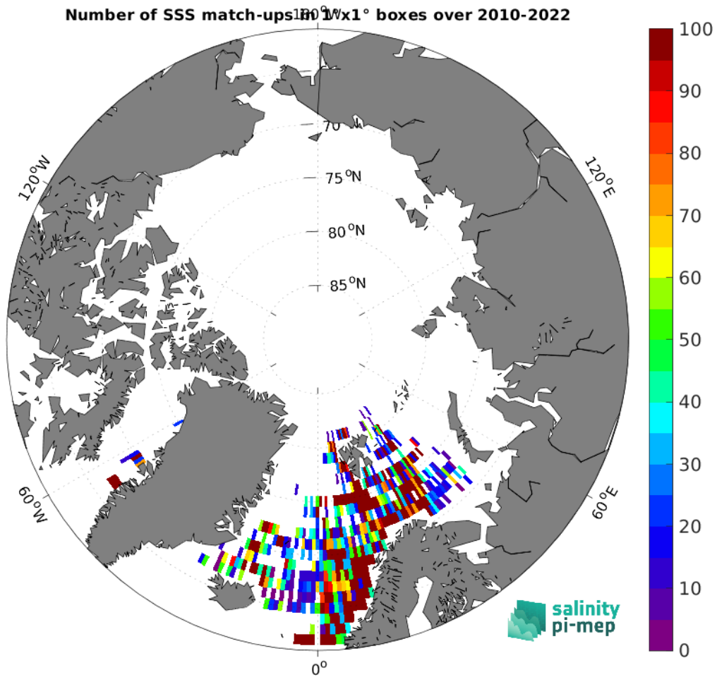
Figure 4: Number of SSS match-ups between ICES SSS and the SMOS SSS L2Q v331 - No FLAG (CMEMS-CATDS-CPDC) SSS product for the Arctic Ocean Pi-MEP region over 1^\circ \times 1^\circ boxes and for the full satellite product period.
