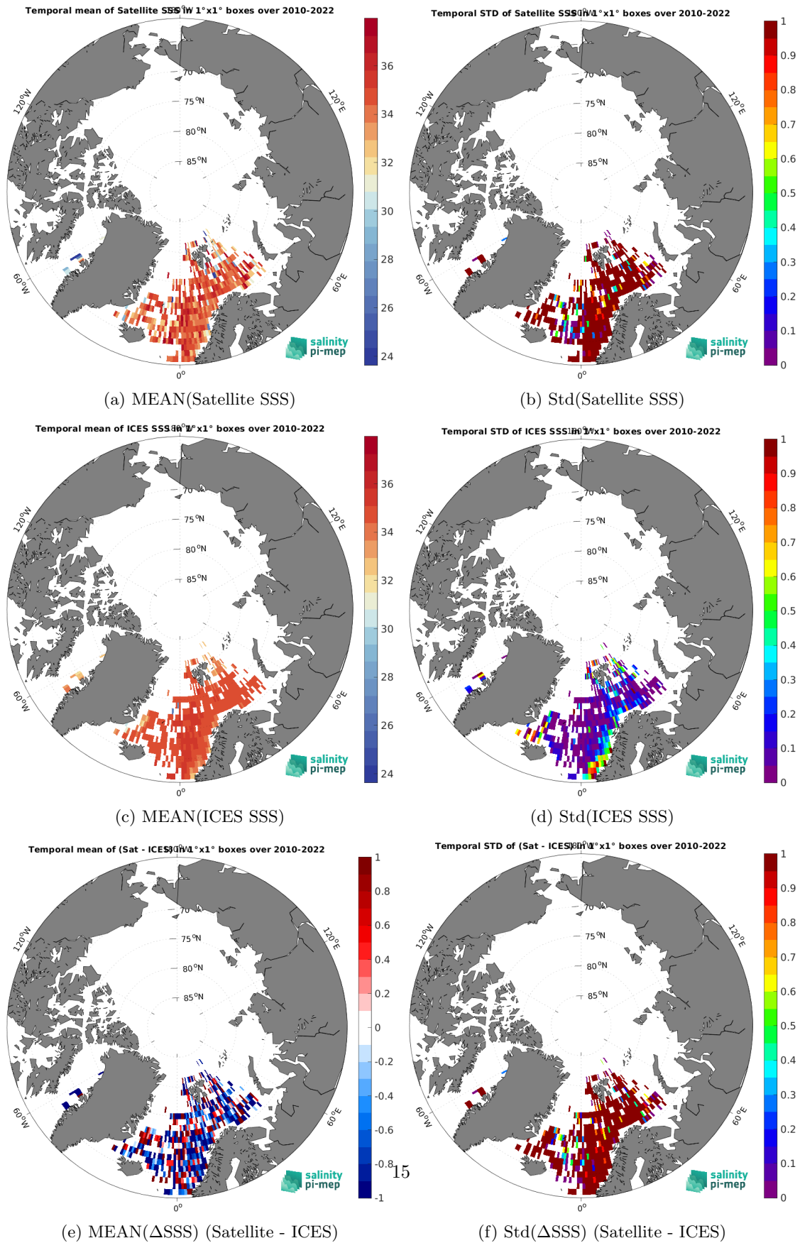
Figure 6: Temporal mean (left) and Std (right) of SSS from SMOS SSS L2Q v331 - No FLAG (CMEMS-CATDS-CPDC) (top), ICES (middle), and of \Delta SSS (Satellite - ICES). Only match-up pairs are used to generate these maps.
