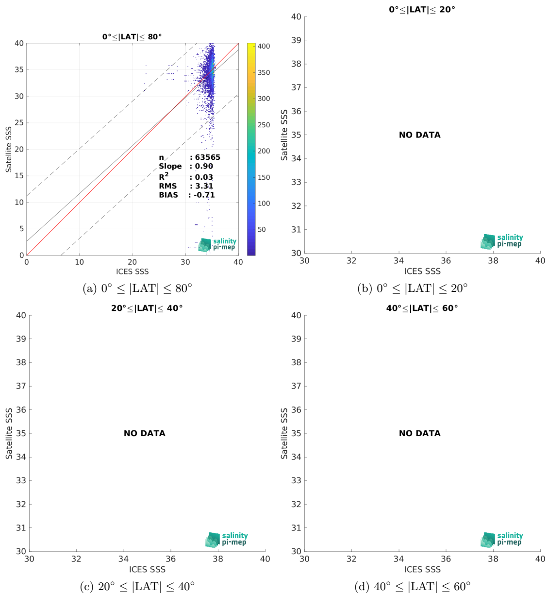
Figure 9: Contour maps of the concentration of SMOS SSS L2Q v331 - No FLAG (CMEMS-CATDS-CPDC) SSS (y-axis) versus ICES SSS (x-axis) at match-up pairs for different latitude bands. For each plot, the red line shows x=y . The black thin and dashed lines indicate a linear fit through the data cloud and the \pm 95\% confidence levels, respectively. The number match-up pairs n , the slope and R^2 coefficient of the linear fit, the root mean square (RMS) and the mean bias between satellite and in situ data are indicated for each latitude band in each plots.
