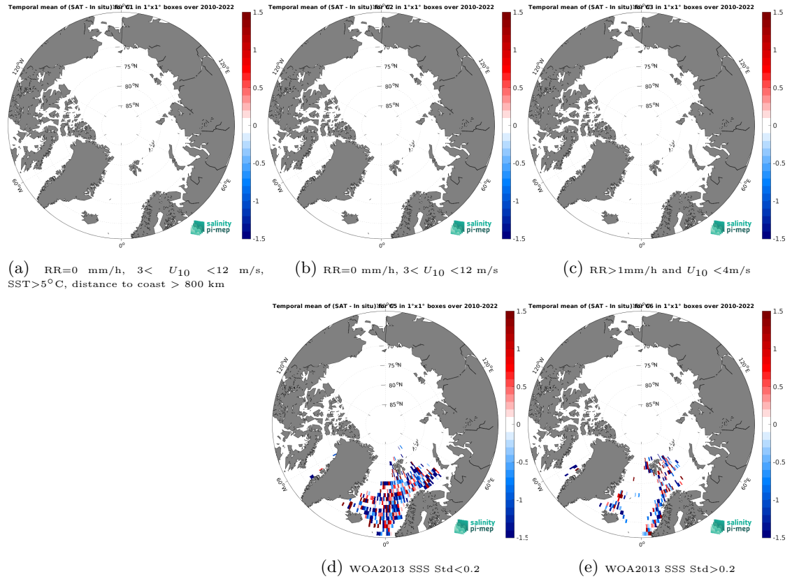
Figure 12: Temporal mean gridded over spatial boxes of size 1^{\circ}\times 1^{\circ} of \Delta\text{SSS} (SMOS SSS L2Q v331 - No FLAG (CMEMS-CATDS-CPDC) - ICES) for 5 different subdatasets corresponding to: RR=0 mm/h, 3 < U_{10} < 12 m/s, SST > 5^{\circ}\text{C} , distance to coast > 800 km (a), RR=0 mm/h, 3 < U_{10} < 12 m/s (b), RR > 1 mm/h and U_{10} < 4 m/s (c), WOA2013 SSS Std < 0.2 (d), WOA2013 SSS Std > 0.2 (e).
