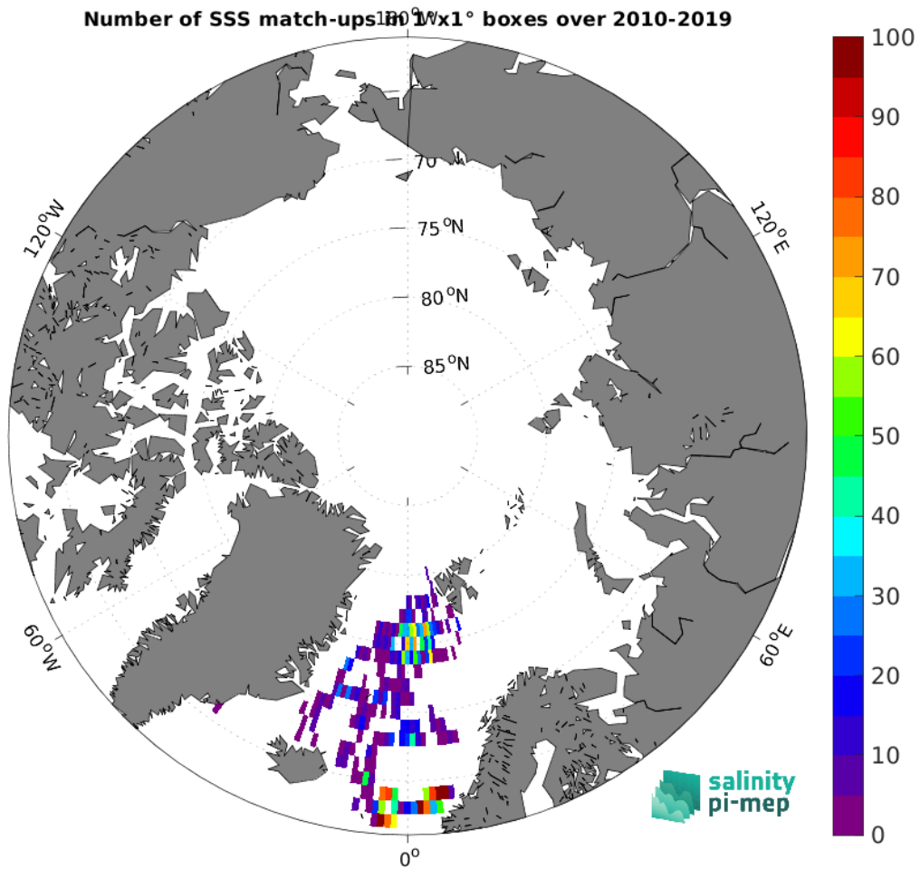
Figure 3: Number of SSS match-ups between Surface drifters SSS and the SMOS SSS L2Q v331 - No FLAG (CMEMS-CATDS-CPDC) SSS product for the Arctic Ocean Pi-MEP region over 1^\circ \times 1^\circ boxes and for the full satellite product period.
