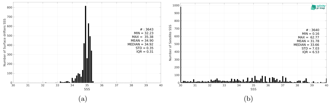
Figure 2: Histograms of SSS from Surface drifters (a) and SMOS SSS L2Q v331 - No FLAG (CMEMS-CATDS-CPDC) (b) considering all match-up pairs per bins of 0.1 over the Arctic Ocean Pi-MEP region and for the full satellite product period.
