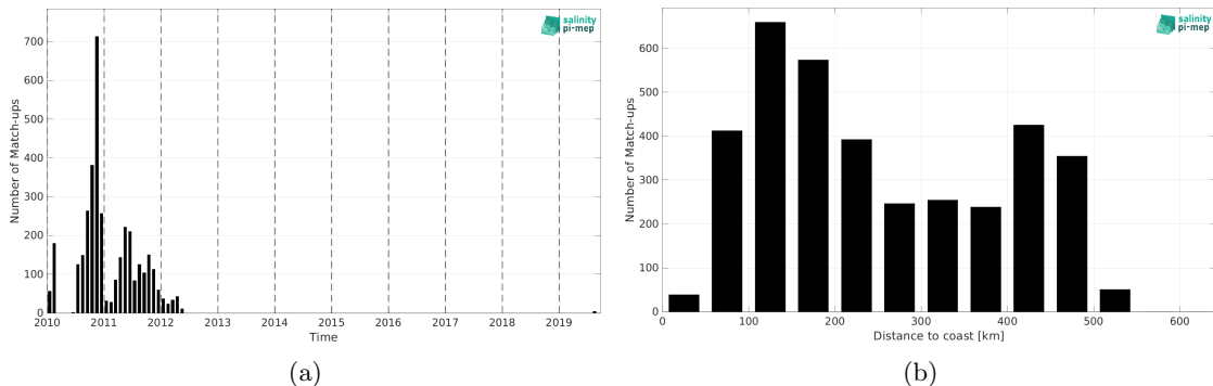
Figure 1: Number of match-ups between Surface drifters and SMOS SSS L2Q v331 - No FLAG (CMEMS-CATDS-CPDC) SSS as a function of time (a) and as function of the distance to coast (b) over the Arctic Ocean Pi-MEP region and for the full satellite product period.
