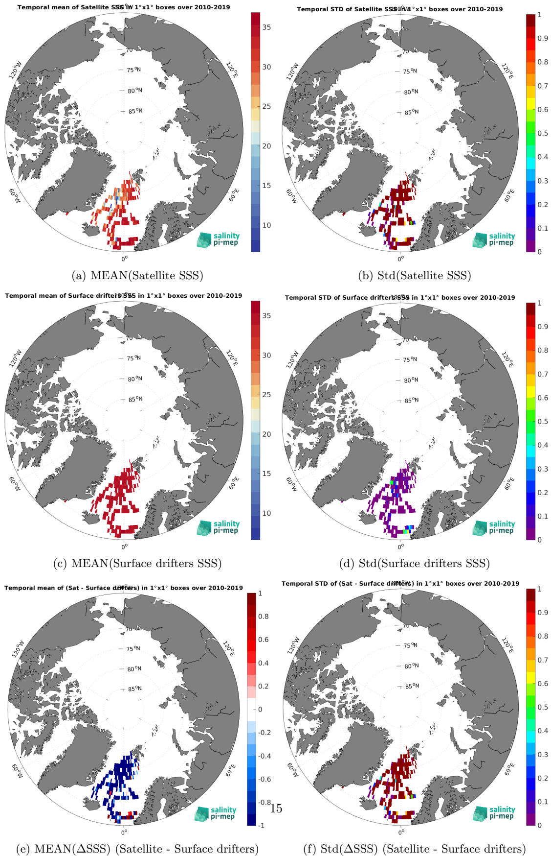
Figure 5: Temporal mean (left) and Std (right) of SSS from SMOS SSS L2Q v331 - No FLAG (CMEMS-CATDS-CPDC) (top), Surface drifters (middle), and of \Delta SSS (Satellite - Surface drifters). Only match-up pairs are used to generate these maps.
