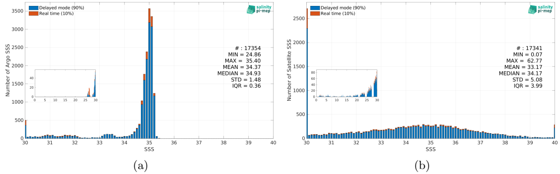
Figure 3: Histograms of SSS from Argo (a) and SMOS SSS L2Q v331 - No FLAG (CMEMS-CATDS-CPDC) (b) considering all match-up pairs per bins of 0.1 over the Arctic Ocean Pi-MEP region and for the full satellite product period.
