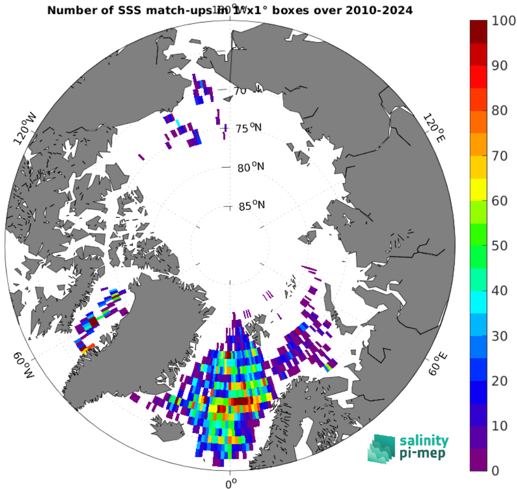
Figure 5: Number of SSS match-ups between Argo SSS and the SMOS SSS L2Q v331 - No FLAG (CMEMS-CATDS-CPDC) SSS product for the Arctic Ocean Pi-MEP region over 1^\circ \times 1^\circ boxes and for the full satellite product period.
