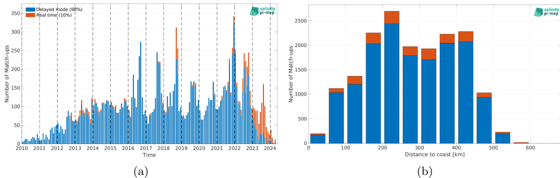
Figure 2: Number of match-ups between Argo and SMOS SSS L2Q v331 - No FLAG (CMEMS-CATDS-CPDC) SSS as a function of time (a) and as function of the distance to coast (b) over the Arctic Ocean Pi-MEP region and for the full satellite product period.
