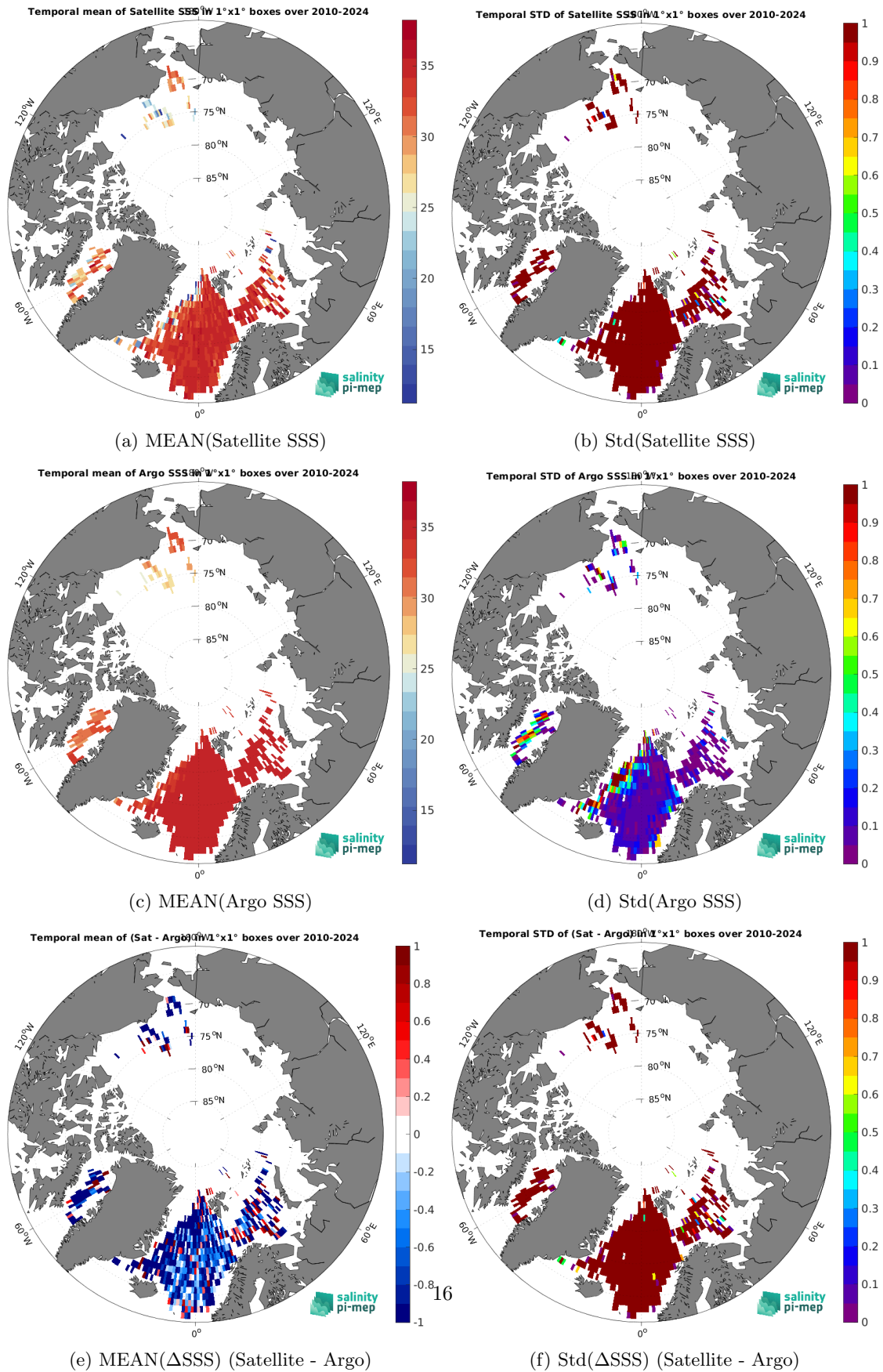
Figure 7: Temporal mean (left) and Std (right) of SSS from SMOS SSS L2Q v331 - No FLAG (CMEMS-CATDS-CPDC) (top), Argo (middle), and of \Delta SSS (Satellite - Argo). Only match-up pairs are used to generate these maps.
