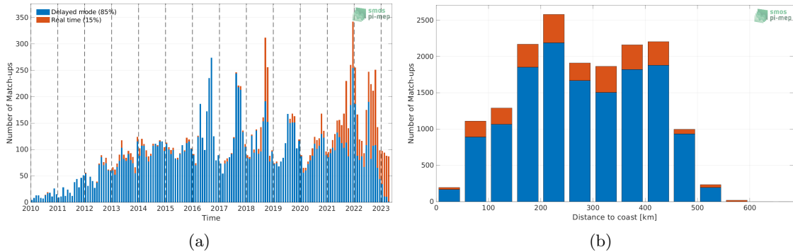
Figure 1: Number of match-ups between Argo and SMOS SSS L2Q v331 - No FLAG (CMEMS-CATDS-CPDC) SSS as a function of time (a) and as function of the distance to coast (b) over the Arctic Ocean Pi-MEP region and for the full satellite product period.
