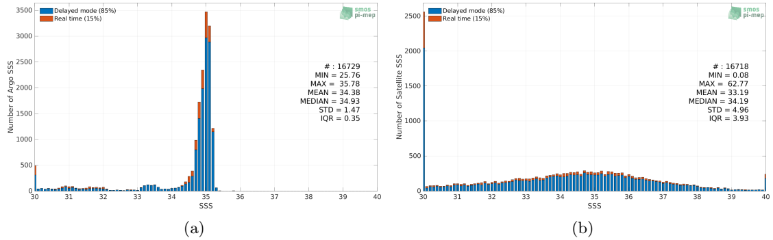
Figure 2: Histograms of SSS from Argo (a) and SMOS SSS L2Q v331 - No FLAG (CMEMS-CATDS-CPDC) (b) considering all match-up pairs per bins of 0.1 over the Arctic Ocean Pi-MEP region and for the full satellite product period.
