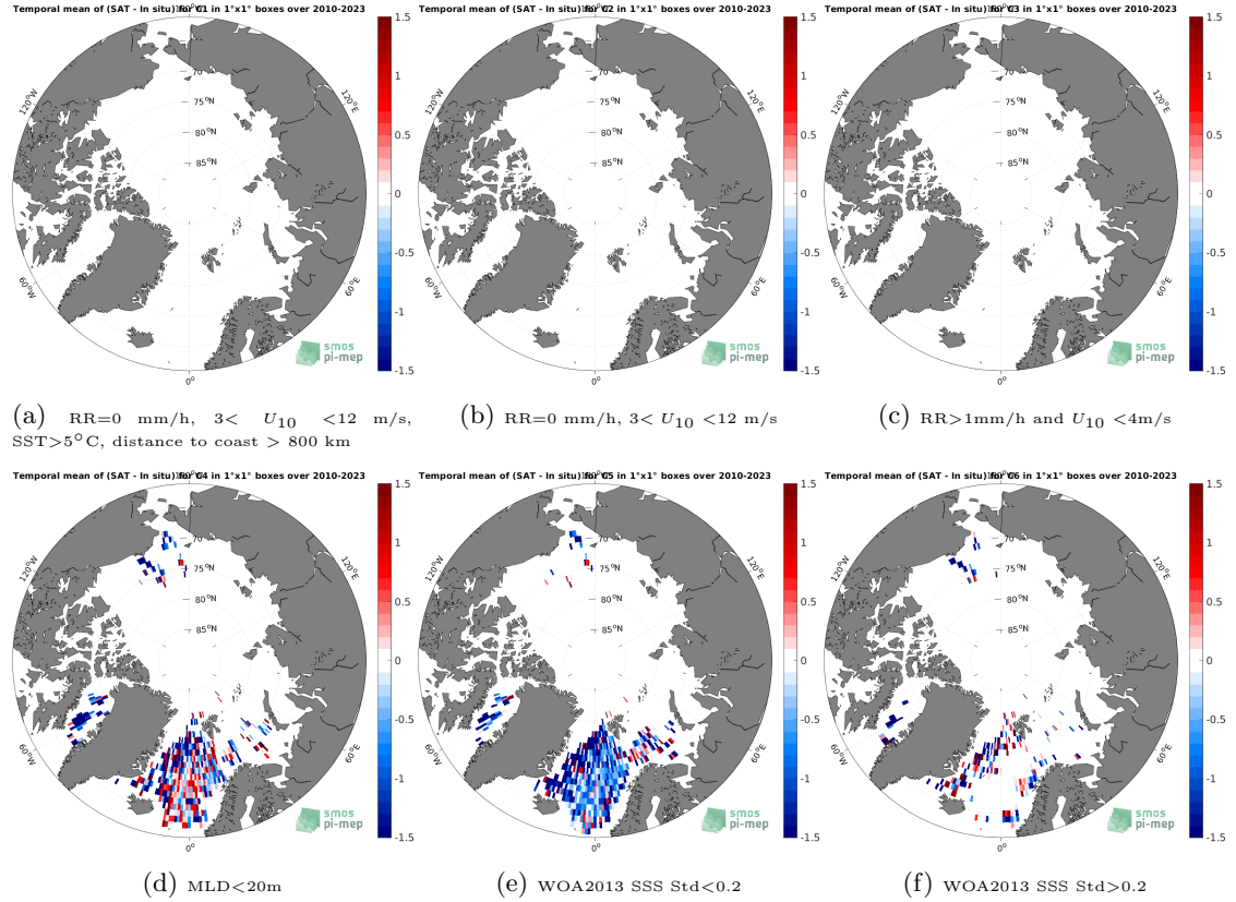
Figure 12: Temporal mean gridded over spatial boxes of size 1^{\circ}\times 1^{\circ} of \Delta\text{SSS} (SMOS SSS L2Q v331 - No FLAG (CMEMS-CATDS-CPDC) - Argo) for 6 different subdatasets corresponding to:RR=0 mm/h, 3 < U_{10} < 12 m/s, SST >5^{\circ}\text{C} , distance to coast > 800 km (a), RR=0 mm/h, 3 < U_{10} < 12 m/s (b), RR >1 mm/h and U_{10} < 4 m/s (c),MLD <20 m (d),WOA2013 SSS Std <0.2 (e),WOA2013 SSS Std >0.2 (f).
