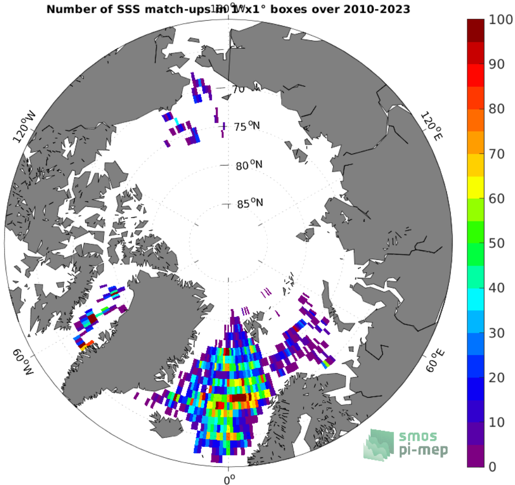
Figure 4: Number of SSS match-ups between Argo SSS and the SMOS SSS L2Q v331 - No FLAG (CMEMS-CATDS-CPDC) SSS product for the Arctic Ocean Pi-MEP region over 1^\circ \times 1^\circ boxes and for the full satellite product period.
