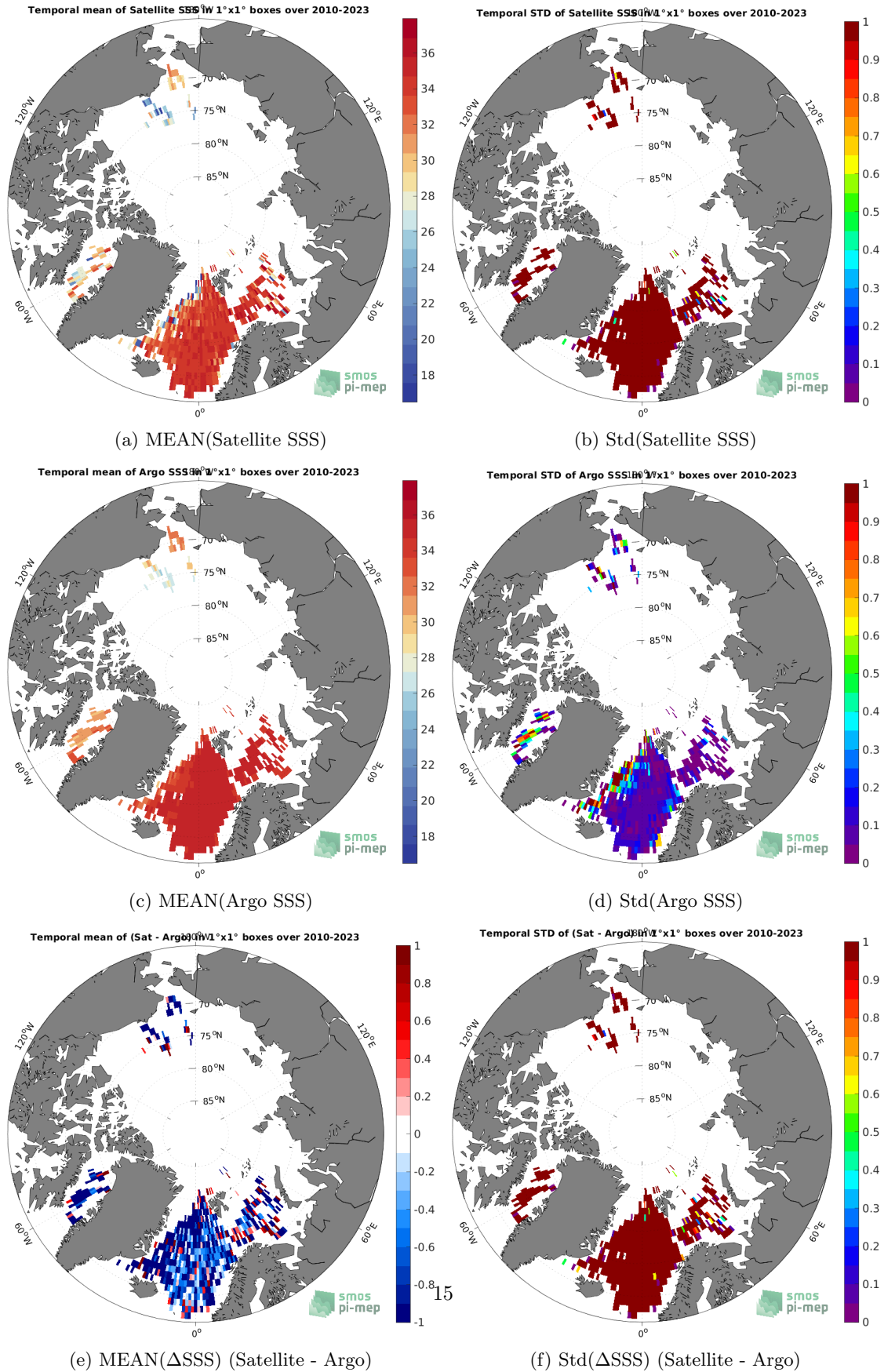
Figure 6: Temporal mean (left) and Std (right) of SSS from SMOS SSS L2Q v331 - No FLAG (CMEMS-CATDS-CPDC) (top), Argo (middle), and of \Delta SSS (Satellite - Argo). Only match-up pairs are used to generate these maps.
