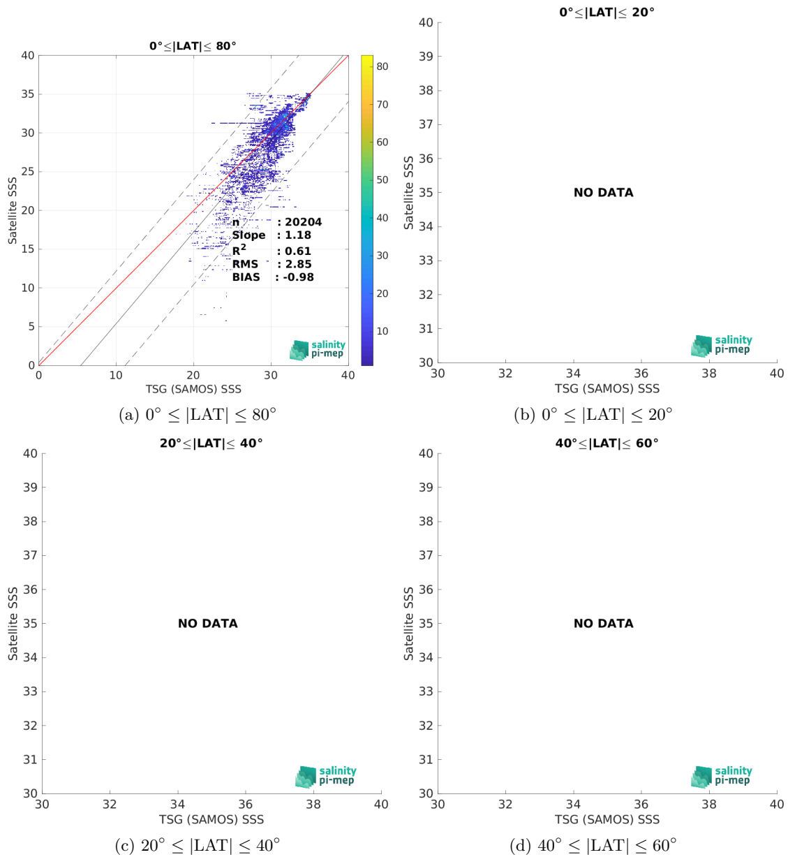
Figure 10: Contour maps of the concentration of SMOS SSS L3 v9 - 9 Days (CATDS-CEC-LOCEAN) SSS ( y -axis) versus TSG (SAMOS) SSS ( x -axis) at match-up pairs for different latitude bands. For each plot, the red line shows x=y . The black thin and dashed lines indicate a linear fit through the data cloud and the \pm 95\% confidence levels, respectively. The number match-up pairs n , the slope and R^2 coefficient of the linear fit, the root mean square (RMS) and the mean bias between satellite and in situ data are indicated for each latitude band in each plots.
