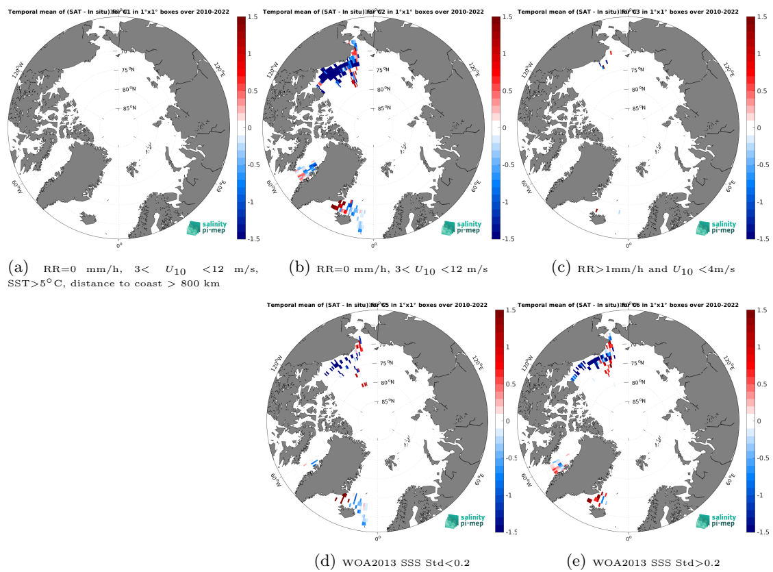
Figure 14: Temporal mean gridded over spatial boxes of size 1^\circ \times 1^\circ of \Delta SSS (SMOS SSS L3 v9 - 9 Days (CATDS-CEC-LOCEAN) - TSG (SAMOS)) for 5 different subdatasets corresponding to: RR=0 mm/h, 3 < U_{10} < 12 m/s, SST > 5^\circ\text{C} , distance to coast > 800 km (a), RR=0 mm/h, 3 < U_{10} < 12 m/s (b), RR > 1 mm/h and U_{10} < 4 m/s (c), WOA2013 SSS Std < 0.2 (d), WOA2013 SSS Std > 0.2 (e).
