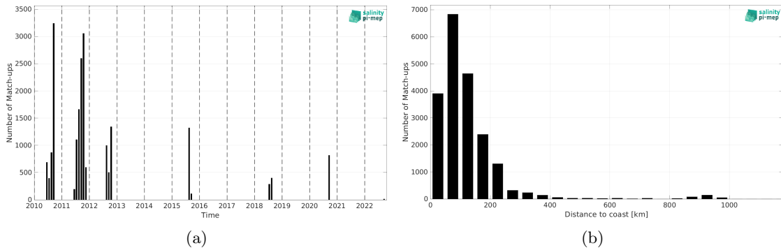
Figure 2: Number of match-ups between TSG (SAMOS) and SMOS SSS L3 v9 - 9 Days (CATDS-CEC-LOCEAN) SSS as a function of time (a) and as function of the distance to coast (b) over the Arctic Ocean Pi-MEP region and for the full satellite product period.
