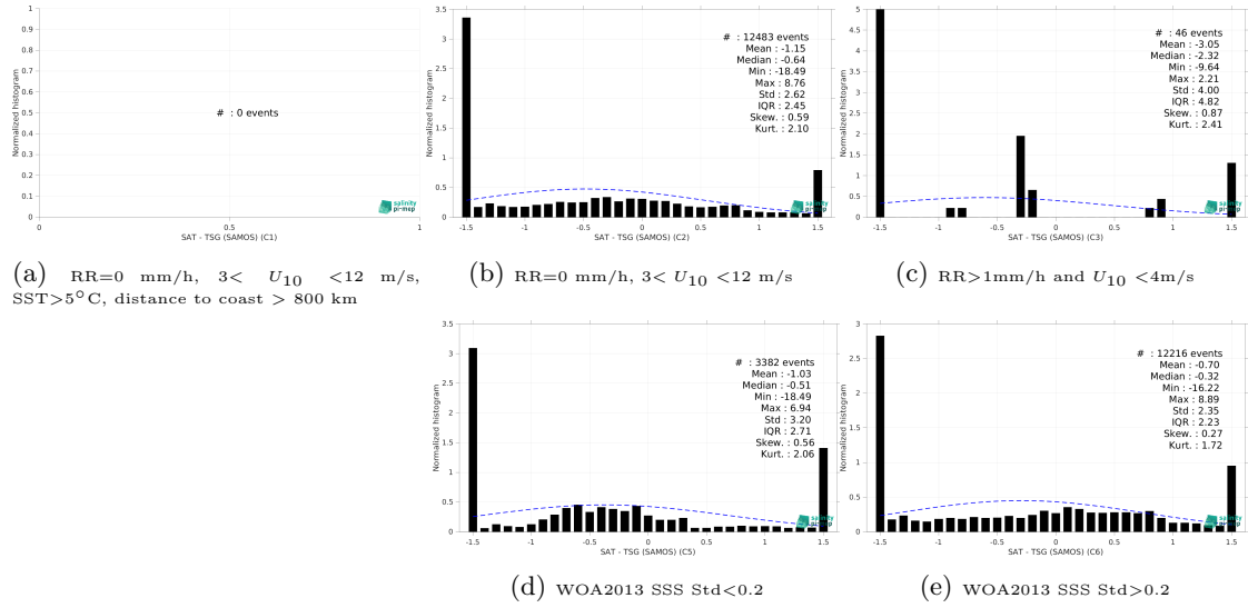
Figure 15: Normalized histogram of \Delta SSS (SMOS SSS L3 v9 - 9 Days (CATDS-CEC-LOCEAN) - TSG (SAMOS)) for 5 different subdatasets corresponding to: RR=0 mm/h, 3 < U_{10} < 12 m/s, SST > 5°C, distance to coast > 800 km (a), RR=0 mm/h, 3 < U_{10} < 12 m/s (b), RR > 1mm/h and U_{10} < 4 m/s (c), WOA2013 SSS Std < 0.2 (d), WOA2013 SSS Std > 0.2 (e).
