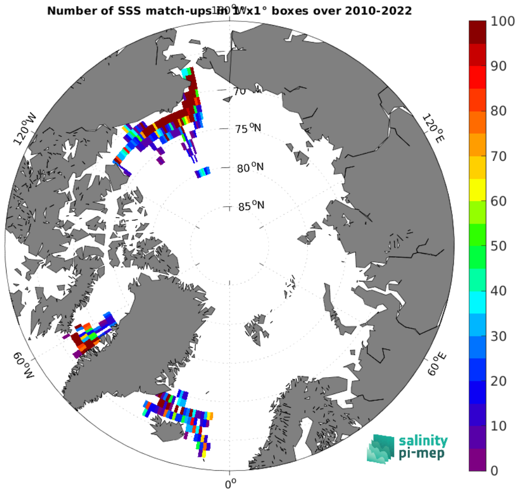
Figure 5: Number of SSS match-ups between TSG (SAMOS) SSS and the SMOS SSS L3 v9 - 9 Days (CATDS-CEC-LOCEAN) SSS product for the Arctic Ocean Pi-MEP region over 1^\circ \times 1^\circ boxes and for the full satellite product period.
