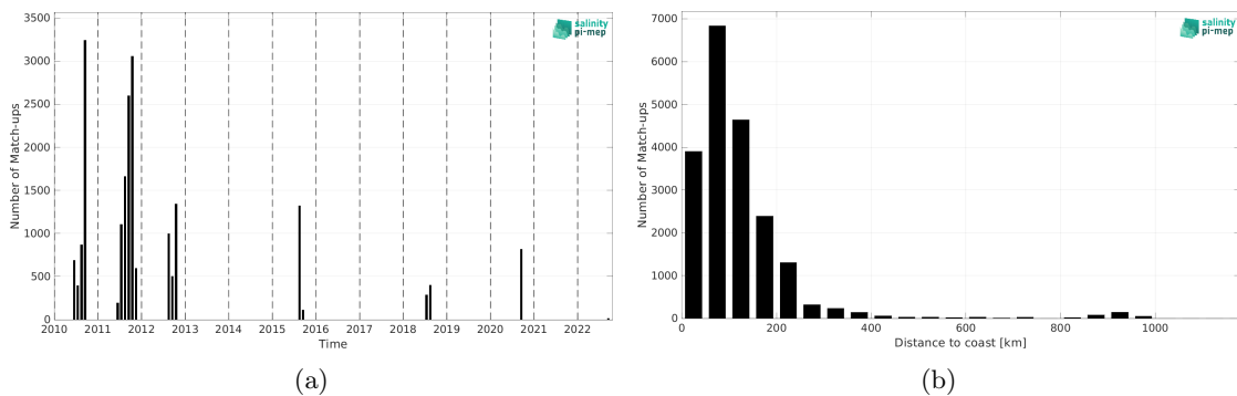
Figure 1: Number of match-ups between TSG (SAMOS) and SMOS SSS L3 v9 - 9 Days (CATDS-CEC-LOCEAN) SSS as a function of time (a) and as function of the distance to coast (b) over the Arctic Ocean Pi-MEP region and for the full satellite product period.
