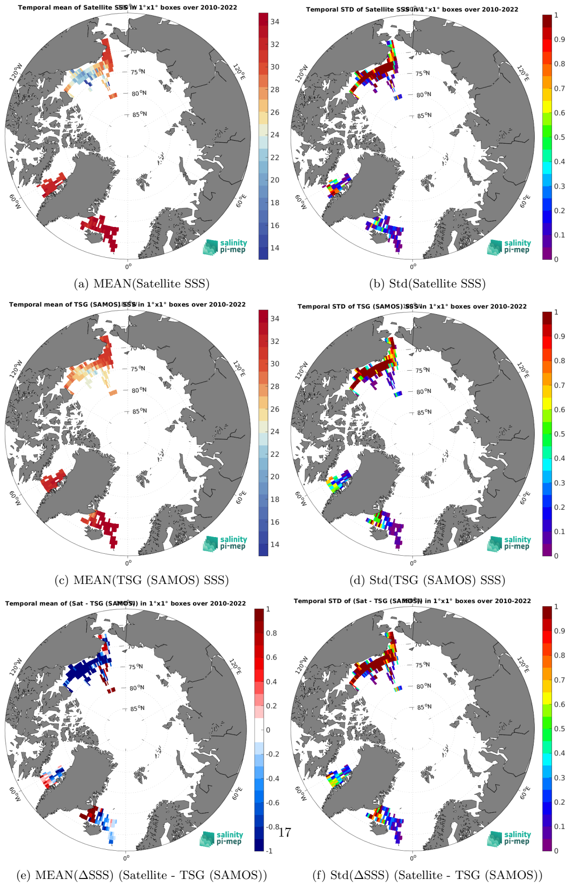
Figure 6: Temporal mean (left) and Std (right) of SSS from SMOS SSS L3 v9 - 9 Days (CATDS-CEC-LOCEAN) (top), TSG (SAMOS) (middle), and of \Delta SSS (Satellite - TSG (SAMOS)). Only match-up pairs are used to generate these maps.
