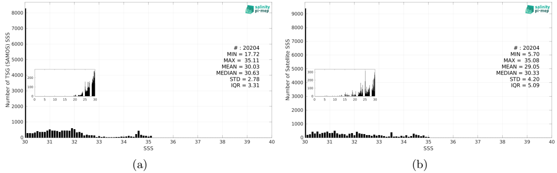
Figure 2: Histograms of SSS from TSG (SAMOS) (a) and SMOS SSS L3 v9 - 9 Days (CATDS-CEC-LOCEAN) (b) considering all match-up pairs per bins of 0.1 over the Arctic Ocean Pi-MEP region and for the full satellite product period.
