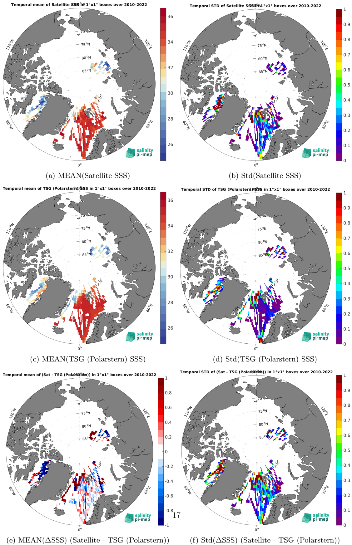
Figure 7: Temporal mean (left) and Std (right) of SSS from SMOS SSS L3 v9 - 9 Days (CATDS-CEC-LOCEAN) (top), TSG (Polarstern) (middle), and of \Delta SSS (Satellite - TSG (Polarstern)). Only match-up pairs are used to generate these maps.
