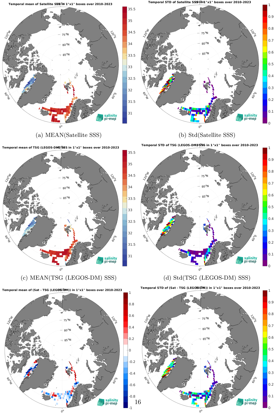
(e) MEAN( \Delta SSS) (Satellite - TSG (LEGOS-DM)) (f) Std( \Delta SSS) (Satellite - TSG (LEGOS-DM)) Figure 7: Temporal mean (left) and Std (right) of SSS from SMOS SSS L3 v9 - 9 Days (CATDS-CEC-LOCEAN) (top), TSG (LEGOS-DM) (middle), and of \Delta SSS (Satellite - TSG (LEGOS-DM)). Only match-up pairs are used to generate these maps.
