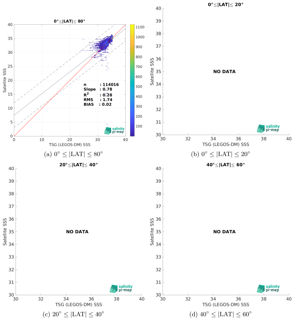
Figure 10: Contour maps of the concentration of SMOS SSS L3 v9 - 9 Days (CATDS-CEC-LOCEAN) SSS (y-axis) versus TSG (LEGOS-DM) SSS (x-axis) at match-up pairs for different latitude bands. For each plot, the red line shows x=y . The black thin and dashed lines indicate a linear fit through the data cloud and the \pm 95\% confidence levels, respectively. The number match-up pairs n , the slope and R^2 coefficient of the linear fit, the root mean square (RMS) and the mean bias between satellite and in situ data are indicated for each latitude band in each plots.
