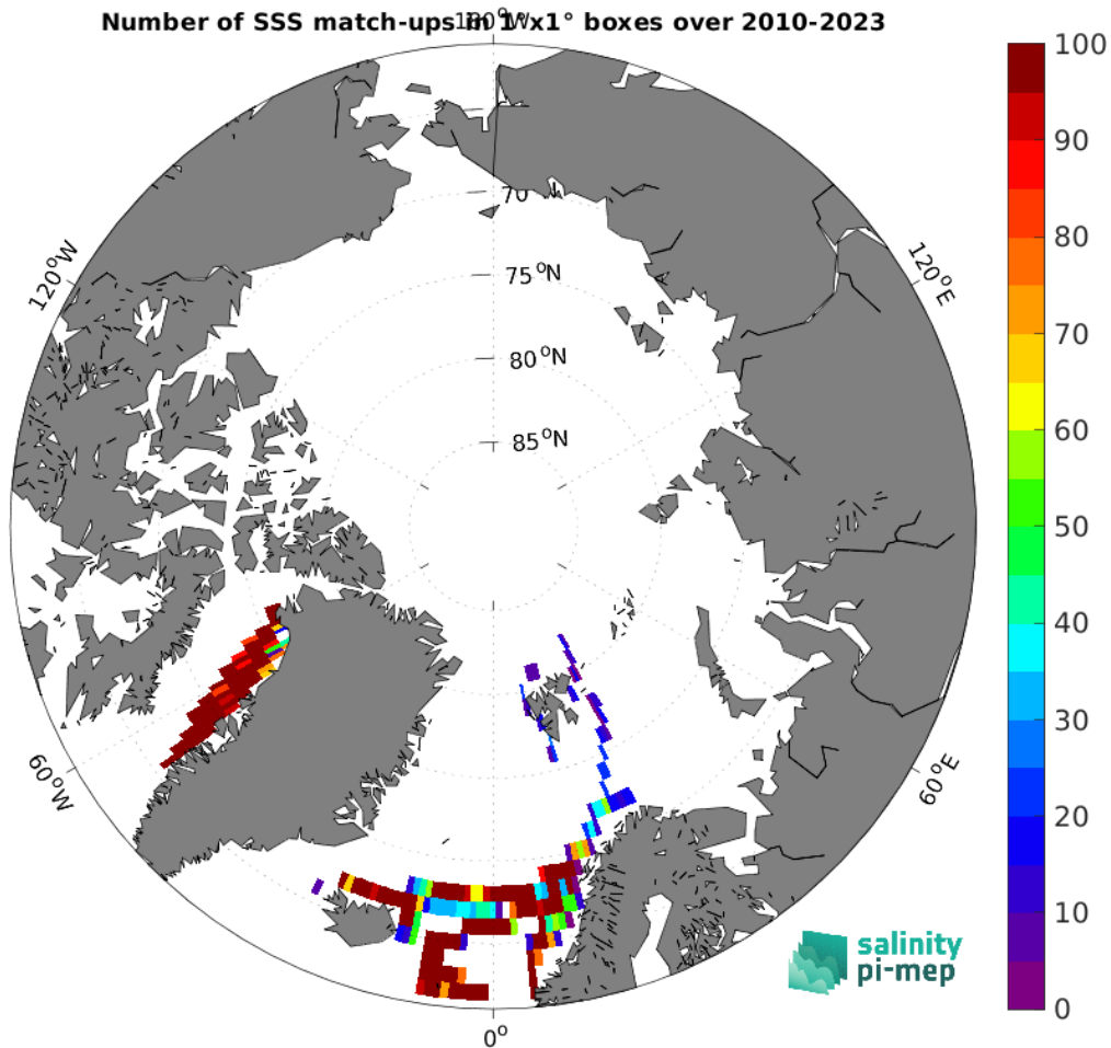
Figure 5: Number of SSS match-ups between TSG (LEGOS-DM) SSS and the SMOS SSS L3 v9 - 9 Days (CATDS-CEC-LOCEAN) SSS product for the Arctic Ocean Pi-MEP region over 1^\circ \times 1^\circ boxes and for the full satellite product period.
