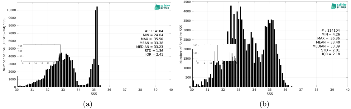
Figure 3: Histograms of SSS from TSG (LEGOS-DM) (a) and SMOS SSS L3 v9 - 9 Days (CATDS-CEC-LOCEAN) (b) considering all match-up pairs per bins of 0.1 over the Arctic Ocean Pi-MEP region and for the full satellite product period.
