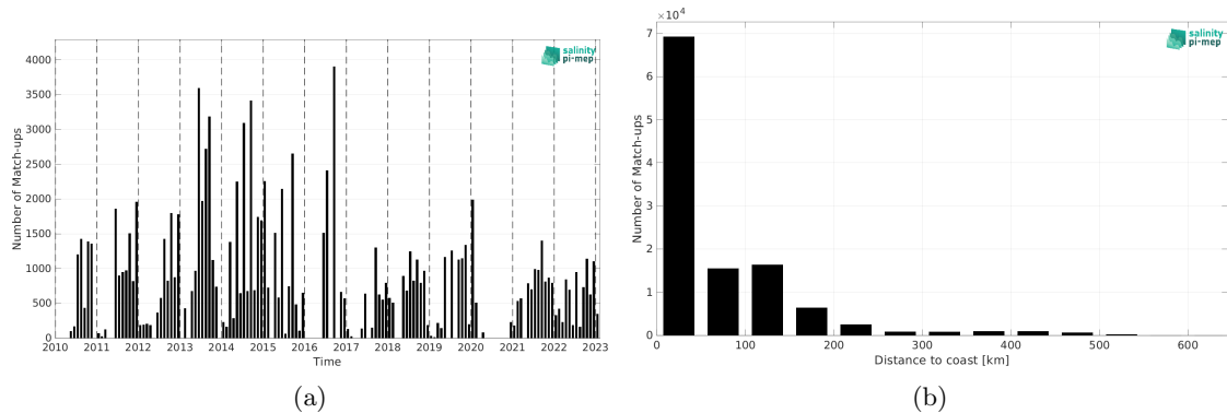
Figure 2: Number of match-ups between TSG (LEGOS-DM) and SMOS SSS L3 v9 - 9 Days (CATDS-CEC-LOCEAN) SSS as a function of time (a) and as function of the distance to coast (b) over the Arctic Ocean Pi-MEP region and for the full satellite product period.
