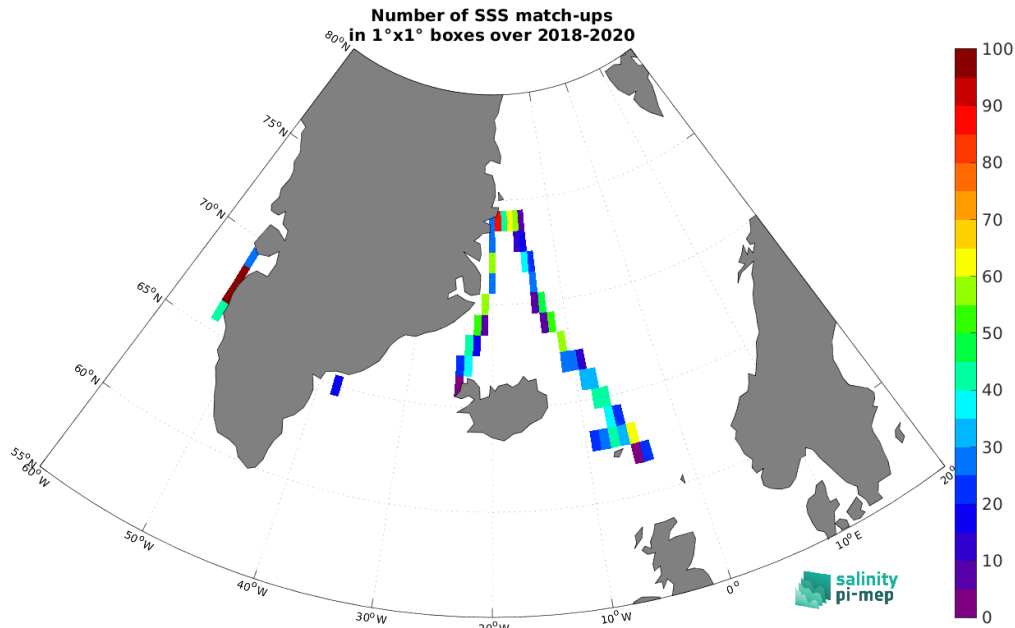
Figure 5: Number of SSS match-ups between TSG (Lauge-Koch) SSS and the SMOS SSS L3 v9 - 9 Days (CATDS-CEC-LOCEAN) SSS product for the Arctic Ocean Pi-MEP region over 1^\circ \times 1^\circ boxes and for the full satellite product period.
