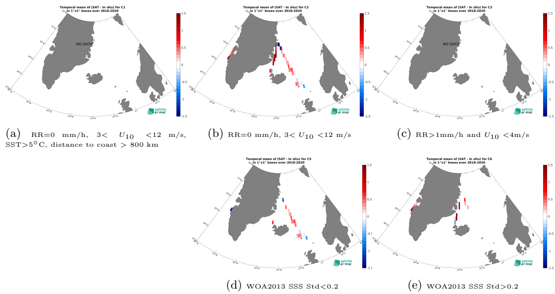
Figure 14: Temporal mean gridded over spatial boxes of size 1^\circ \times 1^\circ of \Delta SSS (SMOS SSS L3 v9 - 9 Days (CATDS-CEC-LOCEAN) - TSG (Lauge-Koch)) for 5 different subdatasets corresponding to:RR=0 mm/h, 3 < U_{10} < 12 m/s, SST >5^\circ C, distance to coast > 800 km (a), RR=0 mm/h, 3 < U_{10} < 12 m/s (b), RR >1 mm/h and U_{10} < 4 m/s (c), WOA2013 SSS Std <0.2 (d), WOA2013 SSS Std >0.2 (e).
