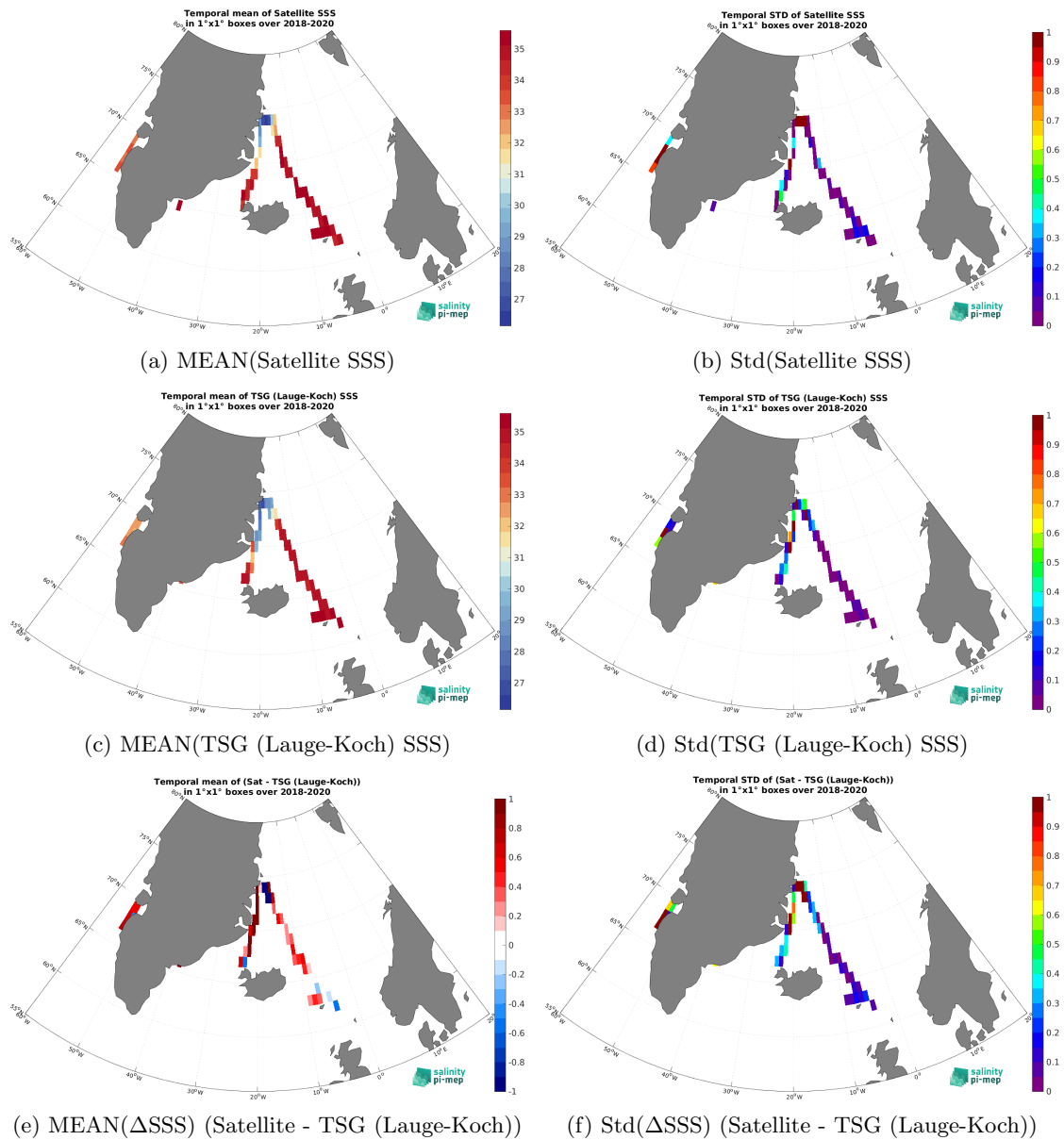
Figure 7: Temporal mean (left) and Std (right) of SSS from SMOS SSS L3 v9 - 9 Days (CATDS-CEC-LOCEAN) (top), TSG (Lauge-Koch) (middle), and of \Delta SSS (Satellite - TSG (Lauge-Koch)). Only match-up pairs are used to generate these maps.
