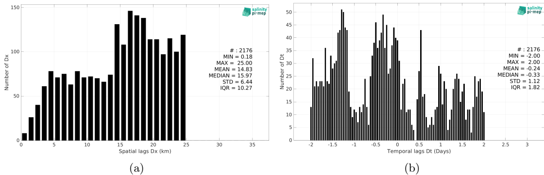
Figure 6: Histograms of the spatial (a) and temporal (b) lags between the location/time of the TSG (Lauge-Koch) measurement and the date of the corresponding SMOS SSS L3 v9 - 9 Days (CATDS-CEC-LOCEAN) SSS pixel.
