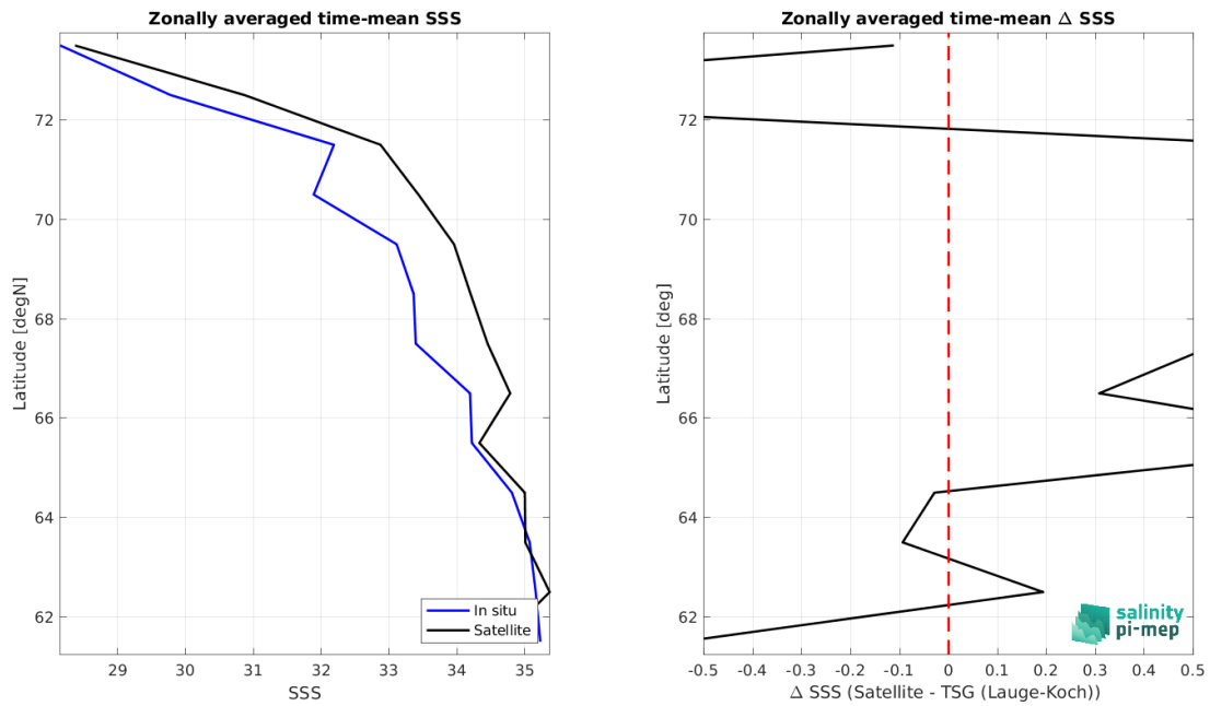
Figure 9: Left panel: Zonal mean SSS from SMOS SSS L3 v9 - 9 Days (CATDS-CEC-LOCEAN) satellite product (black) and from TSG (Lauge-Koch) (blue). Right panel: Zonal mean of \Delta SSS (Satellite - TSG (Lauge-Koch)) for all the collected Pi-MEP match-up pairs estimated over the full satellite product period.
