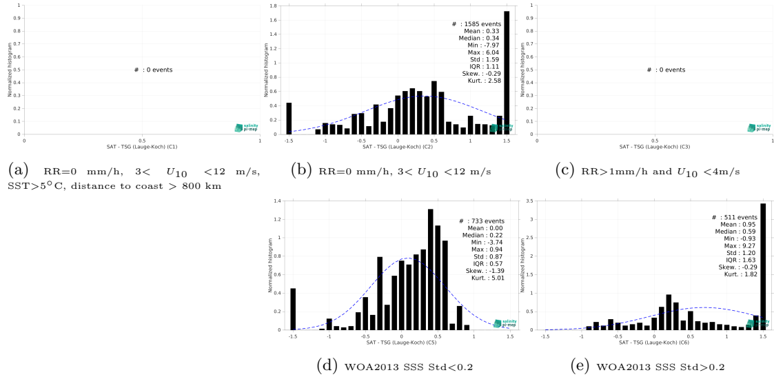
Figure 15: Normalized histogram of \Delta SSS (SMOS SSS L3 v9 - 9 Days (CATDS-CEC-LOCEAN) - TSG (Lauge-Koch)) for 5 different subdatasets corresponding to: RR=0 mm/h, 3 < U_{10} < 12 m/s, SST > 5°C, distance to coast > 800 km (a), RR=0 mm/h, 3 < U_{10} < 12 m/s (b), RR > 1mm/h and U_{10} < 4 m/s (c), WOA2013 SSS Std < 0.2 (d), WOA2013 SSS Std > 0.2 (e).
