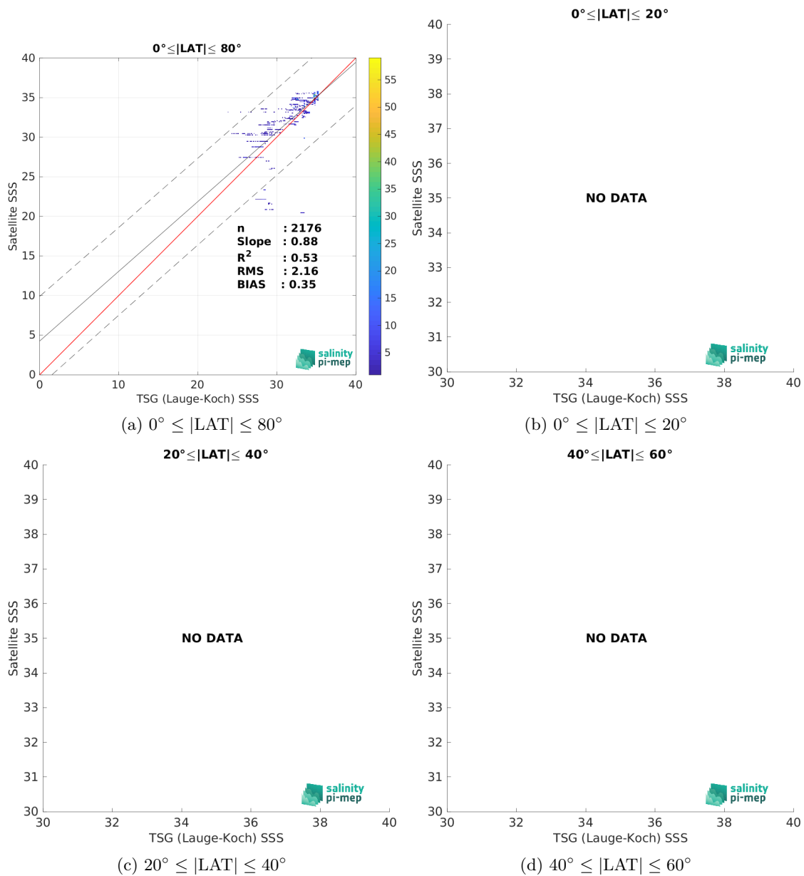
Figure 10: Contour maps of the concentration of SMOS SSS L3 v9 - 9 Days (CATDS-CEC-LOCEAN) SSS (y-axis) versus TSG (Lauge-Koch) SSS (x-axis) at match-up pairs for different latitude bands. For each plot, the red line shows x=y . The black thin and dashed lines indicate a linear fit through the data cloud and the \pm 95\% confidence levels, respectively. The number match-up pairs n , the slope and R^2 coefficient of the linear fit, the root mean square (RMS) and the mean bias between satellite and in situ data are indicated for each latitude band in each plots.
