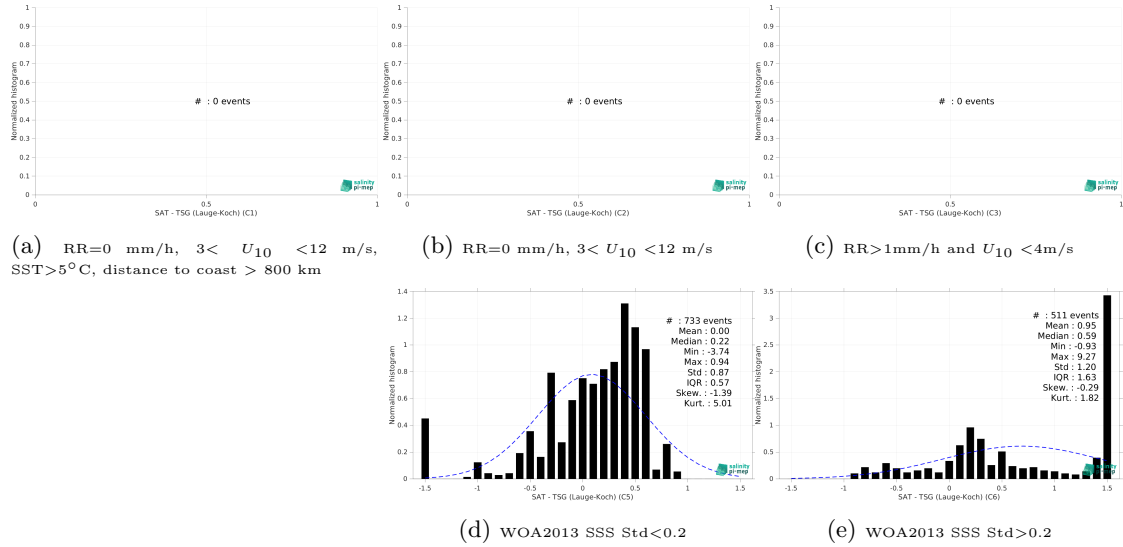
Figure 13: Normalized histogram of \Delta SSS (SMOS SSS L3 v9 - 9 Days (CATDS-CEC-LOCEAN) - TSG (Laue-Koch)) for 5 different subdatasets corresponding to: RR=0 mm/h, 3 < U_{10} < 12 m/s, SST>5°C, distance to coast > 800 km (a), RR=0 mm/h, 3 < U_{10} < 12 m/s (b), RR>1mm/h and U_{10} < 4 m/s (c), WOA2013 SSS Std<0.2 (d), WOA2013 SSS Std>0.2 (e).
