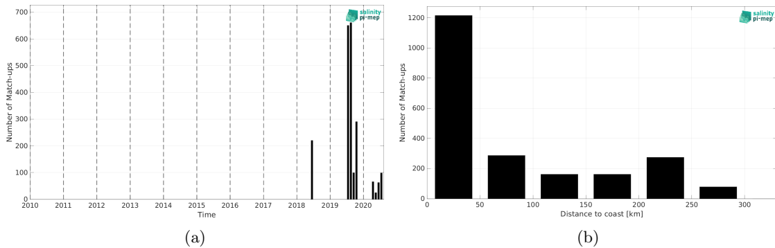
Figure 1: Number of match-ups between TSG (Lauge-Koch) and SMOS SSS L3 v9 - 9 Days (CATDS-CEC-LOCEAN) SSS as a function of time (a) and as function of the distance to coast (b) over the Arctic Ocean Pi-MEP region and for the full satellite product period.
