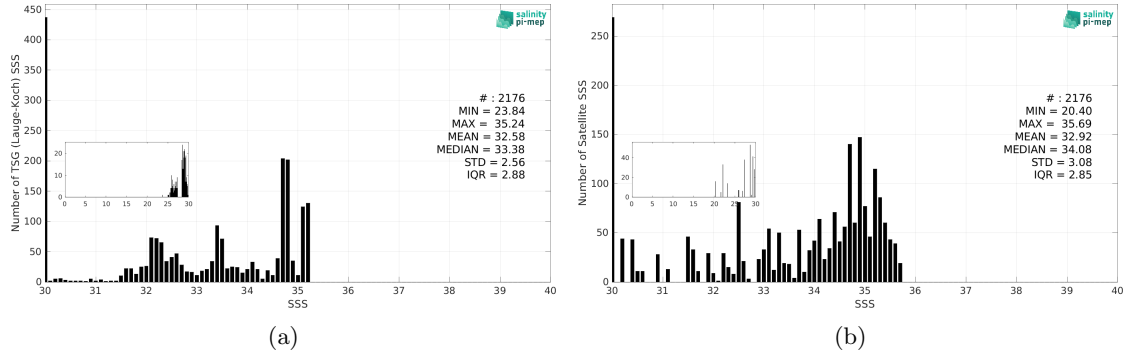
Figure 2: Histograms of SSS from TSG (Lauge-Koch) (a) and SMOS SSS L3 v9 - 9 Days (CATDS-CEC-LOCEAN) (b) considering all match-up pairs per bins of 0.1 over the Arctic Ocean Pi-MEP region and for the full satellite product period.
