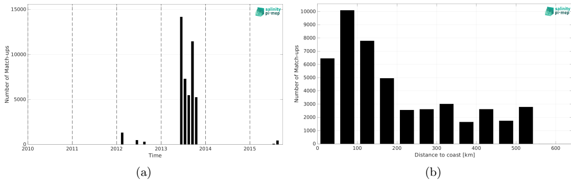
Figure 1: Number of match-ups between TSG (GOSUD-Sailing-ship) and SMOS SSS L3 v9 - 9 Days (CATDS-CEC-LOCEAN) SSS as a function of time (a) and as function of the distance to coast (b) over the Arctic Ocean Pi-MEP region and for the full satellite product period.
