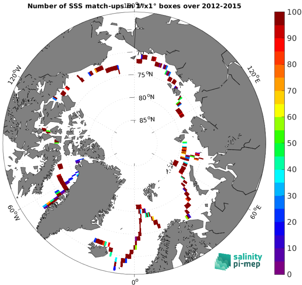
Figure 4: Number of SSS match-ups between TSG (GOSUD-Sailing-ship) SSS and the SMOS SSS L3 v9 - 9 Days (CATDS-CEC-LOCEAN) SSS product for the Arctic Ocean Pi-MEP region over 1^\circ \times 1^\circ boxes and for the full satellite product period.
