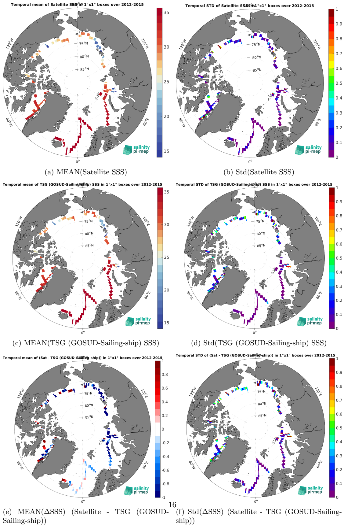
Figure 6: Temporal mean (left) and Std (right) of SSS from SMOS SSS L3 v9 - 9 Days (CATDS-CEC-LOCEAN) (top), TSG (GOSUD-Sailing-ship) (middle), and of \Delta SSS (Satellite - TSG (GOSUD-Sailing-ship)). Only match-up pairs are used to generate these maps.
