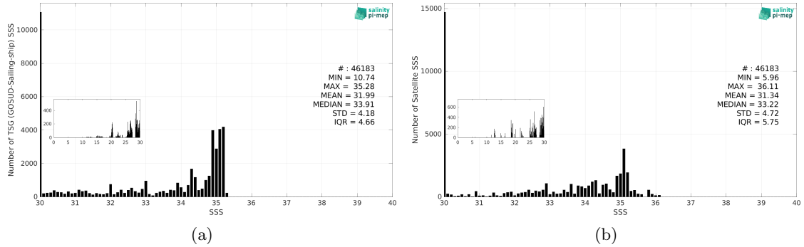
Figure 2: Histograms of SSS from TSG (GOSUD-Sailing-ship) (a) and SMOS SSS L3 v9 - 9 Days (CATDS-CEC-LOCEAN) (b) considering all match-up pairs per bins of 0.1 over the Arctic Ocean Pi-MEP region and for the full satellite product period.
