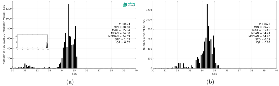
Figure 3: Histograms of SSS from TSG (GOSUD-Research-vessel) (a) and SMOS SSS L3 v9 - 9 Days (CATDS-CEC-LOCEAN) (b) considering all match-up pairs per bins of 0.1 over the Arctic Ocean Pi-MEP region and for the full satellite product period.
