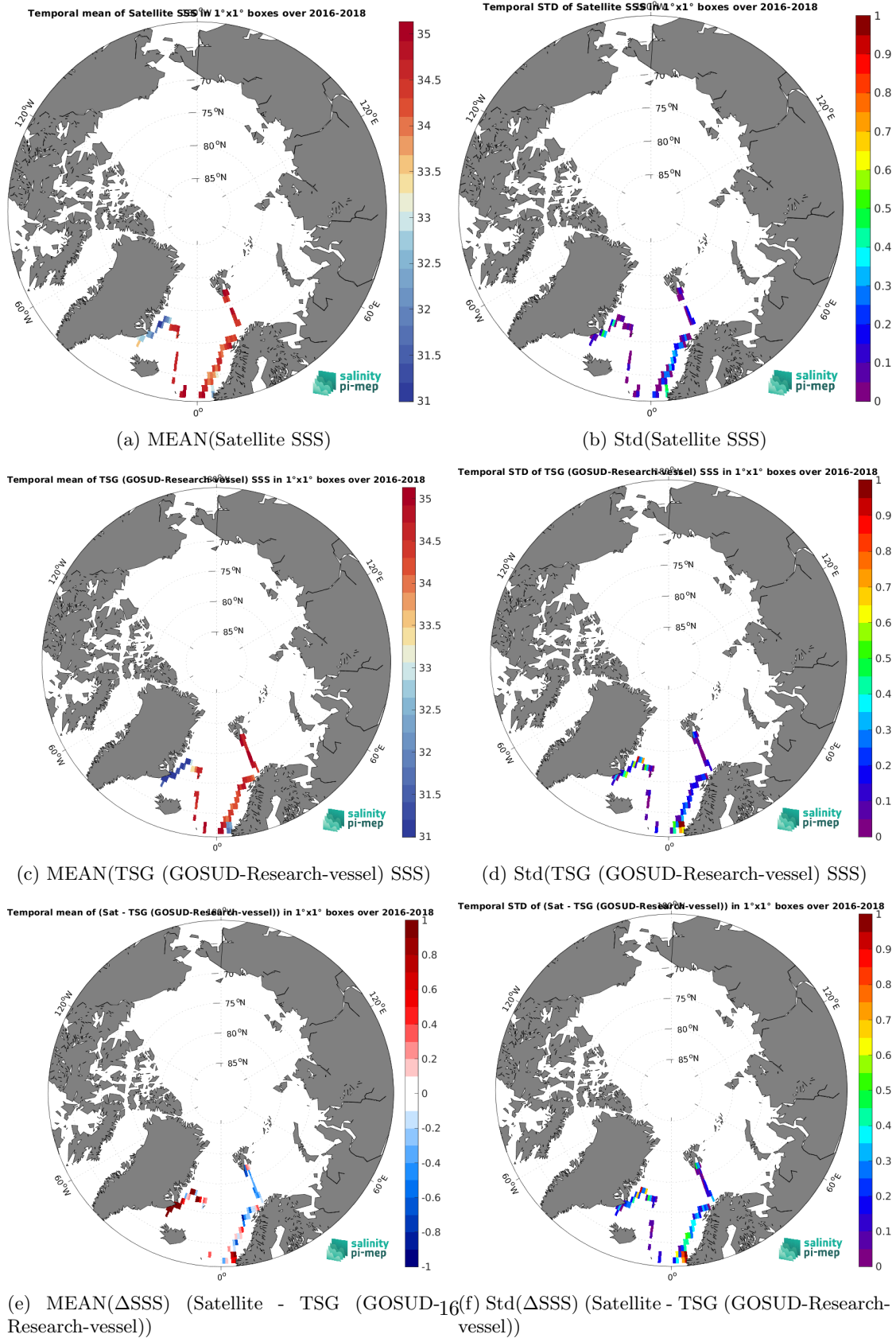
Figure 7: Temporal mean (left) and Std (right) of SSS from SMOS SSS L3 v9 - 9 Days (CATDS-CEC-LOCEAN) (top), TSG (GOSUD-Research-vessel) (middle), and of \Delta SSS (Satellite - TSG (GOSUD-Research-vessel)). Only match-up pairs are used to generate these maps.
