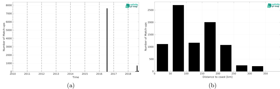
Figure 2: Number of match-ups between TSG (GOSUD-Research-vessel) and SMOS SSS L3 v9 - 9 Days (CATDS-CEC-LOCEAN) SSS as a function of time (a) and as function of the distance to coast (b) over the Arctic Ocean Pi-MEP region and for the full satellite product period.
