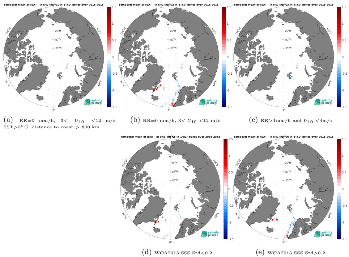
Figure 14: Temporal mean gridded over spatial boxes of size 1^\circ \times 1^\circ of \Delta\text{SSS} (SMOS SSS L3 v9 - 9 Days (CATDS-CEC-LOCEAN) - TSG (GOSUD-Research-vessel)) for 5 different subdatasets corresponding to: RR=0 mm/h, 3 < U_{10} < 12 m/s, SST > 5°C, distance to coast > 800 km (a), RR=0 mm/h, 3 < U_{10} < 12 m/s (b), RR > 1mm/h and U_{10} < 4 m/s (c), WOA2013 SSS Std < 0.2 (d), WOA2013 SSS Std > 0.2 (e).
