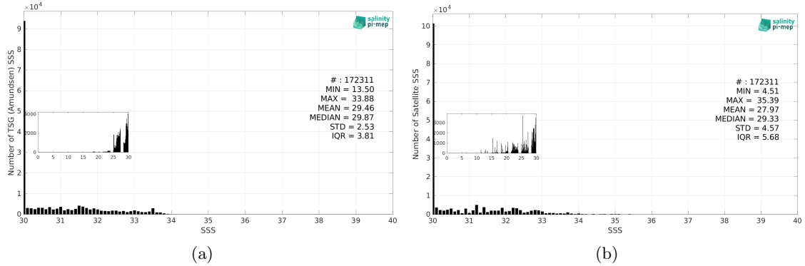
Figure 3: Histograms of SSS from TSG (Amundsen) (a) and SMOS SSS L3 v9 - 9 Days (CATDS-CEC-LOCEAN) (b) considering all match-up pairs per bins of 0.1 over the Arctic Ocean Pi-MEP region and for the full satellite product period.
