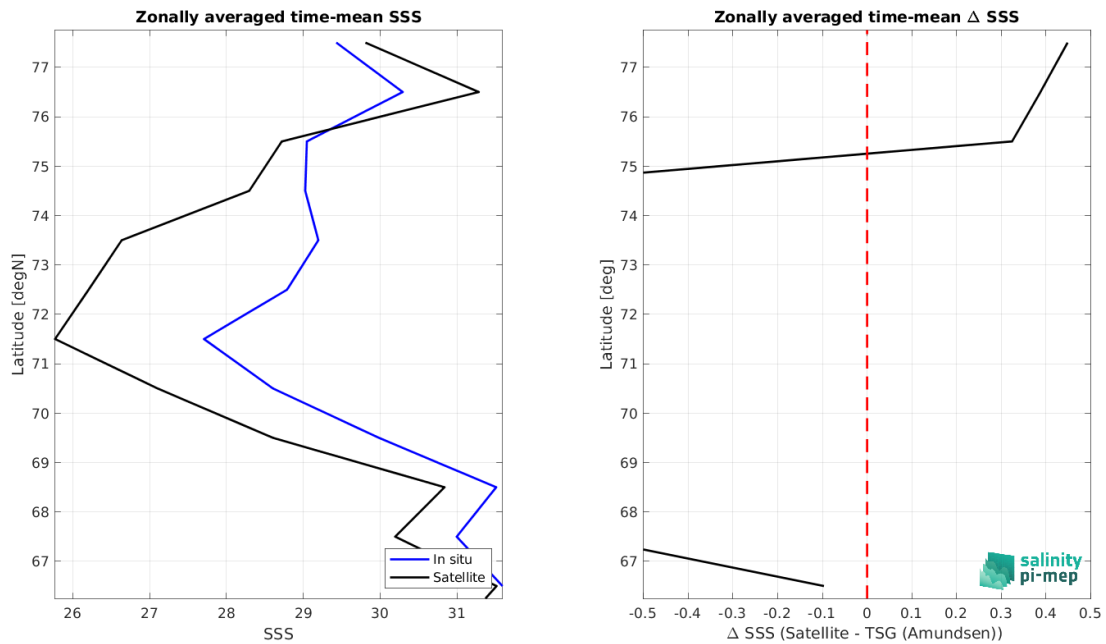
Figure 9: Left panel: Zonal mean SSS from SMOS SSS L3 v9 - 9 Days (CATDS-CEC-LOCEAN) satellite product (black) and from TSG (Amundsen) (blue). Right panel: Zonal mean of \Delta SSS (Satellite - TSG (Amundsen)) for all the collected Pi-MEP match-up pairs estimated over the full satellite product period.
