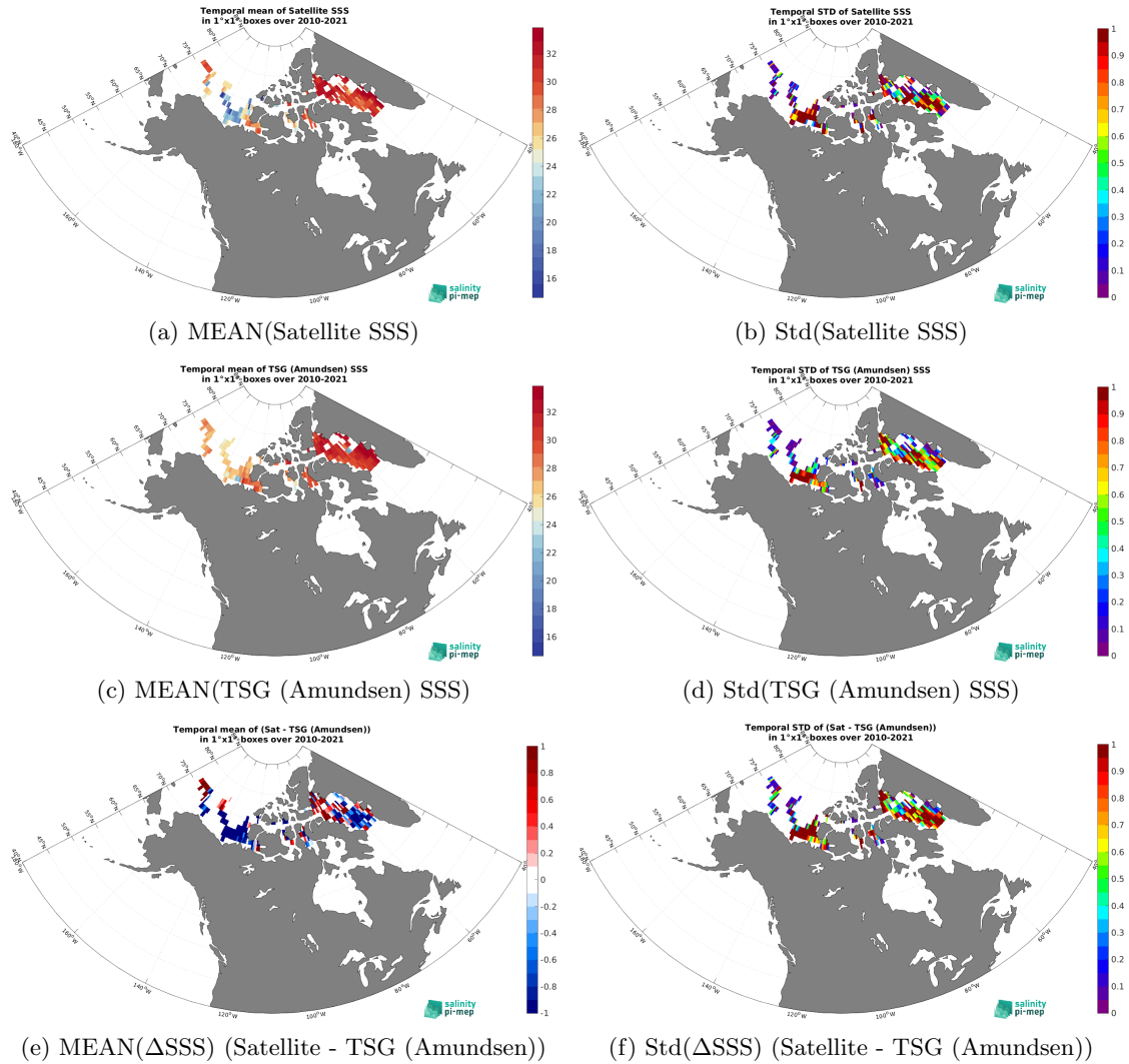
Figure 7: Temporal mean (left) and Std (right) of SSS from SMOS SSS L3 v9 - 9 Days (CATDS-CEC-LOCEAN) (top), TSG (Amundsen) (middle), and of \Delta SSS (Satellite - TSG (Amundsen)). Only match-up pairs are used to generate these maps.
