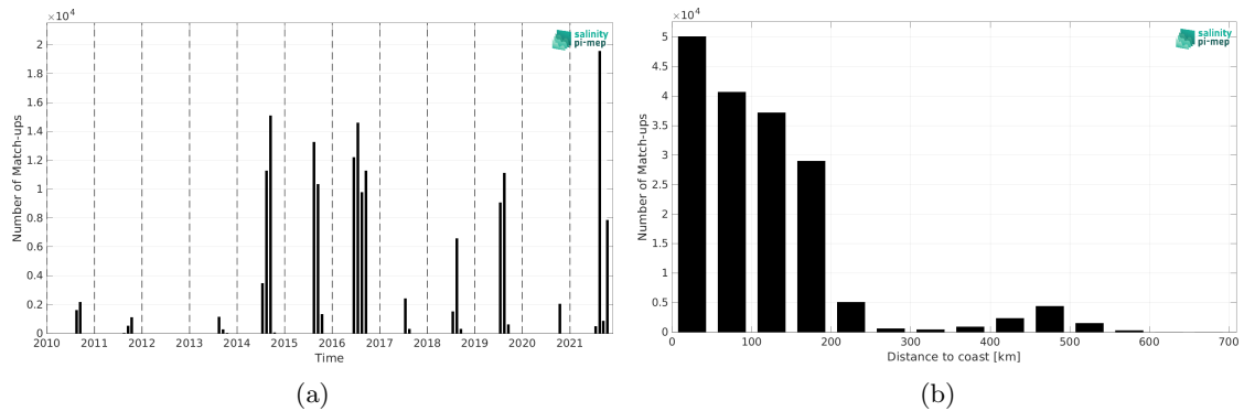
Figure 2: Number of match-ups between TSG (Amundsen) and SMOS SSS L3 v9 - 9 Days (CATDS-CEC-LOCEAN) SSS as a function of time (a) and as function of the distance to coast (b) over the Arctic Ocean Pi-MEP region and for the full satellite product period.
