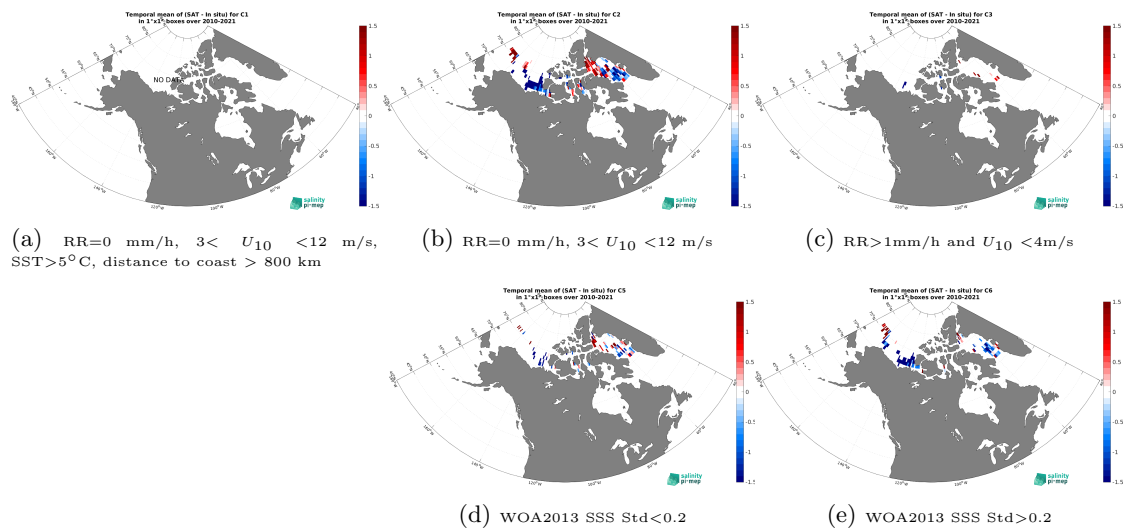
Figure 14: Temporal mean gridded over spatial boxes of size 1^\circ \times 1^\circ of \Delta SSS (SMOS SSS L3 v9 - 9 Days (CATDS-CEC-LOCEAN) - TSG (Amundsen)) for 5 different subdatasets corresponding to:RR=0 mm/h, 3 < U_{10} < 12 m/s, SST > 5°C, distance to coast > 800 km (a), RR=0 mm/h, 3 < U_{10} < 12 m/s (b), RR > 1mm/h and U_{10} < 4 m/s (c), WOA2013 SSS Std < 0.2 (d), WOA2013 SSS Std > 0.2 (e).
