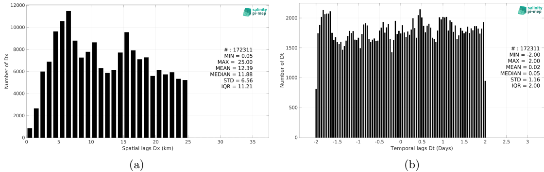
Figure 6: Histograms of the spatial (a) and temporal (b) lags between the location/time of the TSG (Amundsen) measurement and the date of the corresponding SMOS SSS L3 v9 - 9 Days (CATDS-CEC-LOCEAN) SSS pixel.
