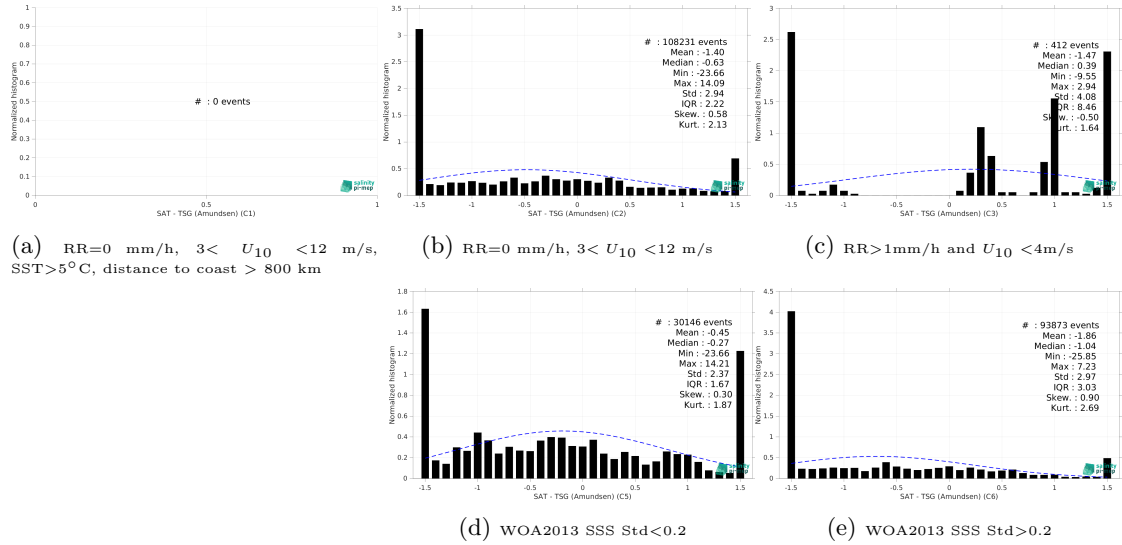
Figure 15: Normalized histogram of \Delta SSS (SMOS SSS L3 v9 - 9 Days (CATDS-CEC-LOCEAN) - TSG (Amundsen)) for 5 different subdatasets corresponding to: RR=0 mm/h, 3 < U_{10} < 12 m/s, SST>5°C, distance to coast > 800 km (a), RR=0 mm/h, 3 < U_{10} < 12 m/s (b), RR>1mm/h and U_{10} < 4 m/s (c), WOA2013 SSS Std<0.2 (d), WOA2013 SSS Std>0.2 (e).
