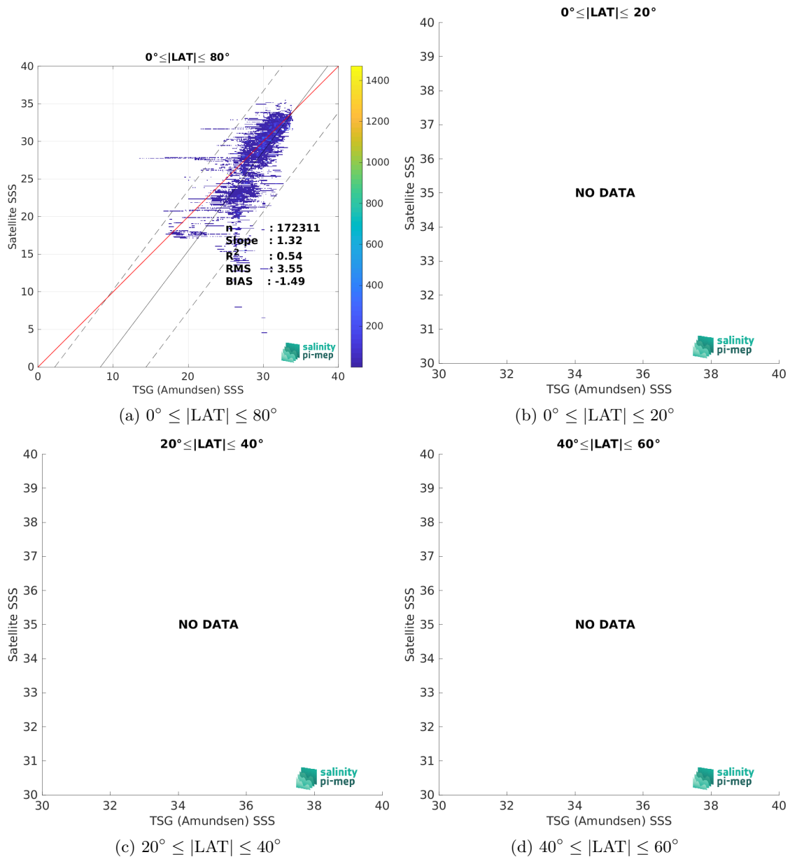
Figure 10: Contour maps of the concentration of SMOS SSS L3 v9 - 9 Days (CATDS-CEC-LOCEAN) SSS (y-axis) versus TSG (Amundsen) SSS (x-axis) at match-up pairs for different latitude bands. For each plot, the red line shows x=y . The black thin and dashed lines indicate a linear fit through the data cloud and the \pm 95\% confidence levels, respectively. The number match-up pairs n , the slope and R^2 coefficient of the linear fit, the root mean square (RMS) and the mean bias between satellite and in situ data are indicated for each latitude band in each plots.
