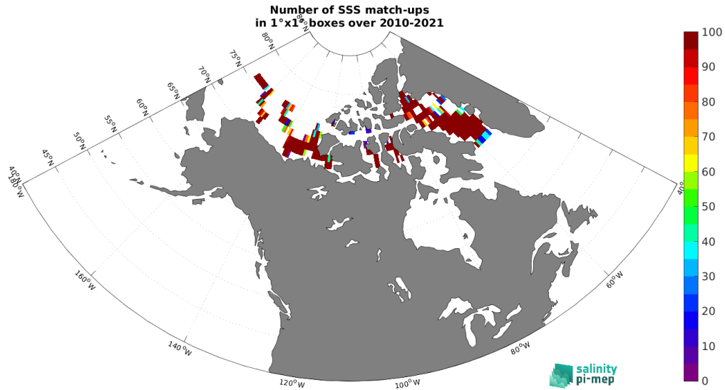
Figure 5: Number of SSS match-ups between TSG (Amundsen) SSS and the SMOS SSS L3 v9 - 9 Days (CATDS-CEC-LOCEAN) SSS product for the Arctic Ocean Pi-MEP region over 1^\circ \times 1^\circ boxes and for the full satellite product period.
