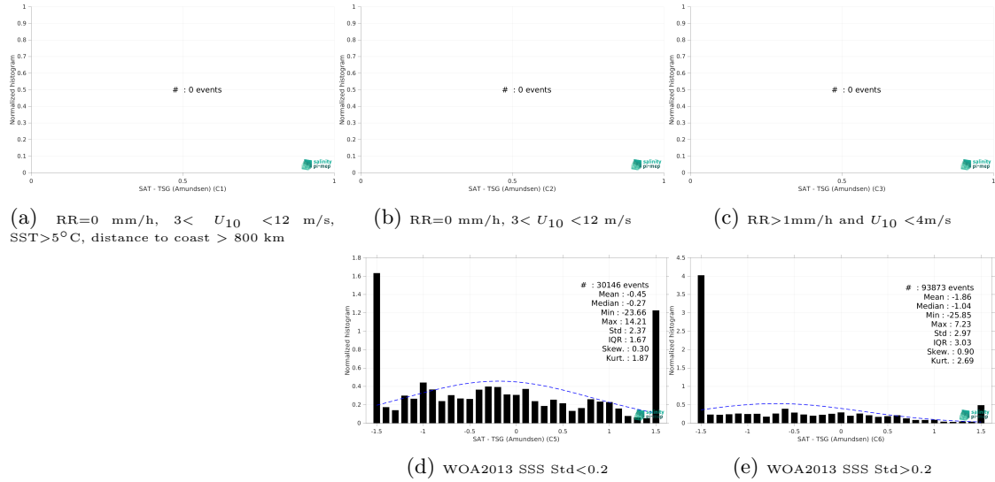
Figure 13: Normalized histogram of \Delta SSS (SMOS SSS L3 v9 - 9 Days (CATDS-CEC-LOCEAN) - TSG (Amundsen)) for 5 different subdatasets corresponding to: RR=0 mm/h, 3 < U_{10} < 12 m/s, SST >5^{\circ} C, distance to coast > 800 km (a), RR=0 mm/h, 3 < U_{10} < 12 m/s (b), RR >1 mm/h and U_{10} < 4 m/s (c), WOA2013 SSS Std <0.2 (d), WOA2013 SSS Std >0.2 (e).
