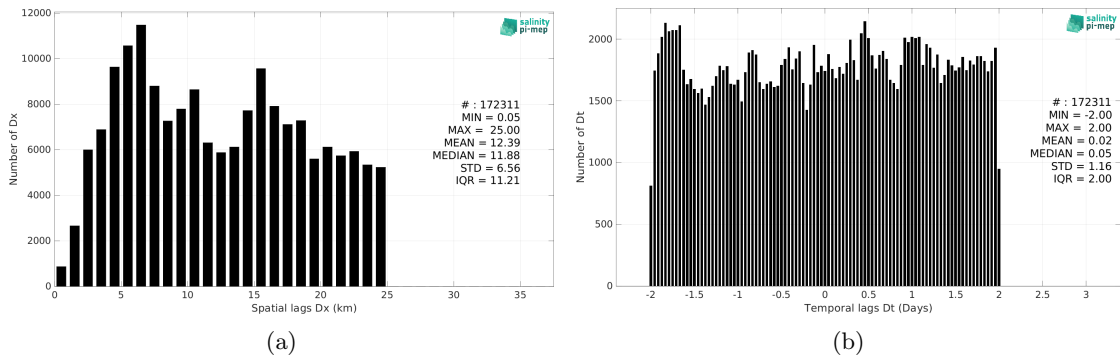
Figure 5: Histograms of the spatial (a) and temporal (b) lags between the location/time of the TSG (Amundsen) measurement and the date of the corresponding SMOS SSS L3 v9 - 9 Days (CATDS-CEC-LOCEAN) SSS pixel.
