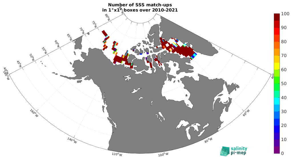
Figure 4: Number of SSS match-ups between TSG (Amundsen) SSS and the SMOS SSS L3 v9 - 9 Days (CATDS-CEC-LOCEAN) SSS product for the Arctic Ocean Pi-MEP region over 1^\circ \times 1^\circ boxes and for the full satellite product period.
