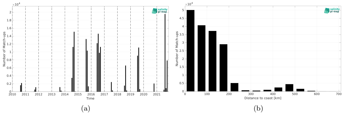
Figure 1: Number of match-ups between TSG (Amundsen) and SMOS SSS L3 v9 - 9 Days (CATDS-CEC-LOCEAN) SSS as a function of time (a) and as function of the distance to coast (b) over the Arctic Ocean Pi-MEP region and for the full satellite product period.
