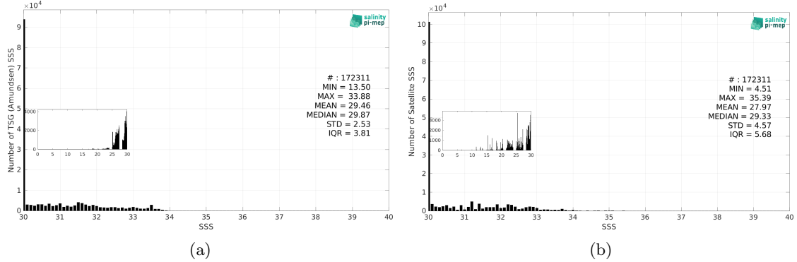
Figure 2: Histograms of SSS from TSG (Amundsen) (a) and SMOS SSS L3 v9 - 9 Days (CATDS-CEC-LOCEAN) (b) considering all match-up pairs per bins of 0.1 over the Arctic Ocean Pi-MEP region and for the full satellite product period.
