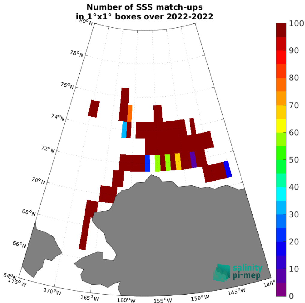
Figure 5: Number of SSS match-ups between SASSIE SSS and the SMOS SSS L3 v9 - 9 Days (CATDS-CEC-LOCEAN) SSS product for the Arctic Ocean Pi-MEP region over 1^\circ \times 1^\circ boxes and for the full satellite product period.
