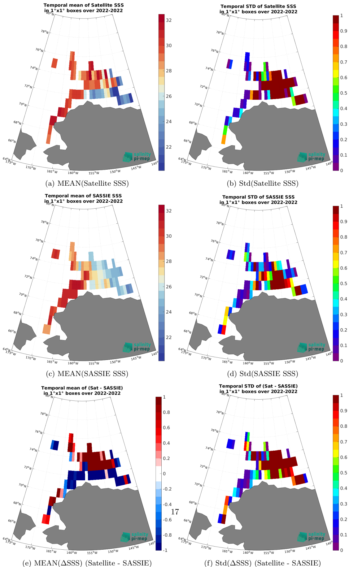
Figure 7: Temporal mean (left) and Std (right) of SSS from SMOS SSS L3 v9 - 9 Days (CATDS-CEC-LOCEAN) (top), SASSIE (middle), and of \Delta SSS (Satellite - SASSIE). Only match-up pairs are used to generate these maps.
