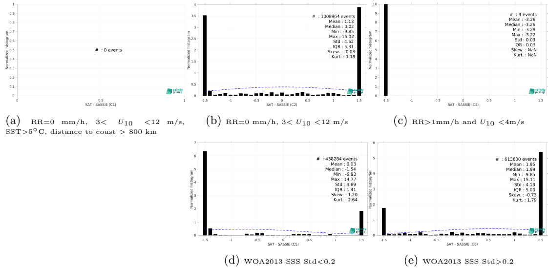
Figure 15: Normalized histogram of \Delta SSS (SMOS SSS L3 v9 - 9 Days (CATDS-CEC-LOCEAN) - SASSIE) for 5 different subdatasets corresponding to: RR=0 mm/h, 3 < U_{10} < 12 m/s, SST > 5°C, distance to coast > 800 km (a), RR=0 mm/h, 3 < U_{10} < 12 m/s (b), RR > 1mm/h and U_{10} < 4 m/s (c), WOA2013 SSS Std < 0.2 (d), WOA2013 SSS Std > 0.2 (e).
