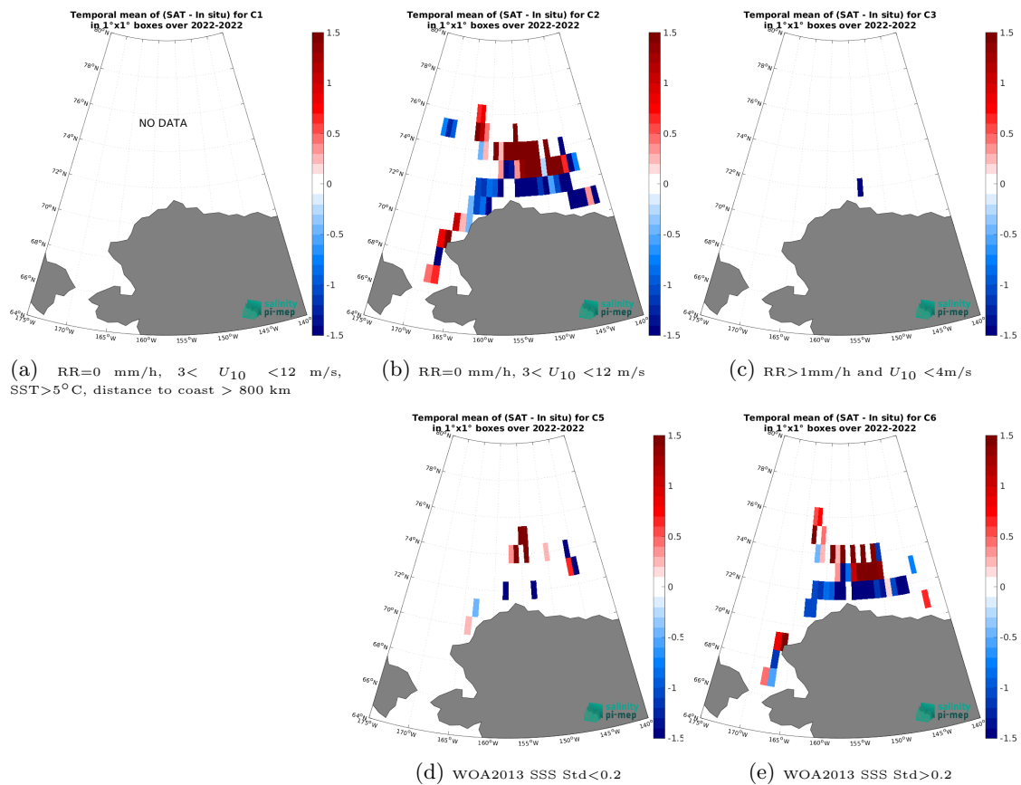
Figure 14: Temporal mean gridded over spatial boxes of size 1^\circ \times 1^\circ of \Delta\text{SSS} (SMOS SSS L3 v9 - 9 Days (CATDS-CEC-LOCEAN) - SASSIE) for 5 different subdatasets corresponding to:RR=0 mm/h, 3 < U_{10} < 12 m/s, SST>5°C, distance to coast > 800 km (a), RR=0 mm/h, 3 < U_{10} < 12 m/s (b), RR>1mm/h and U_{10} < 4 m/s (c), WOA2013 SSS Std<0.2 (d), WOA2013 SSS Std>0.2 (e).
