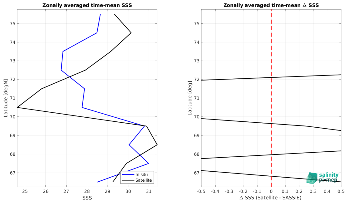
Figure 9: Left panel: Zonal mean SSS from SMOS SSS L3 v9 - 9 Days (CATDS-CEC-LOCEAN) satellite product (black) and from SASSIE (blue). Right panel: Zonal mean of \Delta SSS (Satellite - SASSIE) for all the collected Pi-MEP match-up pairs estimated over the full satellite product period.
