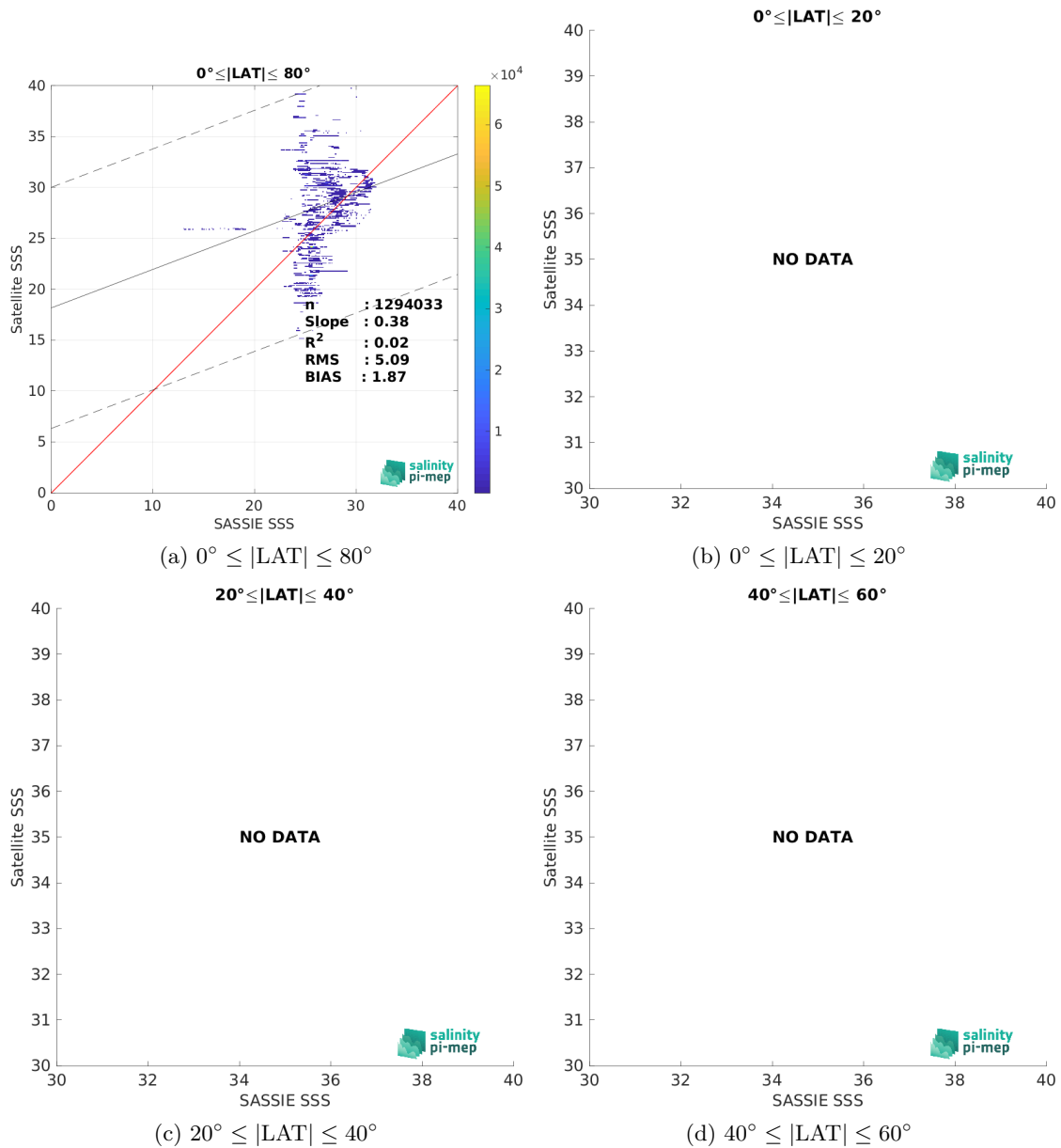
Figure 10: Contour maps of the concentration of SMOS SSS L3 v9 - 9 Days (CATDS-CEC-LOCEAN) SSS (y-axis) versus SASSIE SSS (x-axis) at match-up pairs for different latitude bands. For each plot, the red line shows x=y . The black thin and dashed lines indicate a linear fit through the data cloud and the \pm 95\% confidence levels, respectively. The number match-up pairs n , the slope and R^2 coefficient of the linear fit, the root mean square (RMS) and the mean bias between satellite and in situ data are indicated for each latitude band in each plots.
