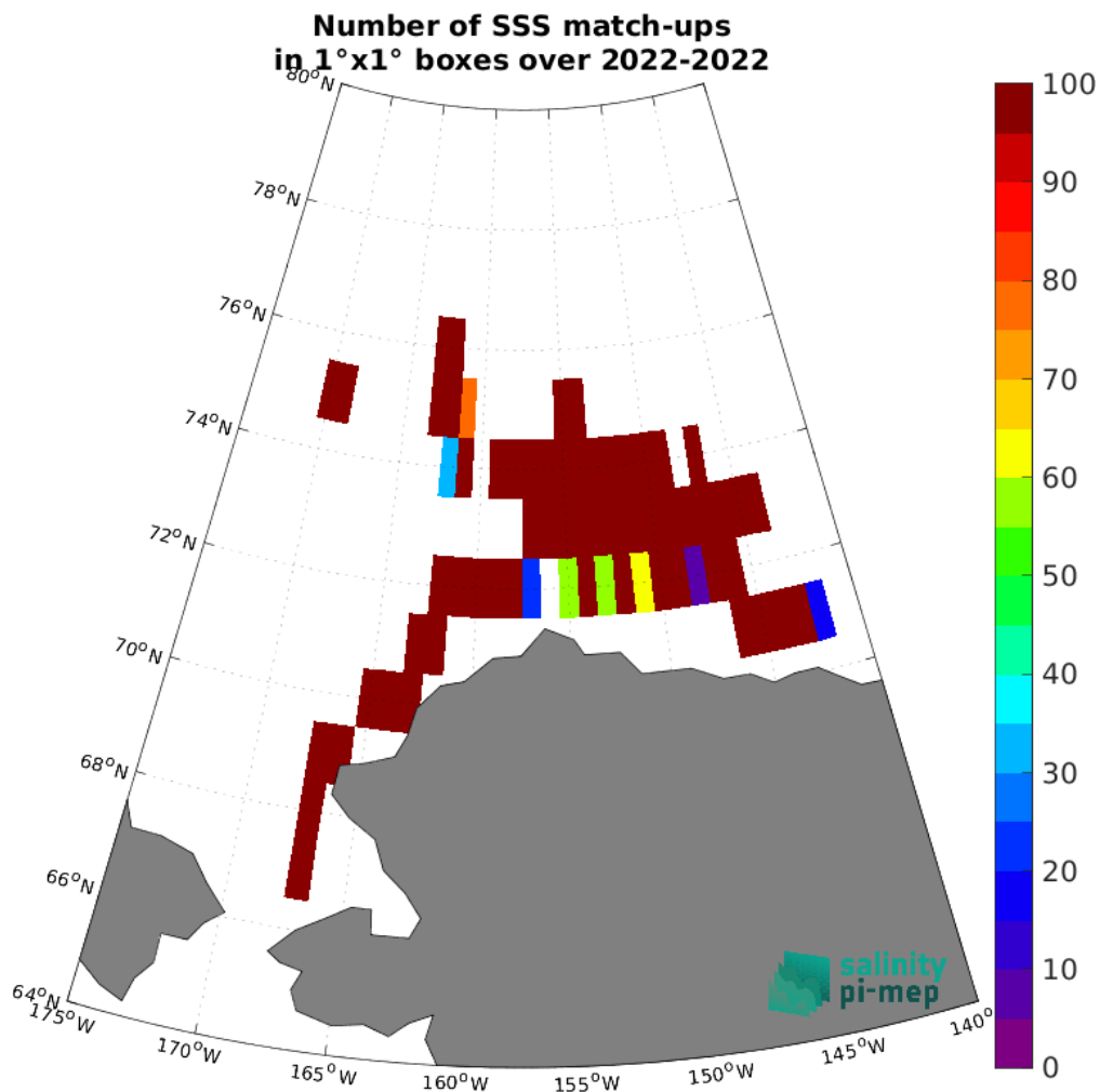
Figure 5: Number of SSS match-ups between SASSIE SSS and the SMOS SSS L3 v9 - 9 Days (CATDS-CEC-LOCEAN) SSS product for the Arctic Ocean Pi-MEP region over 1°x1° boxes and for the full satellite product period.
