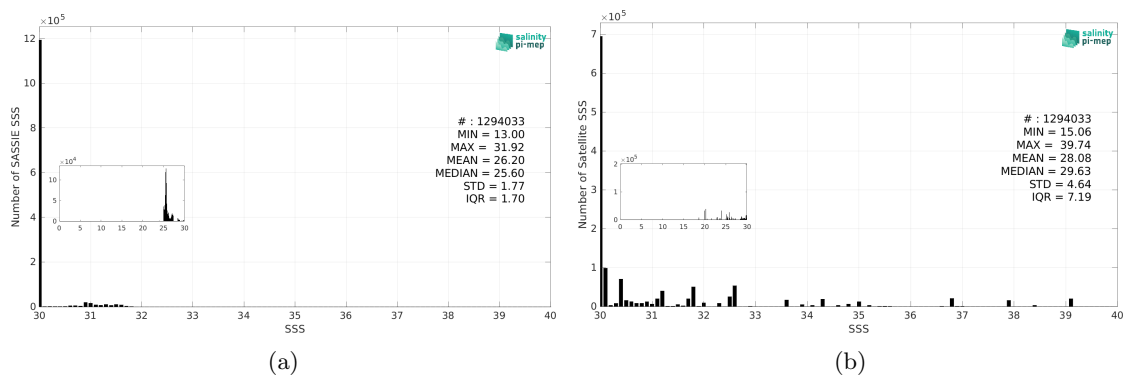
Figure 3: Histograms of SSS from SASSIE (a) and SMOS SSS L3 v9 - 9 Days (CATDS-CEC-LOCEAN) (b) considering all match-up pairs per bins of 0.1 over the Arctic Ocean Pi-MEP region and for the full satellite product period.
