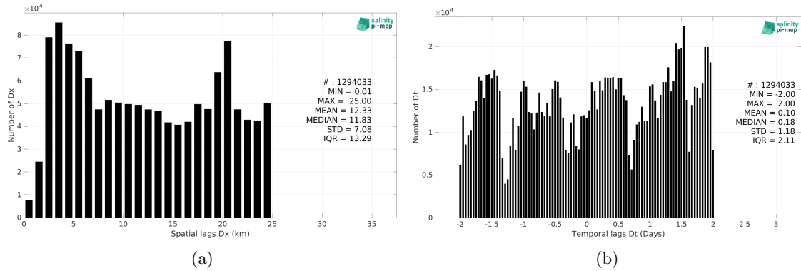
Figure 6: Histograms of the spatial (a) and temporal (b) lags between the location/time of the SASSIE measurement and the date of the corresponding SMOS SSS L3 v9 - 9 Days (CATDS-CEC-LOCEAN) SSS pixel.
