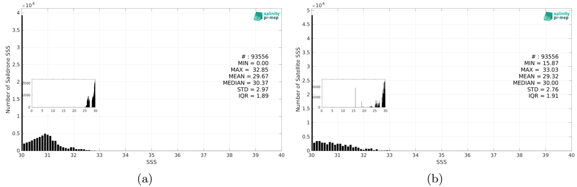
Figure 3: Histograms of SSS from Saildrone (a) and SMOS SSS L3 v9 - 9 Days (CATDS-CEC-LOCEAN) (b) considering all match-up pairs per bins of 0.1 over the Arctic Ocean Pi-MEP region and for the full satellite product period.
