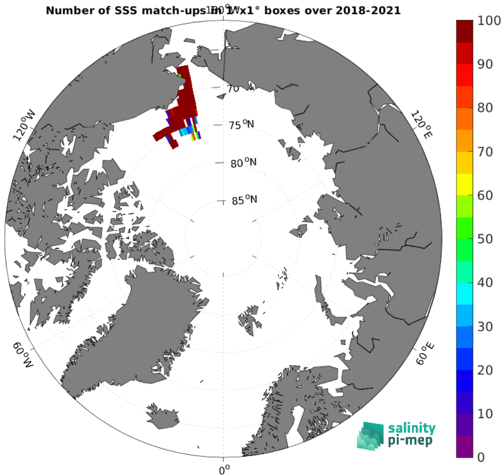
Figure 5: Number of SSS match-ups between Saildrone SSS and the SMOS SSS L3 v9 - 9 Days (CATDS-CEC-LOCEAN) SSS product for the Arctic Ocean Pi-MEP region over 1^{\circ} \times 1^{\circ} boxes and for the full satellite product period.
