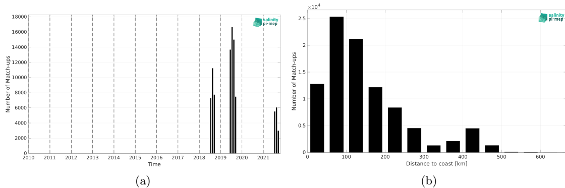
Figure 2: Number of match-ups between Saildrone and SMOS SSS L3 v9 - 9 Days (CATDS-CEC-LOCEAN) SSS as a function of time (a) and as function of the distance to coast (b) over the Arctic Ocean Pi-MEP region and for the full satellite product period.
