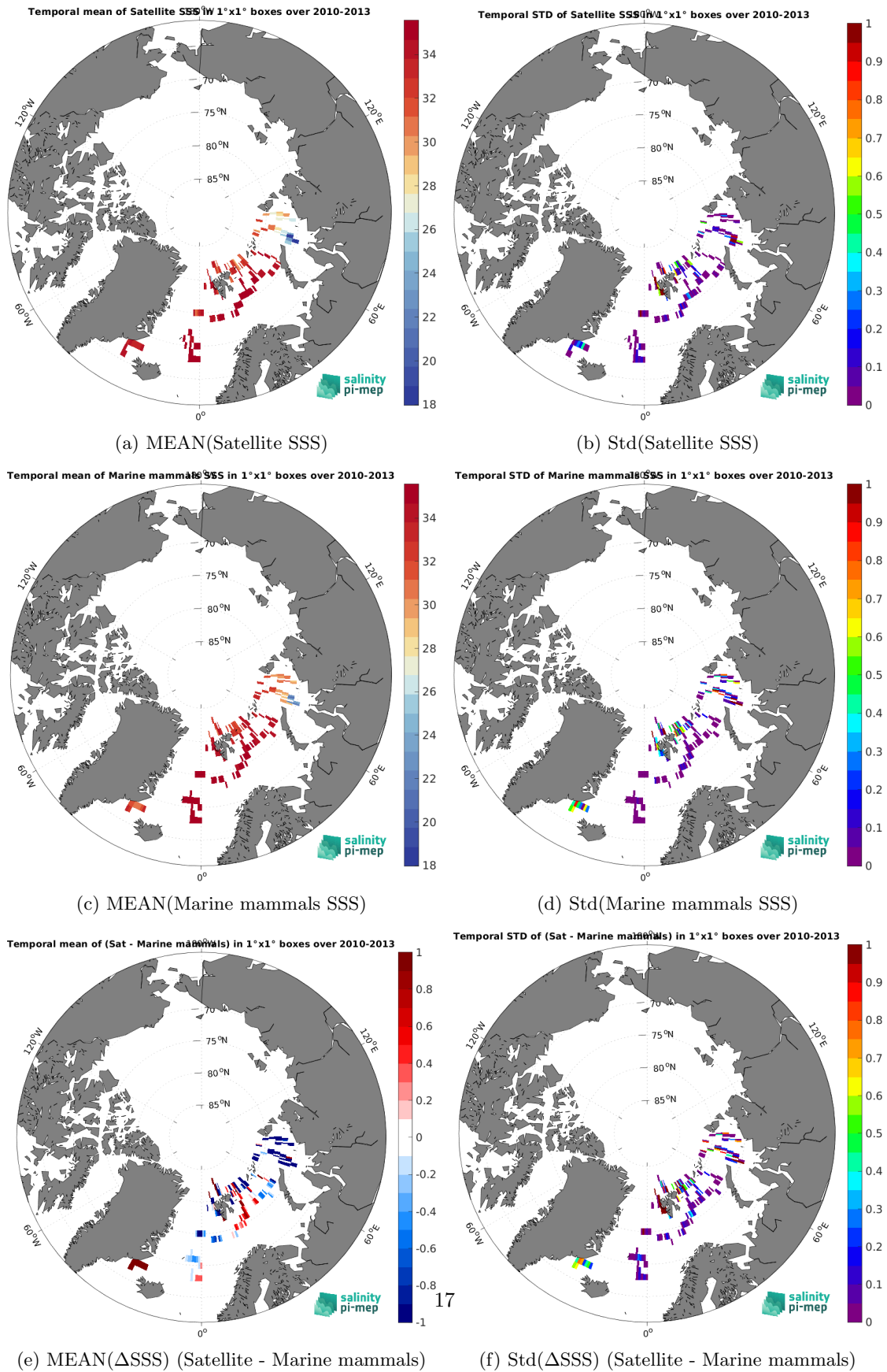
Figure 7: Temporal mean (left) and Std (right) of SSS from SMOS SSS L3 v9 - 9 Days (CATDS-CEC-LOCEAN) (top), Marine mammals (middle), and of \Delta SSS (Satellite - Marine mammals). Only match-up pairs are used to generate these maps.
