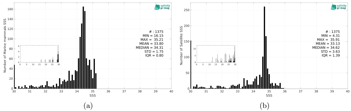
Figure 3: Histograms of SSS from Marine mammals (a) and SMOS SSS L3 v9 - 9 Days (CATDS-CEC-LOCEAN) (b) considering all match-up pairs per bins of 0.1 over the Arctic Ocean Pi-MEP region and for the full satellite product period.
