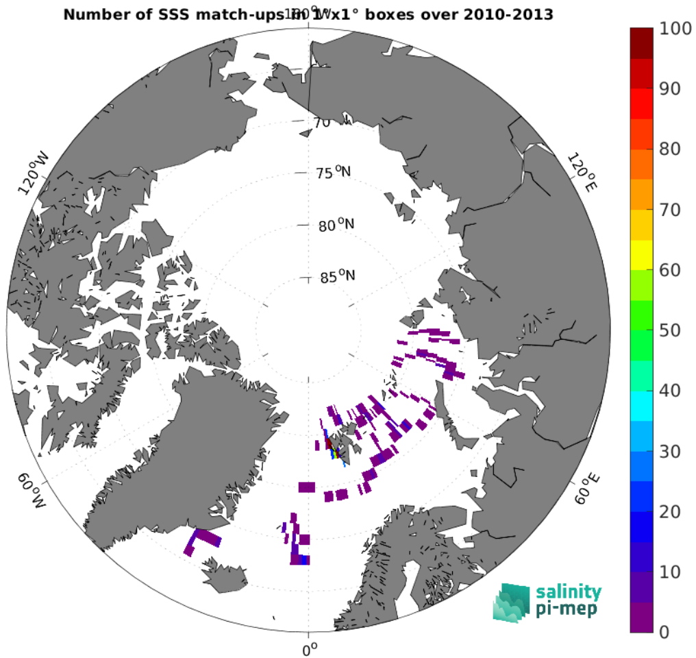
Figure 5: Number of SSS match-ups between Marine mammals SSS and the SMOS SSS L3 v9 - 9 Days (CATDS-CEC-LOCEAN) SSS product for the Arctic Ocean Pi-MEP region over 1^\circ \times 1^\circ boxes and for the full satellite product period.
