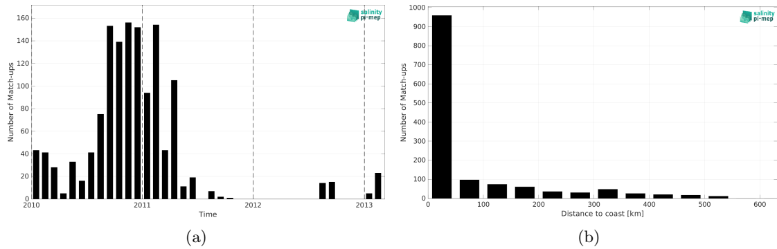
Figure 2: Number of match-ups between Marine mammals and SMOS SSS L3 v9 - 9 Days (CATDS-CEC-LOCEAN) SSS as a function of time (a) and as function of the distance to coast (b) over the Arctic Ocean Pi-MEP region and for the full satellite product period.
