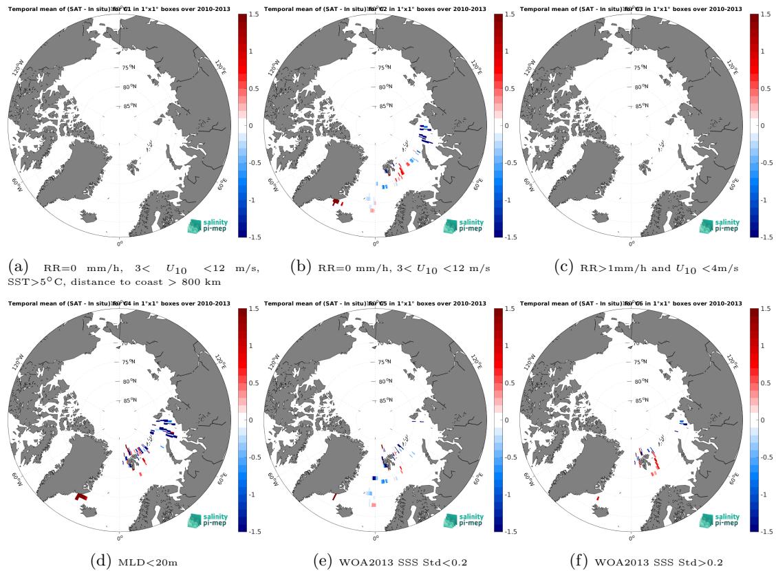
Figure 14: Temporal mean gridded over spatial boxes of size 1^\circ \times 1^\circ of \Delta SSS (SMOS SSS L3 v9 - 9 Days (CATDS-CEC-LOCEAN) - Marine mammals) for 6 different subdatasets corresponding to:RR=0 mm/h, 3 < U_{10} < 12 m/s, SST>5°C, distance to coast > 800 km (a), RR=0 mm/h, 3 < U_{10} < 12 m/s (b), RR>1mm/h and U_{10} < 4 m/s (c),MLD<20m (d),WOA2013 SSS Std<0.2 (e),WOA2013 SSS Std>0.2 (f).
