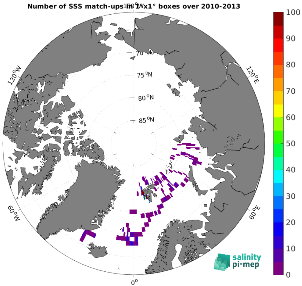
Figure 4: Number of SSS match-ups between Marine mammals SSS and the SMOS SSS L3 v9 - 9 Days (CATDS-CEC-LOCEAN) SSS product for the Arctic Ocean Pi-MEP region over 1^\circ \times 1^\circ boxes and for the full satellite product period.
