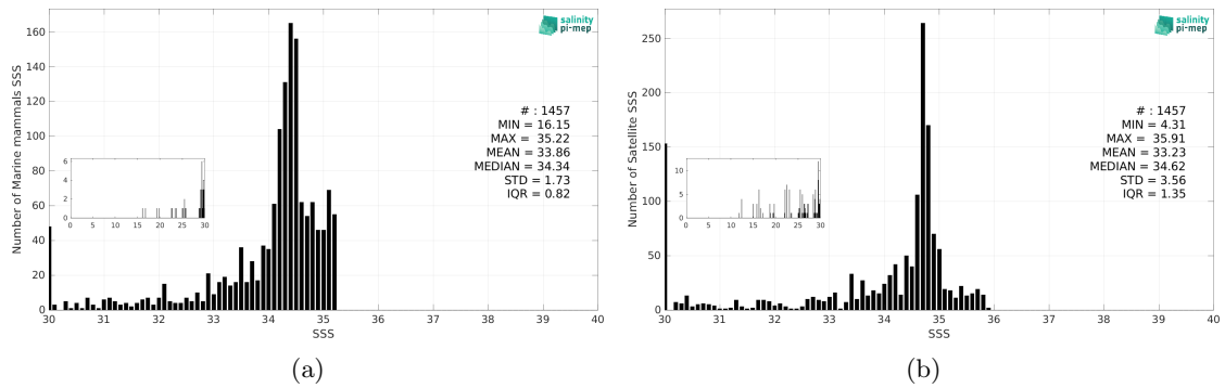
Figure 2: Histograms of SSS from Marine mammals (a) and SMOS SSS L3 v9 - 9 Days (CATDS-CEC-LOCEAN) (b) considering all match-up pairs per bins of 0.1 over the Arctic Ocean Pi-MEP region and for the full satellite product period.
