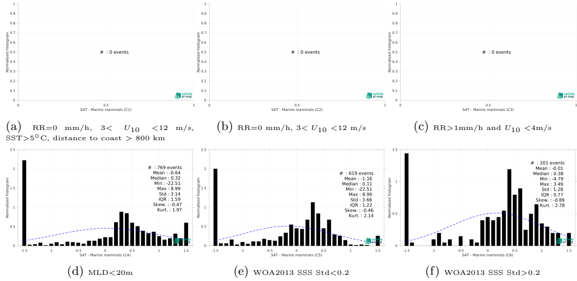
Figure 13: Normalized histogram of \Delta SSS (SMOS SSS L3 v9 - 9 Days (CATDS-CEC-LOCEAN) - Marine mammals) for 6 different subdatasets corresponding to: RR=0 mm/h, 3 < U_{10} < 12 m/s, SST > 5°C, distance to coast > 800 km (a), RR=0 mm/h, 3 < U_{10} < 12 m/s (b), RR > 1mm/h and U_{10} < 4 m/s (c), MLD < 20m (d), WOA2013 SSS Std < 0.2 (e), WOA2013 SSS Std > 0.2 (f).
