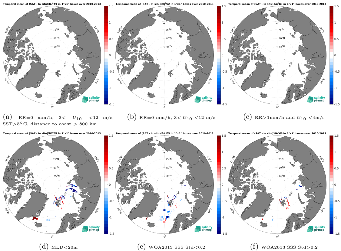
Figure 12: Temporal mean gridded over spatial boxes of size 1^{\circ}\times 1^{\circ} of \Delta\text{SSS} (SMOS SSS L3 v9 - 9 Days (CATDS-CEC-LOCEAN) - Marine mammals) for 6 different subdatasets corresponding to: RR=0 mm/h, 3 < U_{10} < 12 m/s, SST > 5^{\circ}\text{C} , distance to coast > 800 km (a), RR=0 mm/h, 3 < U_{10} < 12 m/s (b), RR > 1\text{mm/h} and U_{10} < 4\text{m/s} (c), MLD < 20\text{m} (d), WOA2013 SSS Std < 0.2 (e), WOA2013 SSS Std > 0.2 (f).
