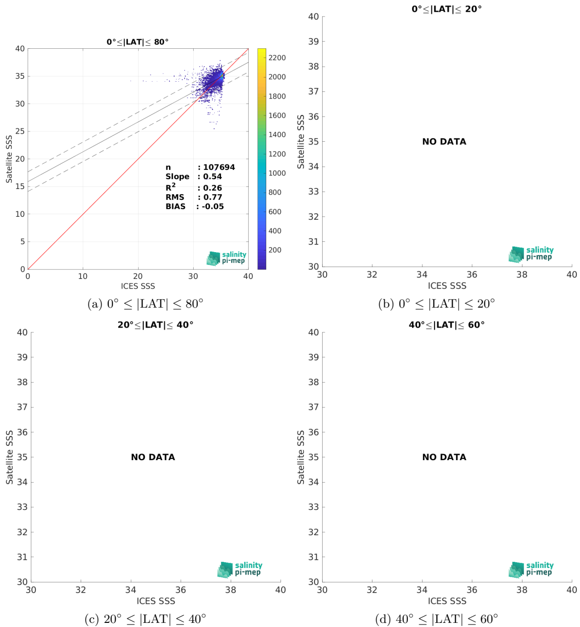
Figure 10: Contour maps of the concentration of SMOS SSS L3 v9 - 9 Days (CATDS-CEC-LOCEAN) SSS (y-axis) versus ICES SSS (x-axis) at match-up pairs for different latitude bands. For each plot, the red line shows x=y . The black thin and dashed lines indicate a linear fit through the data cloud and the \pm 95\% confidence levels, respectively. The number match-up pairs n , the slope and R^2 coefficient of the linear fit, the root mean square (RMS) and the mean bias between satellite and in situ data are indicated for each latitude band in each plots.
