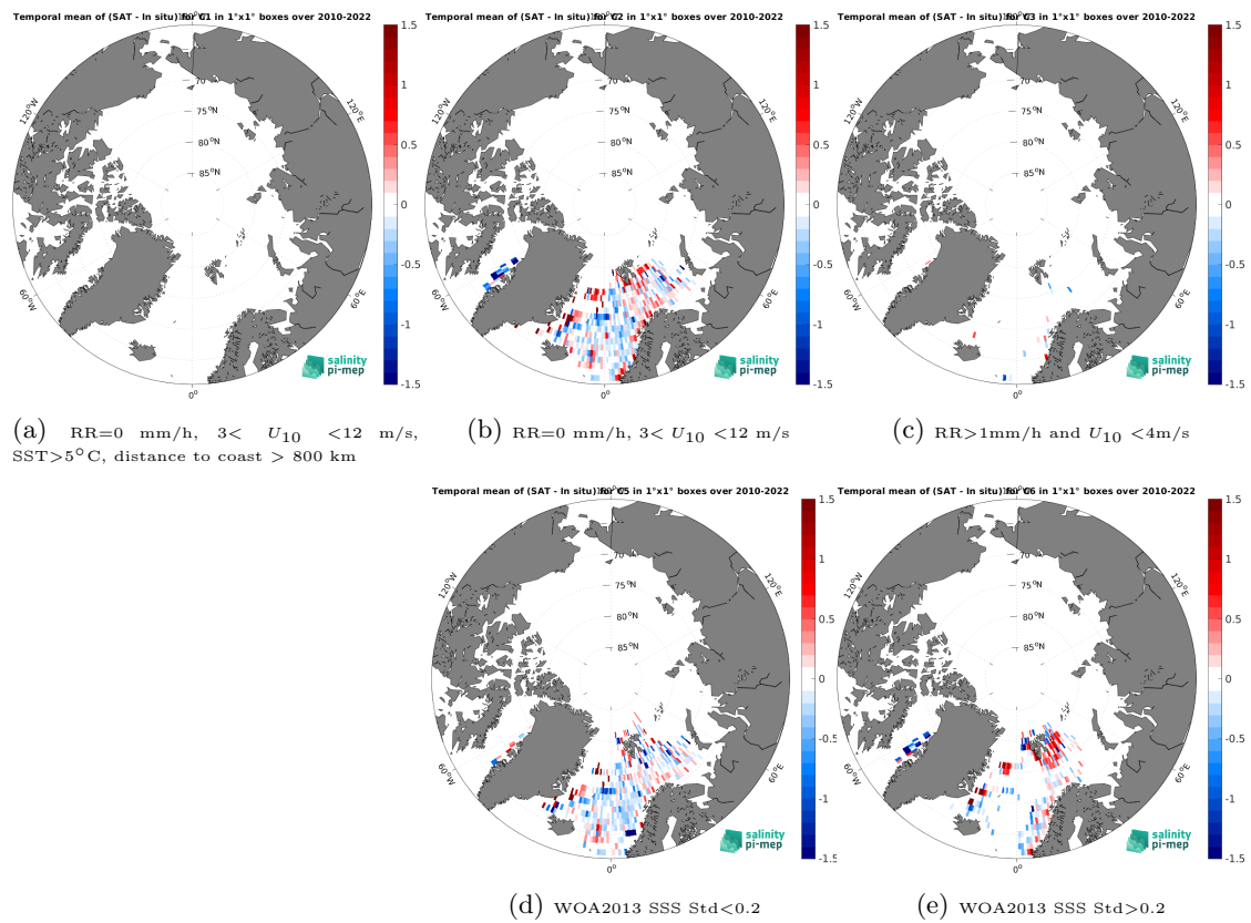
Figure 14: Temporal mean gridded over spatial boxes of size 1^\circ \times 1^\circ of \Delta SSS (SMOS SSS L3 v9 - 9 Days (CATDS-CEC-LOCEAN) - ICES) for 5 different subdatasets corresponding to:RR=0 mm/h, 3 < U_{10} < 12 m/s, SST > 5°C, distance to coast > 800 km (a), RR=0 mm/h, 3 < U_{10} < 12 m/s (b), RR > 1mm/h and U_{10} < 4 m/s (c), WOA2013 SSS Std < 0.2 (d), WOA2013 SSS Std > 0.2 (e).
