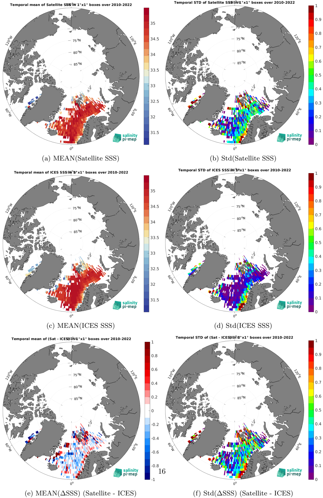
Figure 7: Temporal mean (left) and Std (right) of SSS from SMOS SSS L3 v9 - 9 Days (CATDS-CEC-LOCEAN) (top), ICES (middle), and of \Delta SSS (Satellite - ICES). Only match-up pairs are used to generate these maps.
