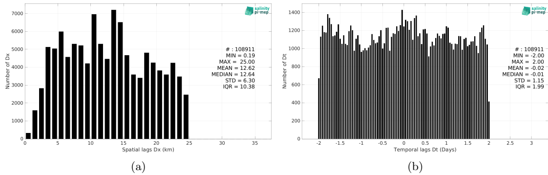
Figure 6: Histograms of the spatial (a) and temporal (b) lags between the location/time of the ICES measurement and the date of the corresponding SMOS SSS L3 v9 - 9 Days (CATDS-CEC-LOCEAN) SSS pixel.
